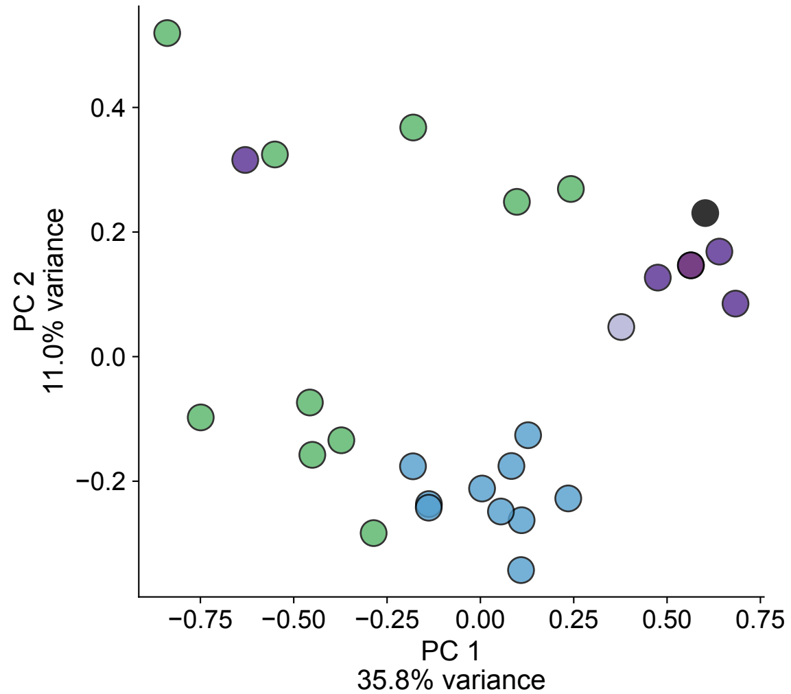
PCA on Correlation of BC Counts CBE EPO screen
