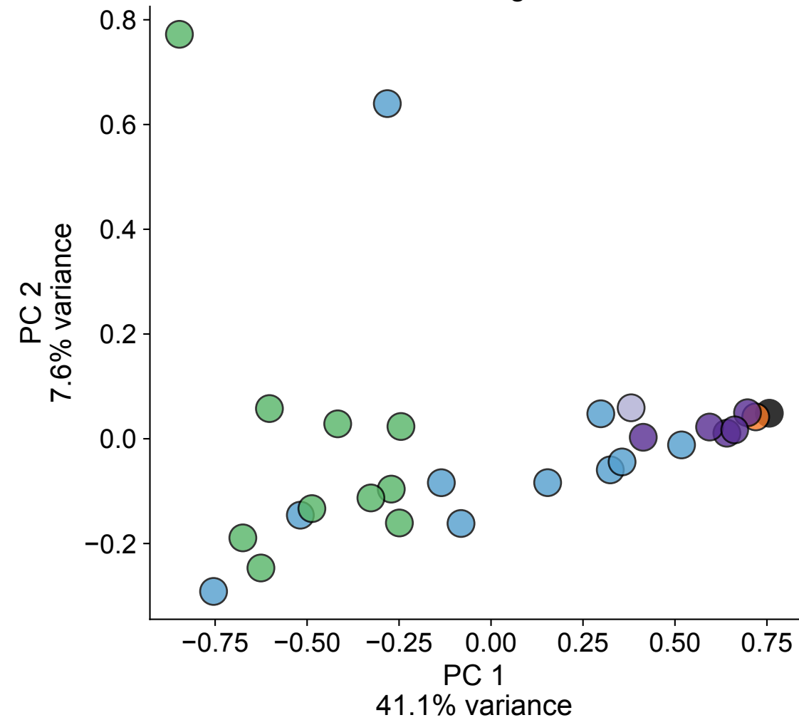
PCA on Correlation of BC Counts CBE barcoding screen
