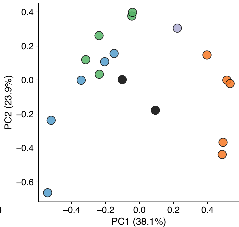
ABE Focused v2 EPO
