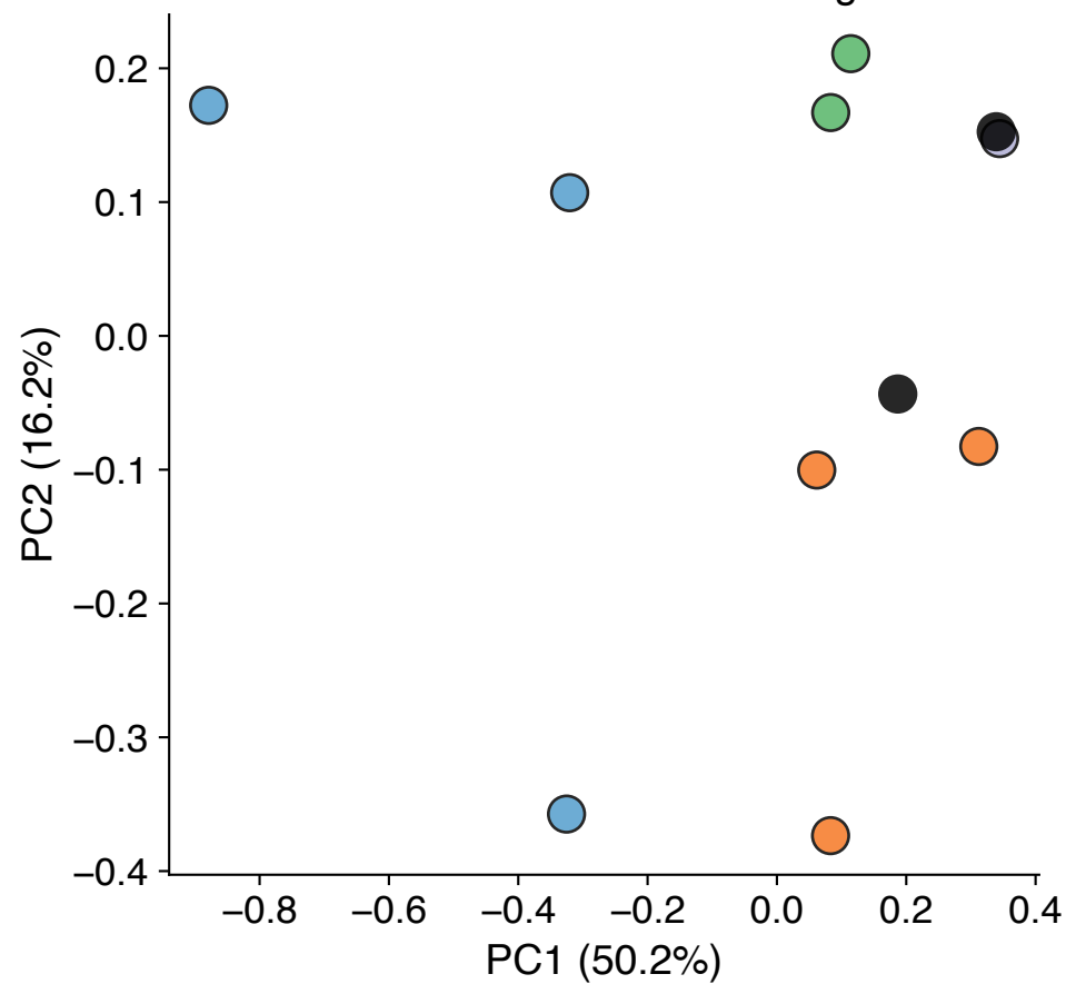
ABE Focused v2 Barcoding
