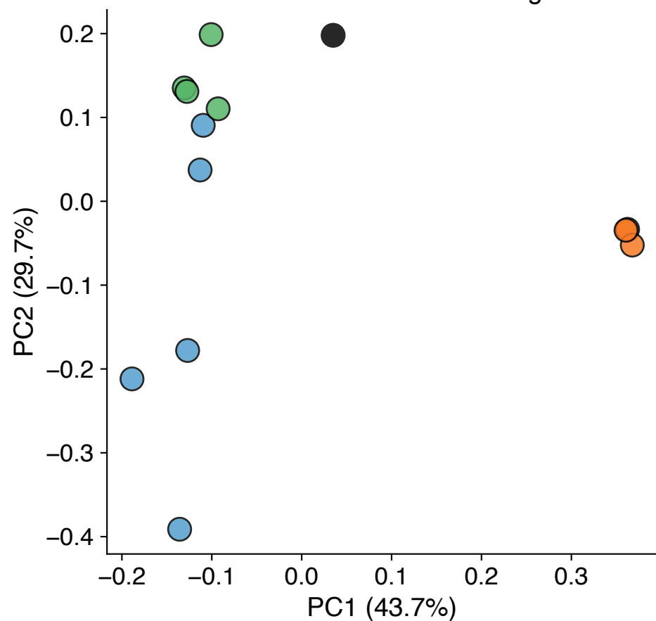
ABE Focused v2 Barcoding
