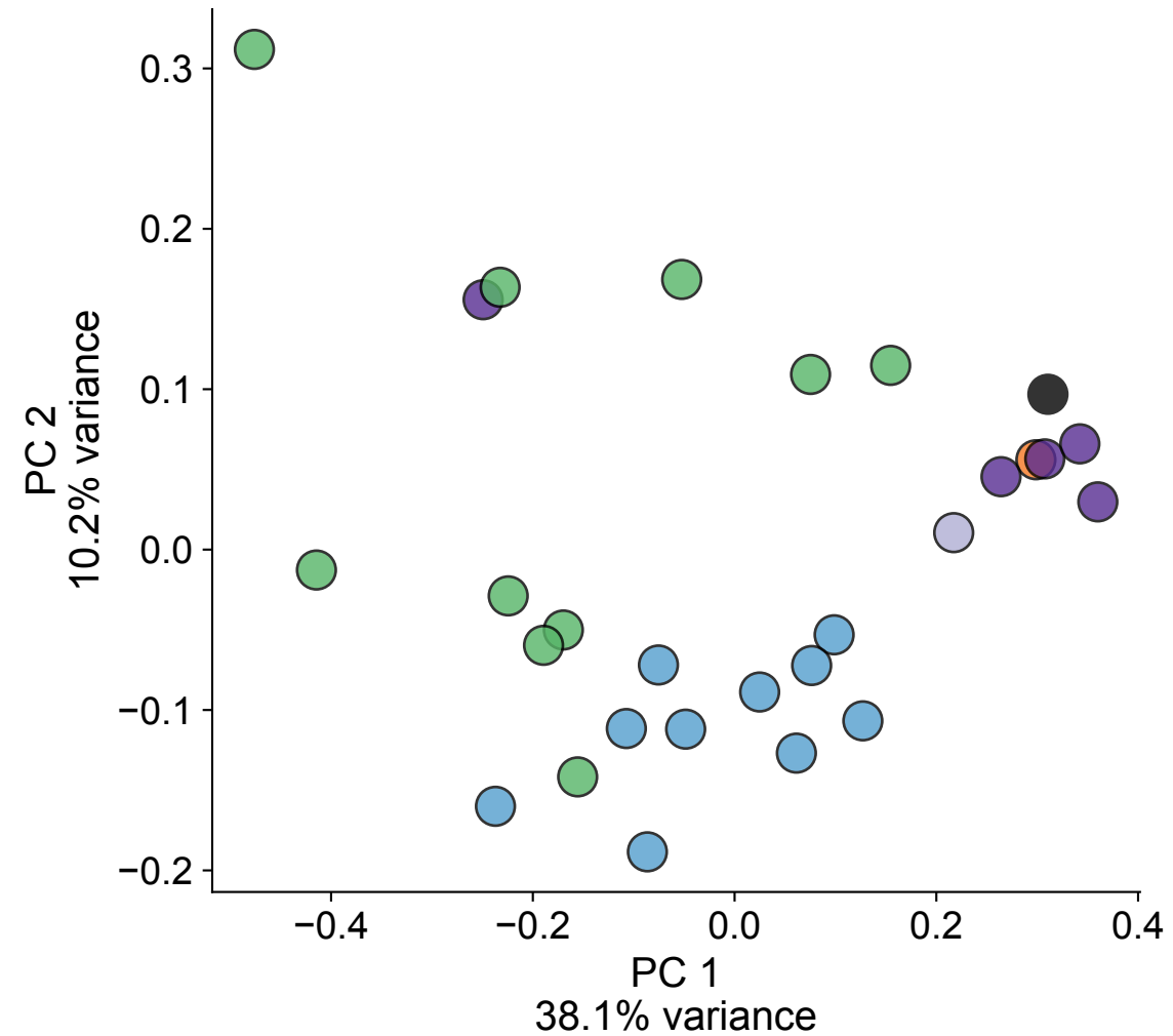
PCA on Correlation of BC Counts CBE EPO screen
