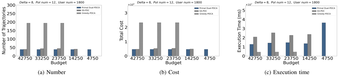
Fig. 2: Performance of the three algorithms under five different budget for meeting data collection requirements.
