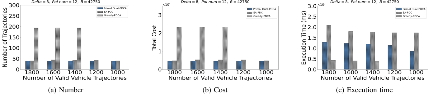
Fig. 3: Performance of the three algorithms under five different number of vehicles for meeting data collection requirements.
