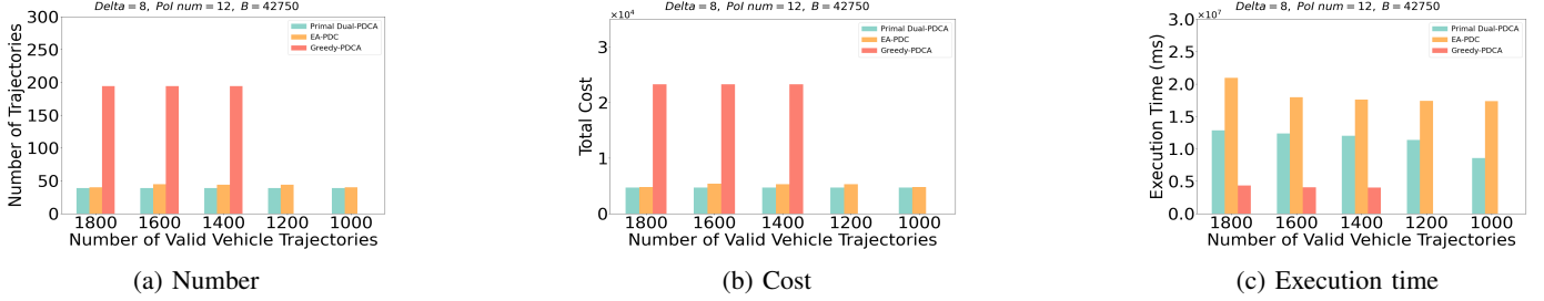
Fig. 2: Performance of the three algorithms under five different number of vehicles for meeting data collection requirements.
