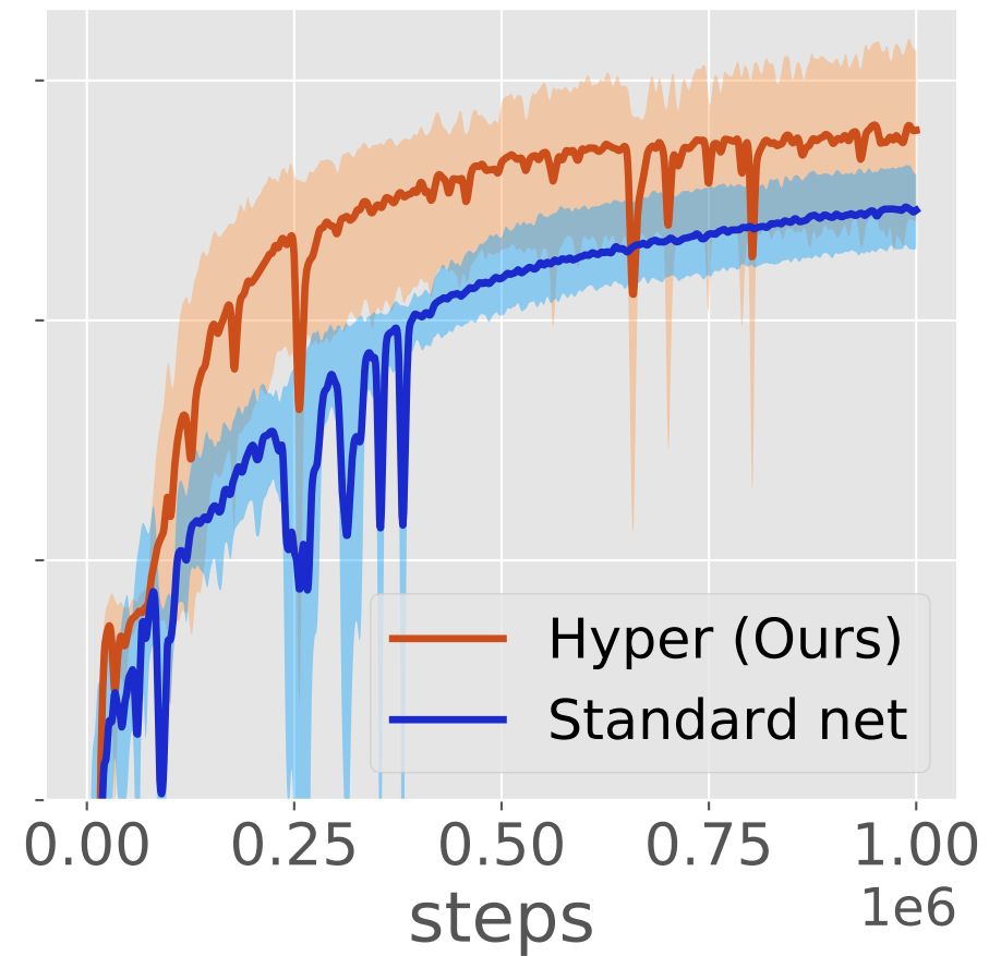
HalfCheetah
