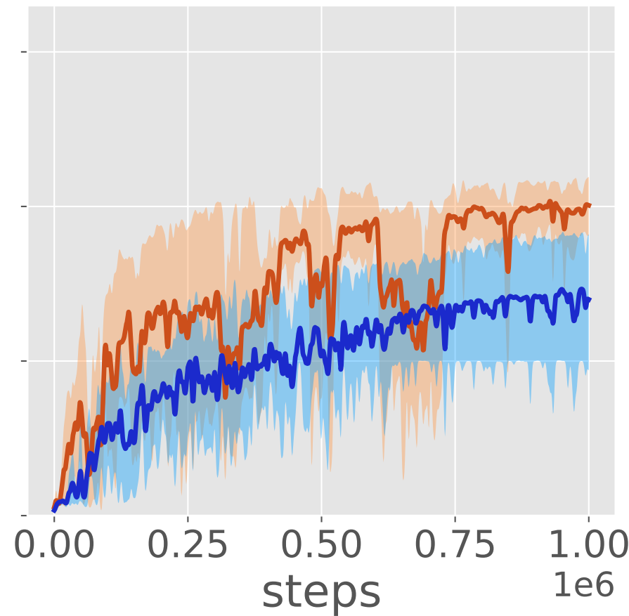
Walker2D
