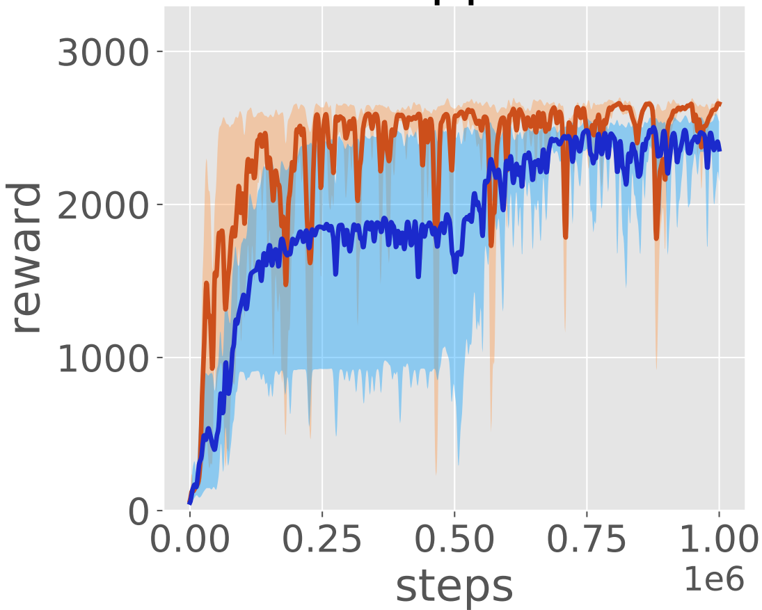
Hopper
