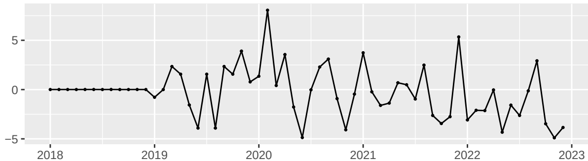
Residuals from ARIMA(0,0,0)(0,1,1)[12]
