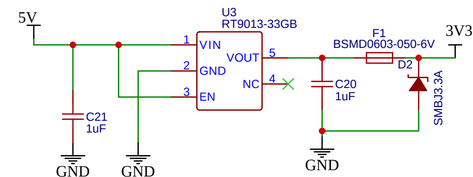
5V TO 3V3
