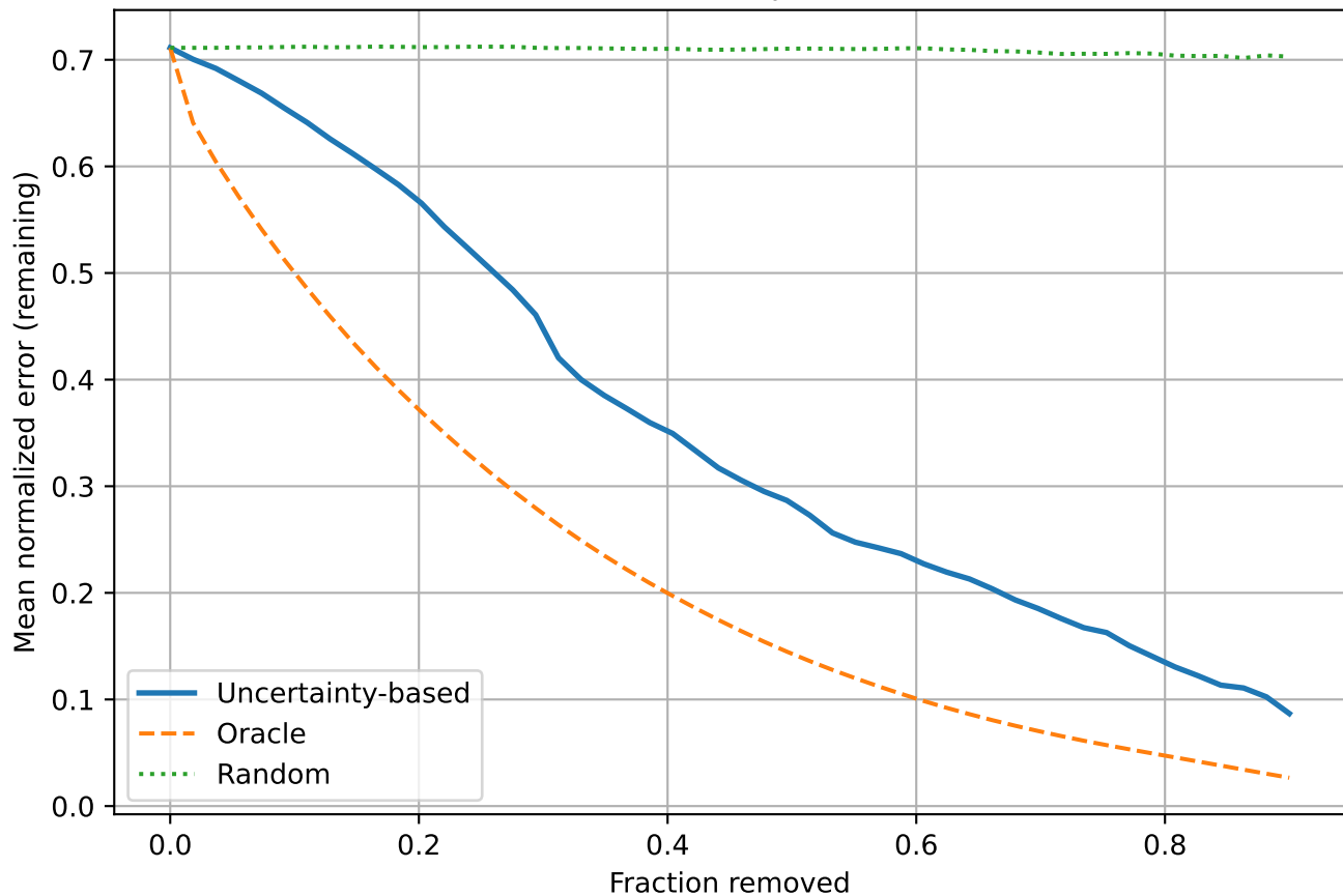
BPIC20ID: Normalized Sparsification Curve
