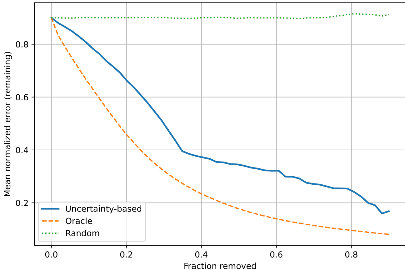
BPIC20PTC: Normalized Sparsification Curve
