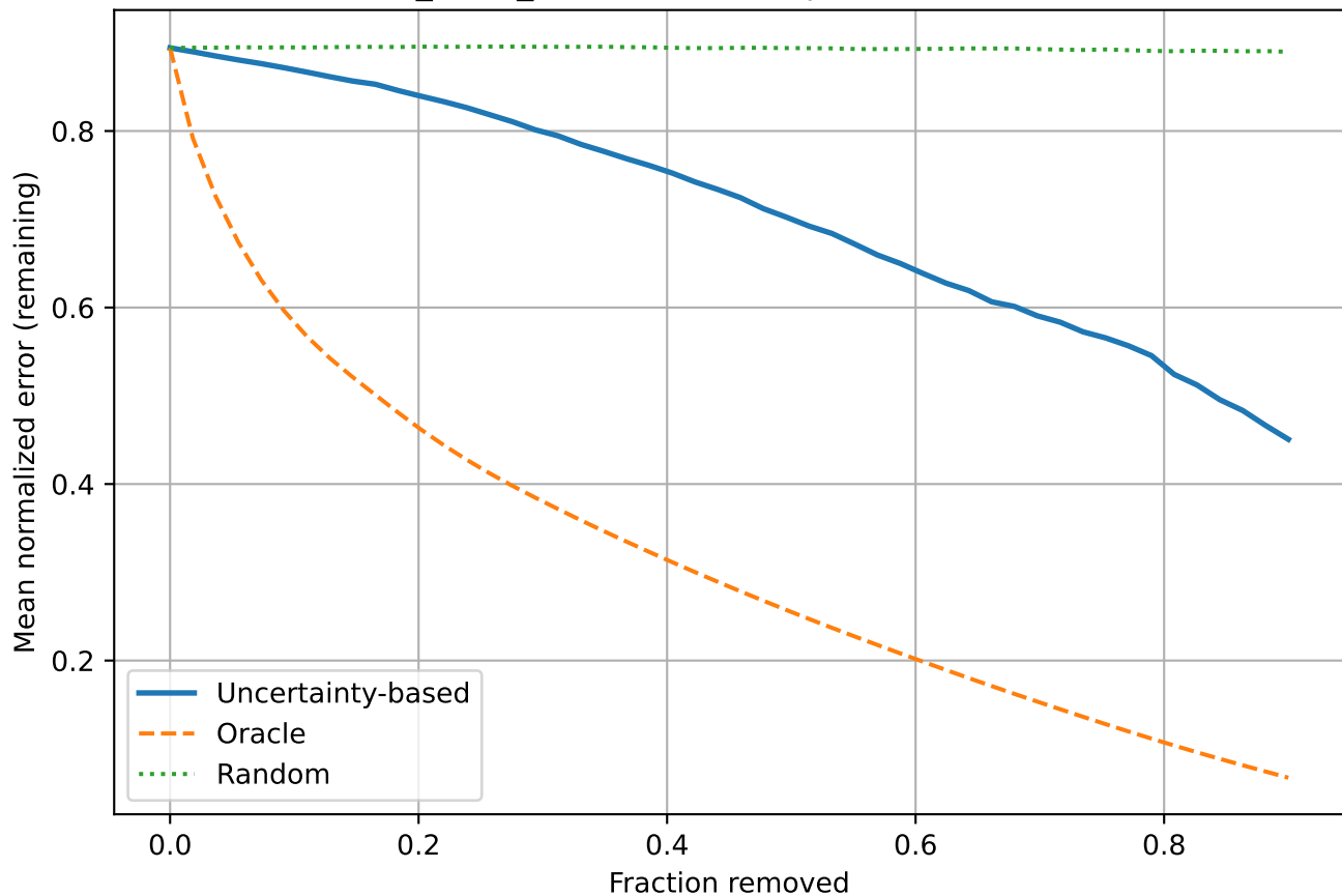
BPIC_2017_W: Normalized Sparsification Curve
