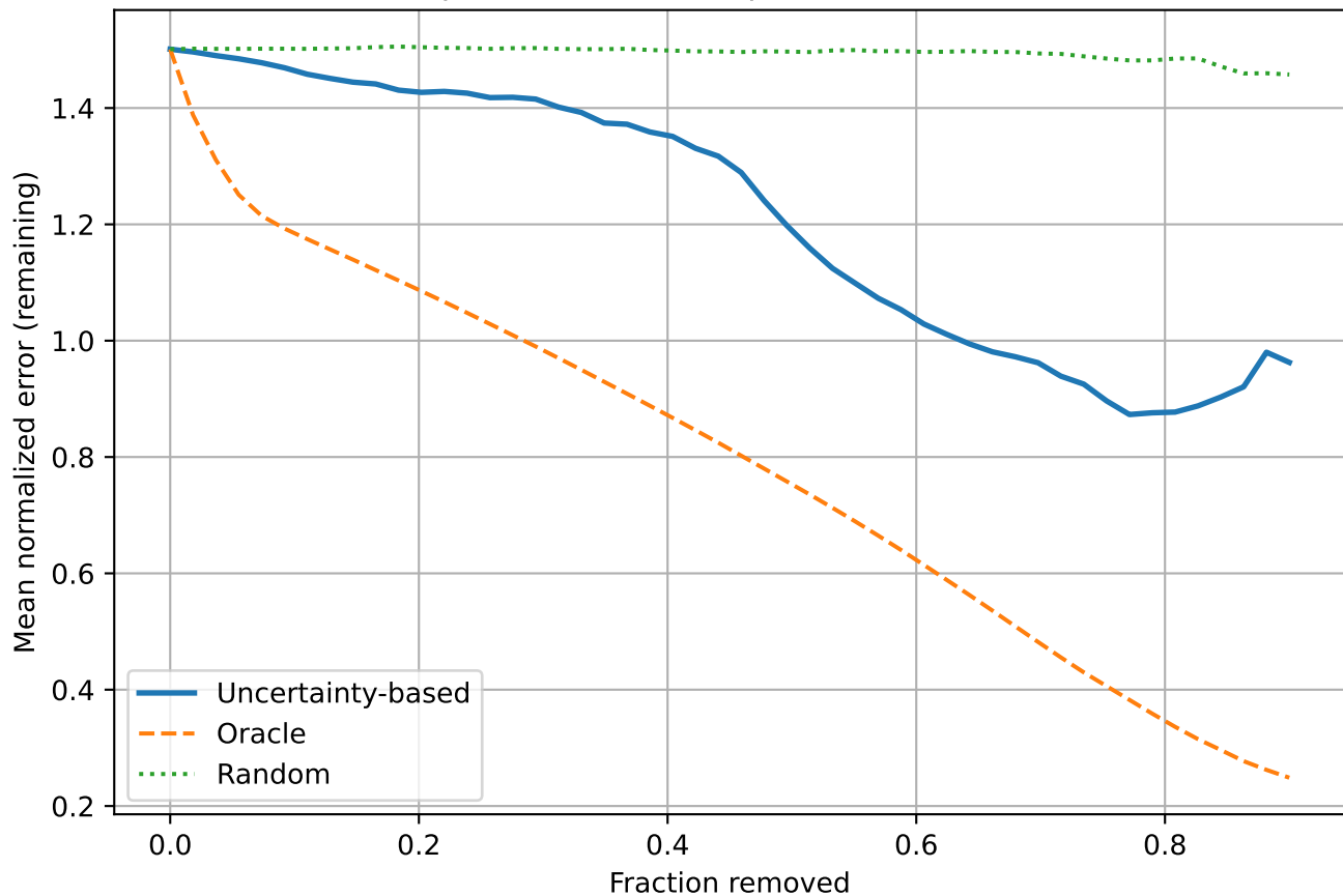
Sepsis: Normalized Sparsification Curve
