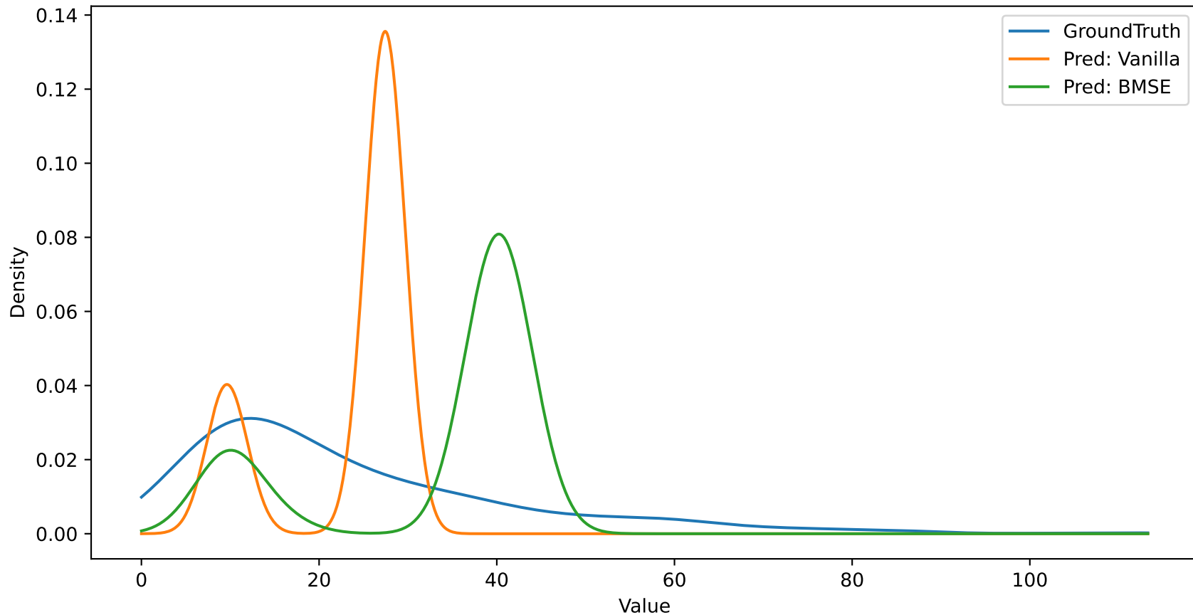
GroundTruth vs Predictions distribution (BPIC20PTC / DALSTM)
