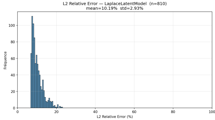
Figure 4: Relative L^2 error on the test set after end-to-end fine-tuning.
