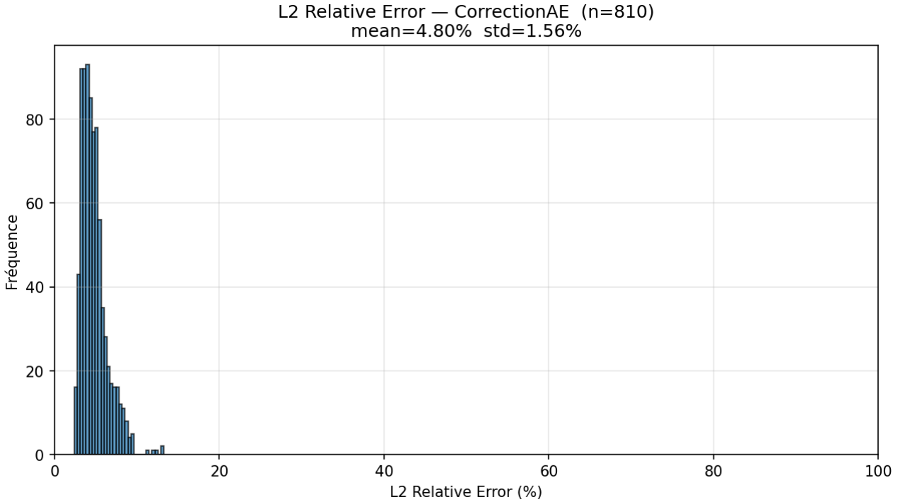
Figure 5: Relative L^2 error distribution after residual correction.
