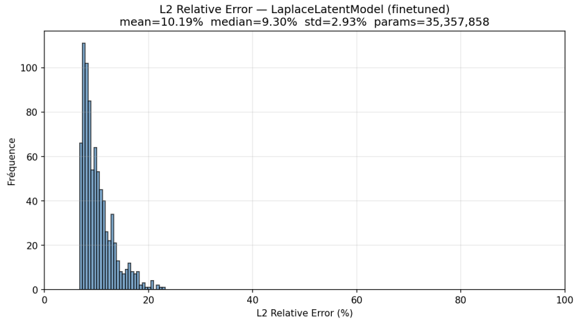
Figure 6: Relative L^2 error distribution after end-to-end fine-tuning (mean: 10.19%, median: 9.30%). Fine-tuning reduces error by approximately 48% compared to the frozen baseline.
