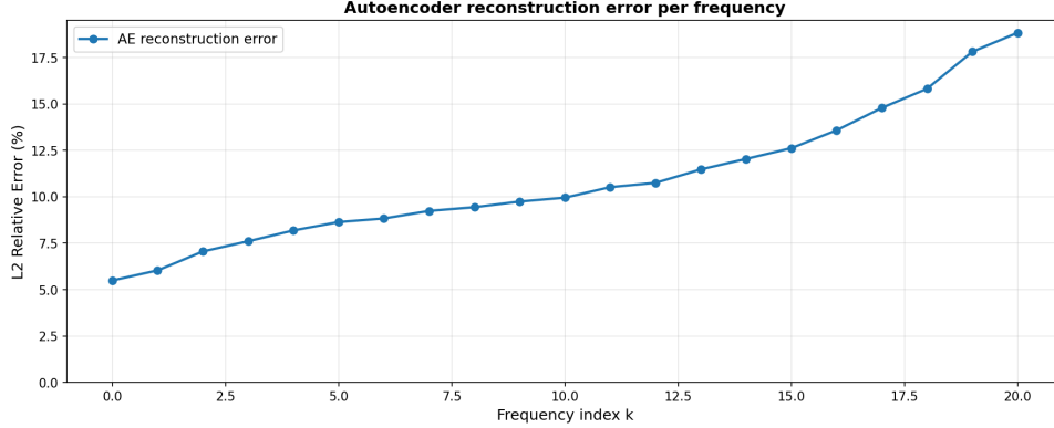
Figure 4: Autoencoder L2 relative reconstruction error per frequency, evaluated on 64 test samples. The AE exhibits increasing error at higher frequencies, reflecting the difficulty of capturing high-frequency oscillations in the latent code.
