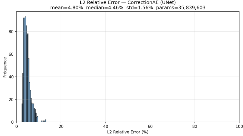
Figure 7: Relative L^2 error distribution after residual UNet correction (mean: 4.80%, median: 4.46%). The correction reduces error by approximately 76% compared to the baseline latent surrogate.
