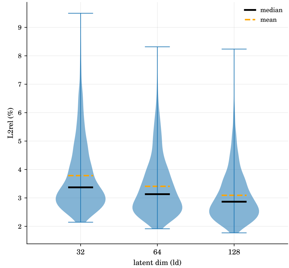
LLAE: effect of latent dim (K=16, \gamma=0.01 )
