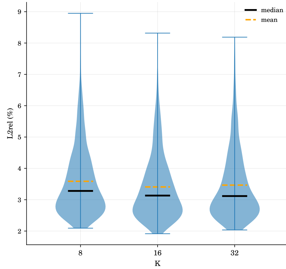
LLAE: effect of K (ld=64, \gamma=0.01 )
