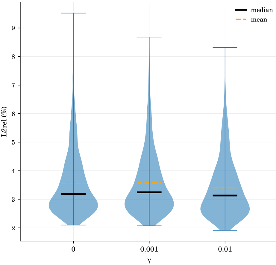
LLAE: effect of \gamma (ld=64, K=16)
