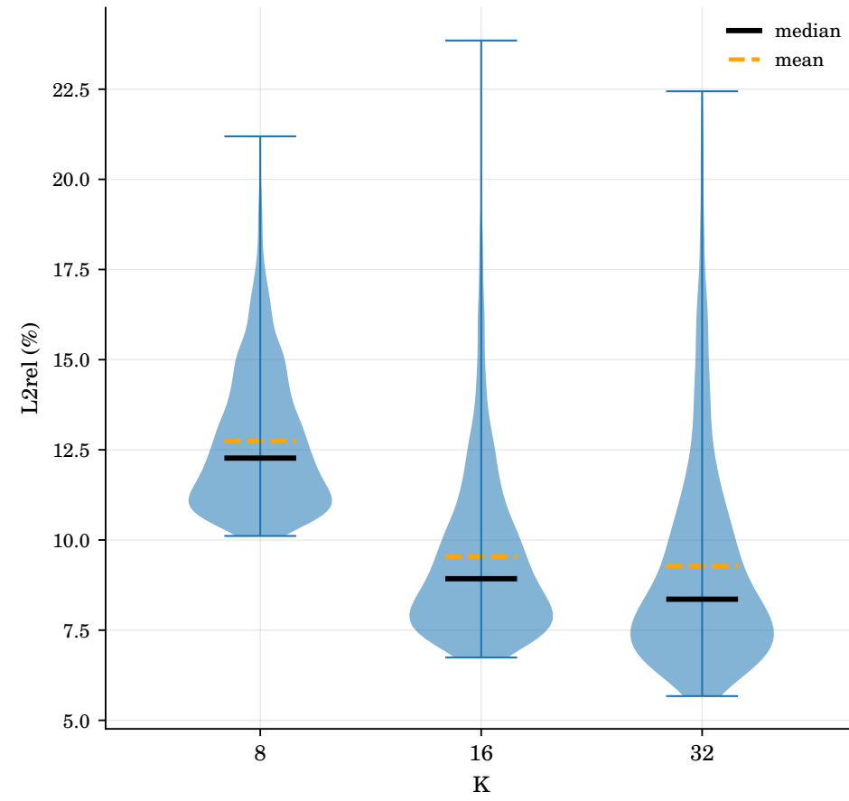
SLAE: effect of K (ld=64, \gamma=0.01 )
