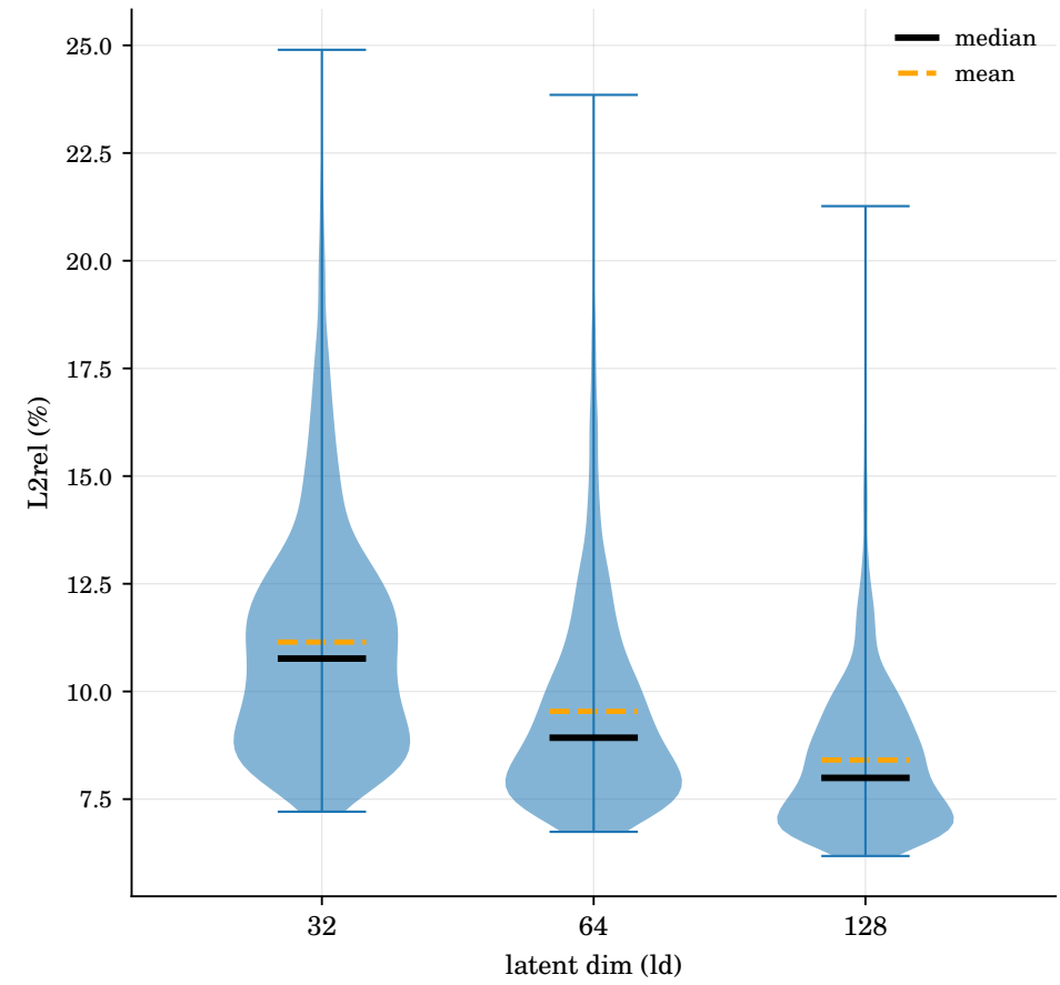
SLAE: effect of latent dim (K=16, \gamma=0.01 )
