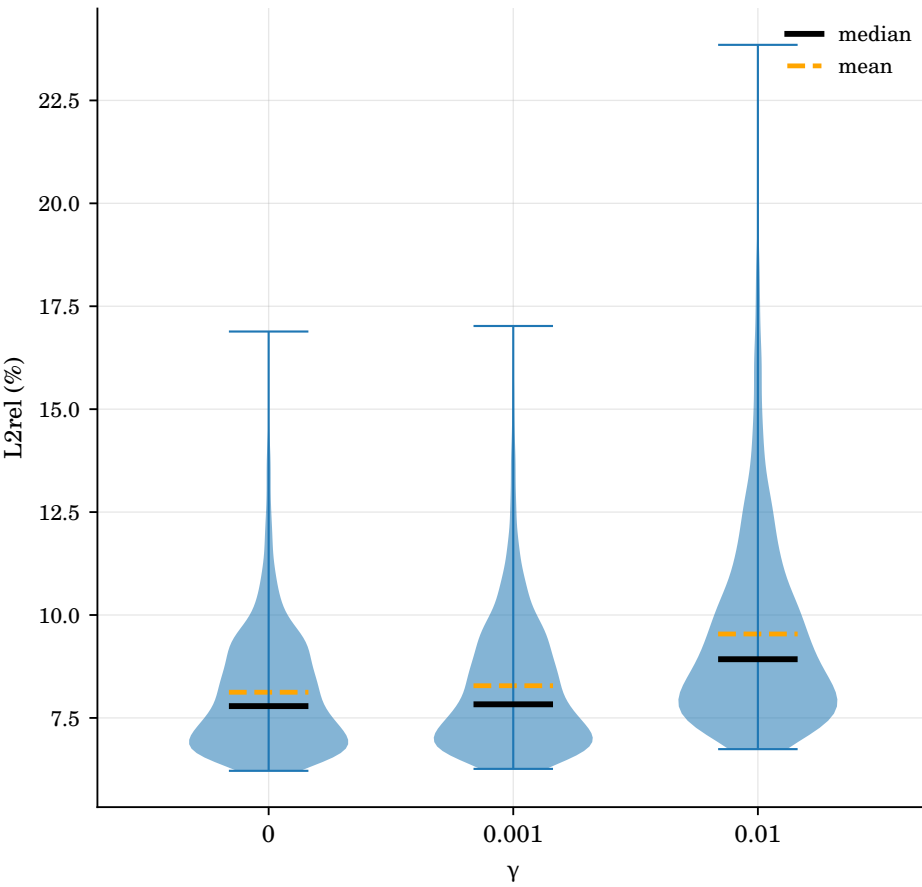
SLAE: effect of \gamma (ld=64, K=16)
