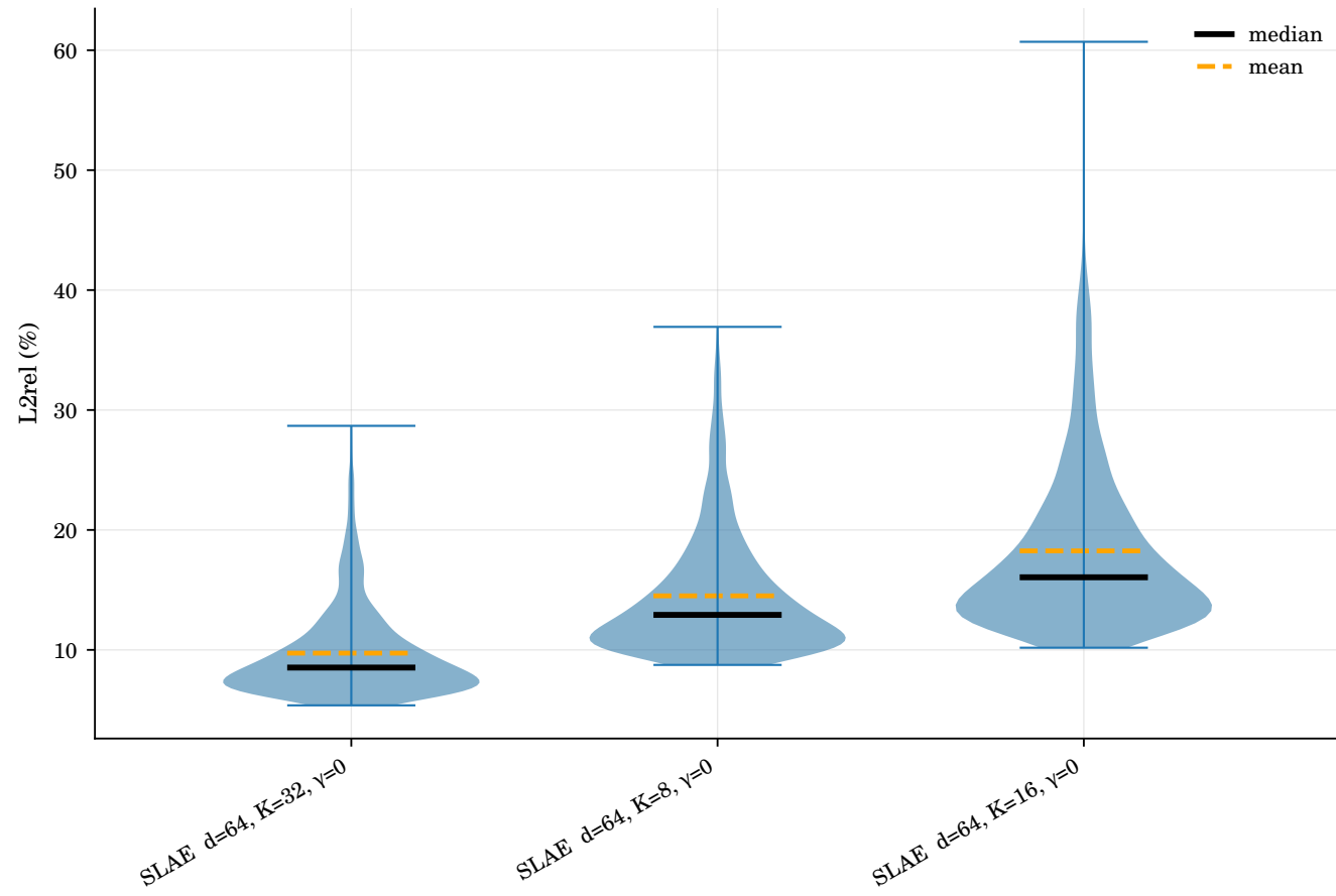
SLAE — L2rel distribution per checkpoint
