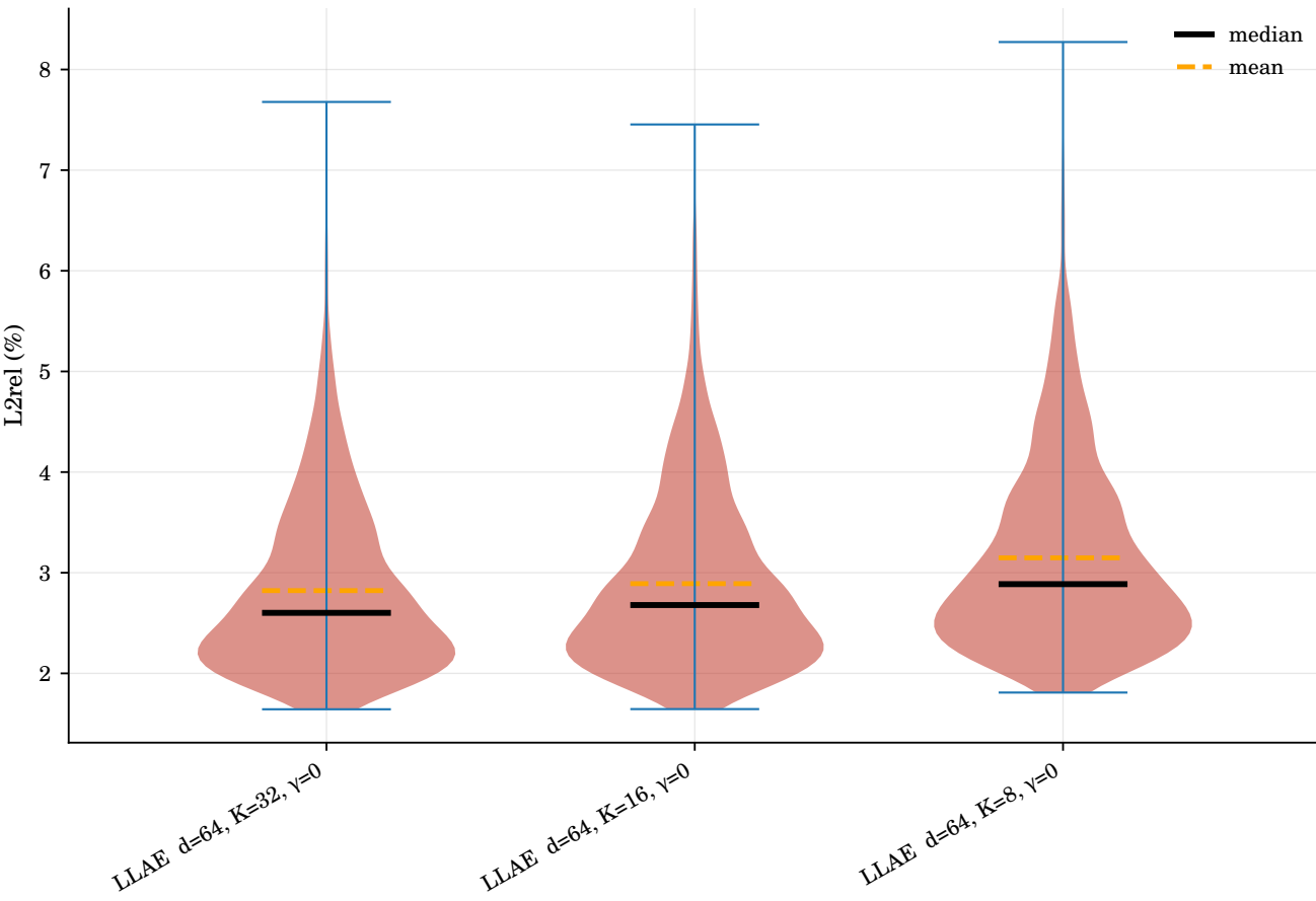
LLAE — L2rel distribution per checkpoint
