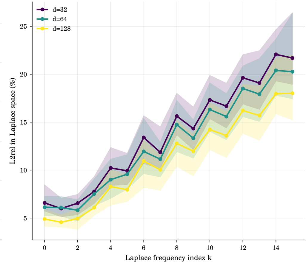
Effect of latent dim (K=16, \gamma=0.01 )
