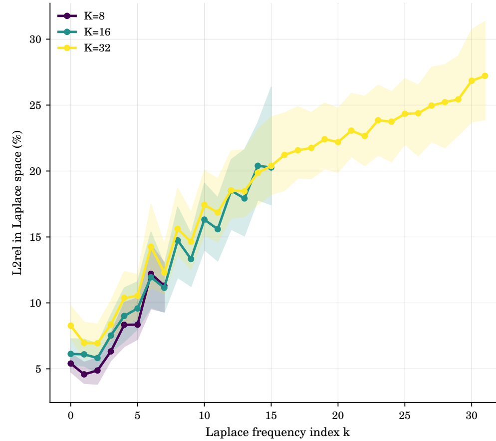
Effect of K (d=64, \gamma=0.01 )
