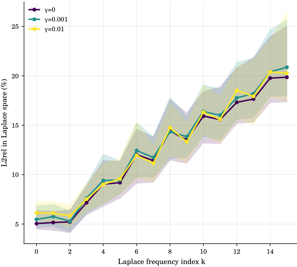
Effect of \gamma (d=64, K=16)
