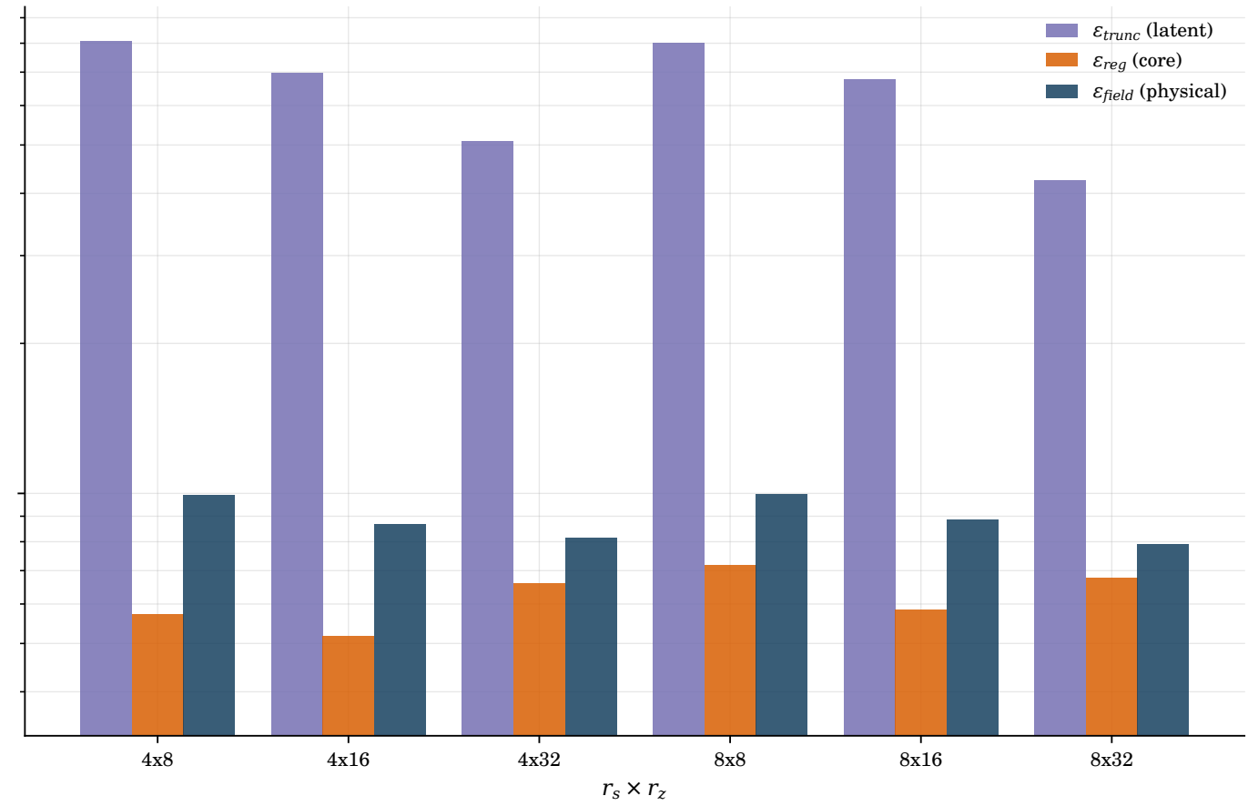
SLAE-Tucker
