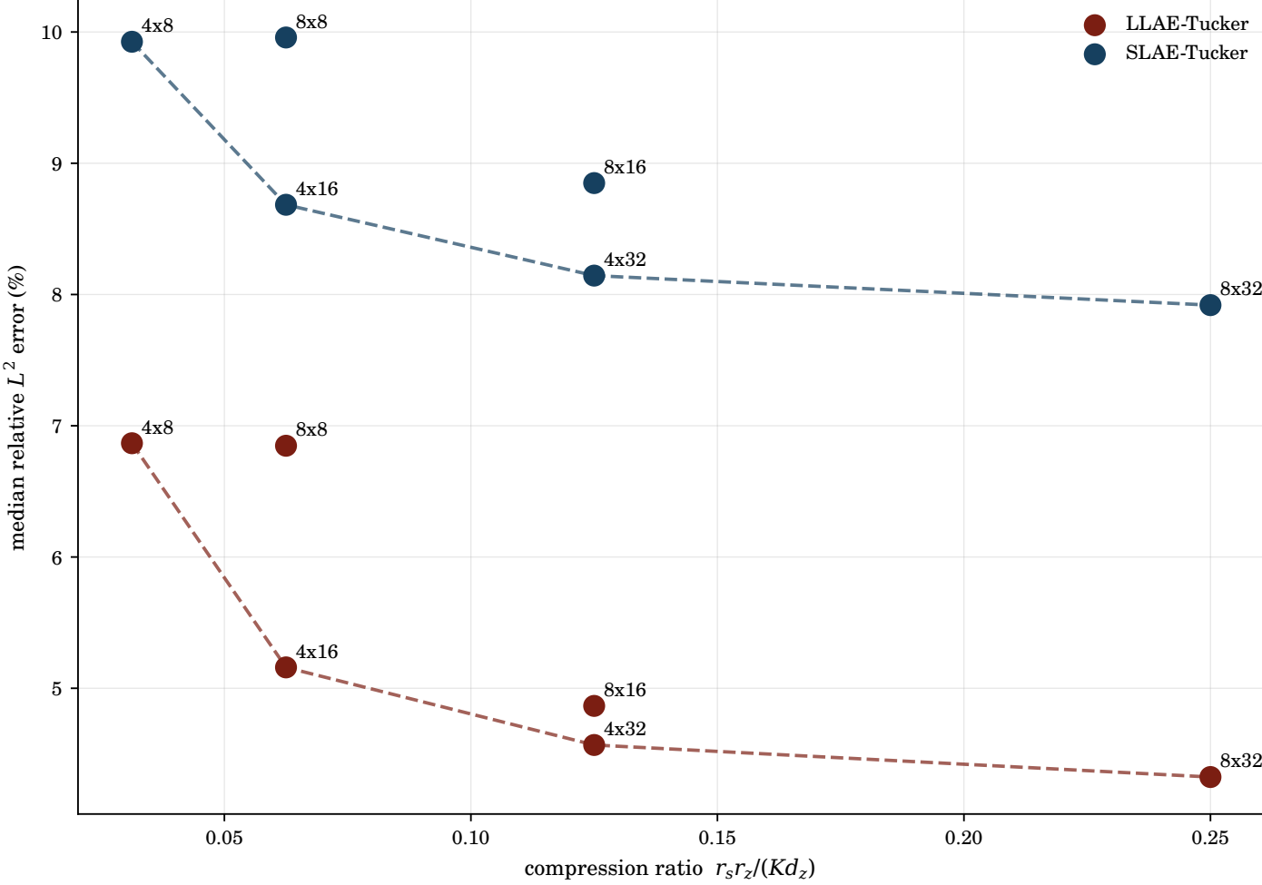
Error vs compression (dashed: Pareto front)
