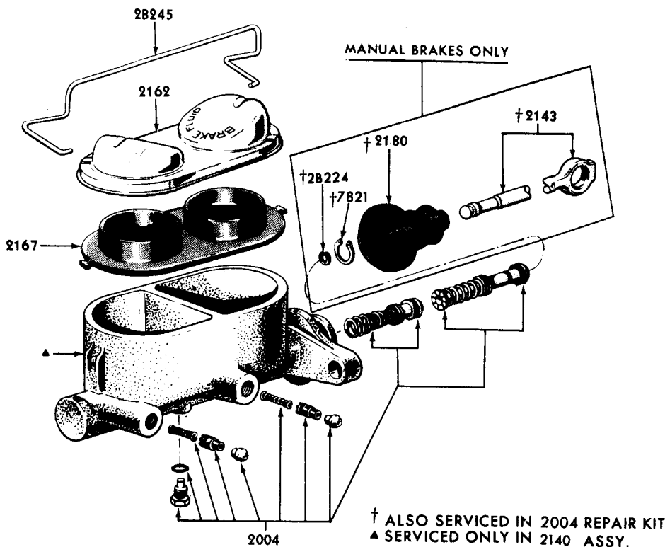
BRAKE MASTER CYLINDER - TYPICAL 1967/72 BRONCO, FORD, FAIRLANE/TORINO, FALCON, PINTO, MAVERICK, MUSTANG, THUNDERBIRD
