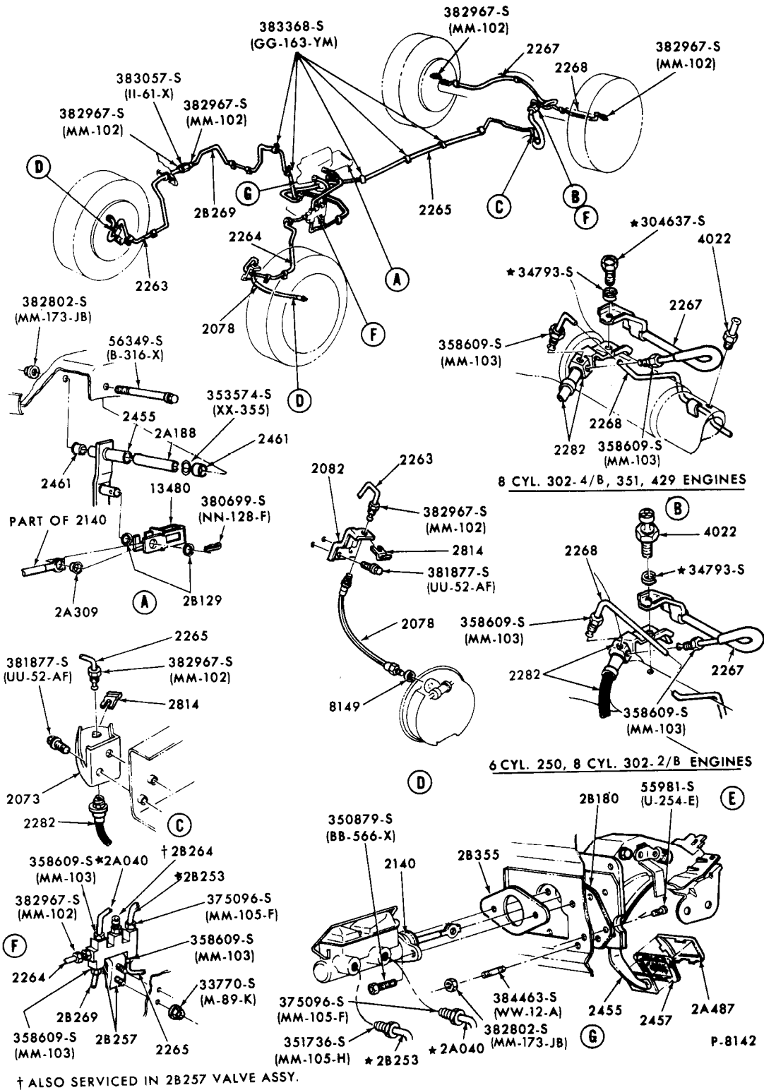
DRUM BRAKE SYSTEM 1971/72 MUSTANG
