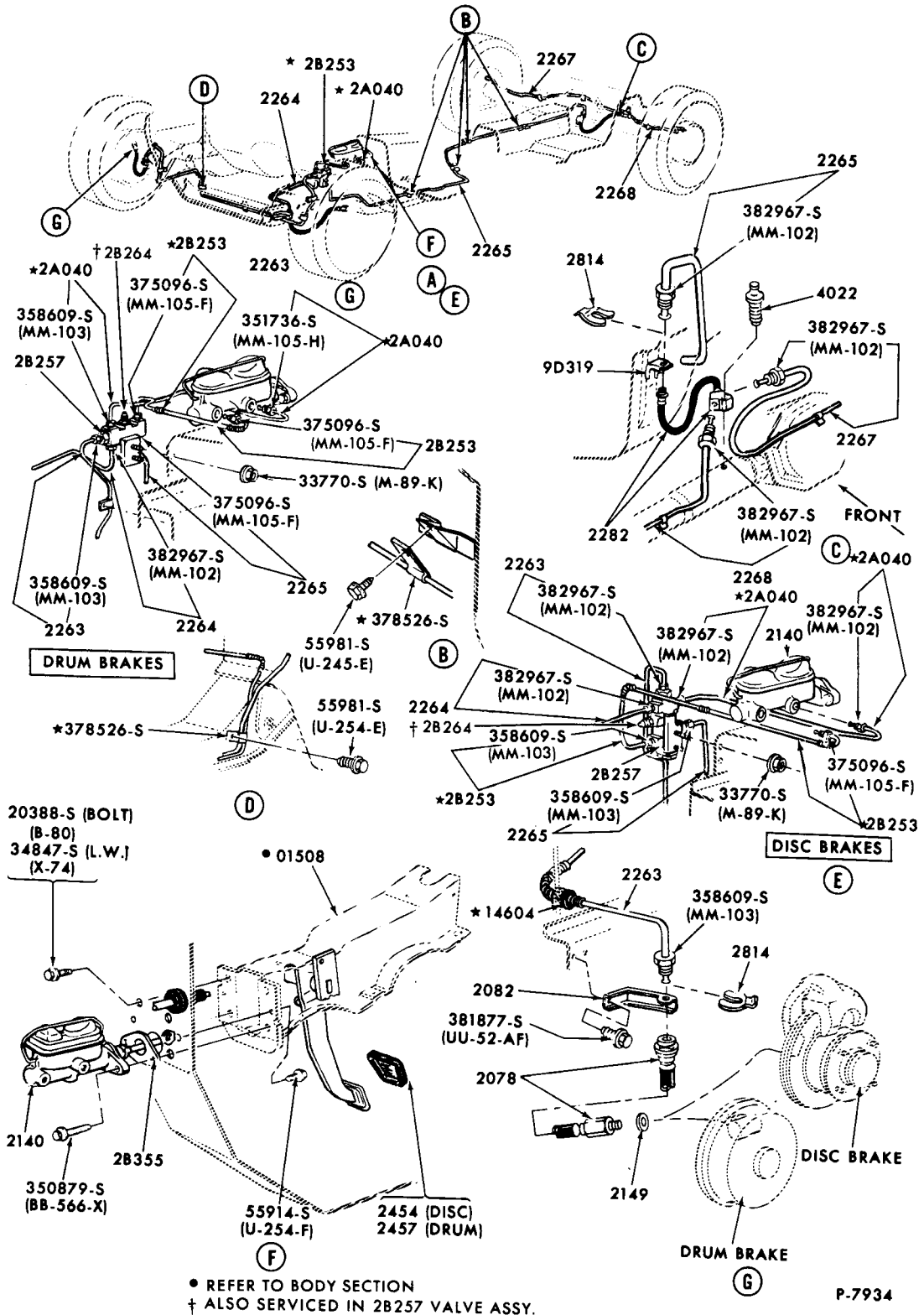
DISC and DRUM BRAKE SYSTEM 1971/72 PINTO
