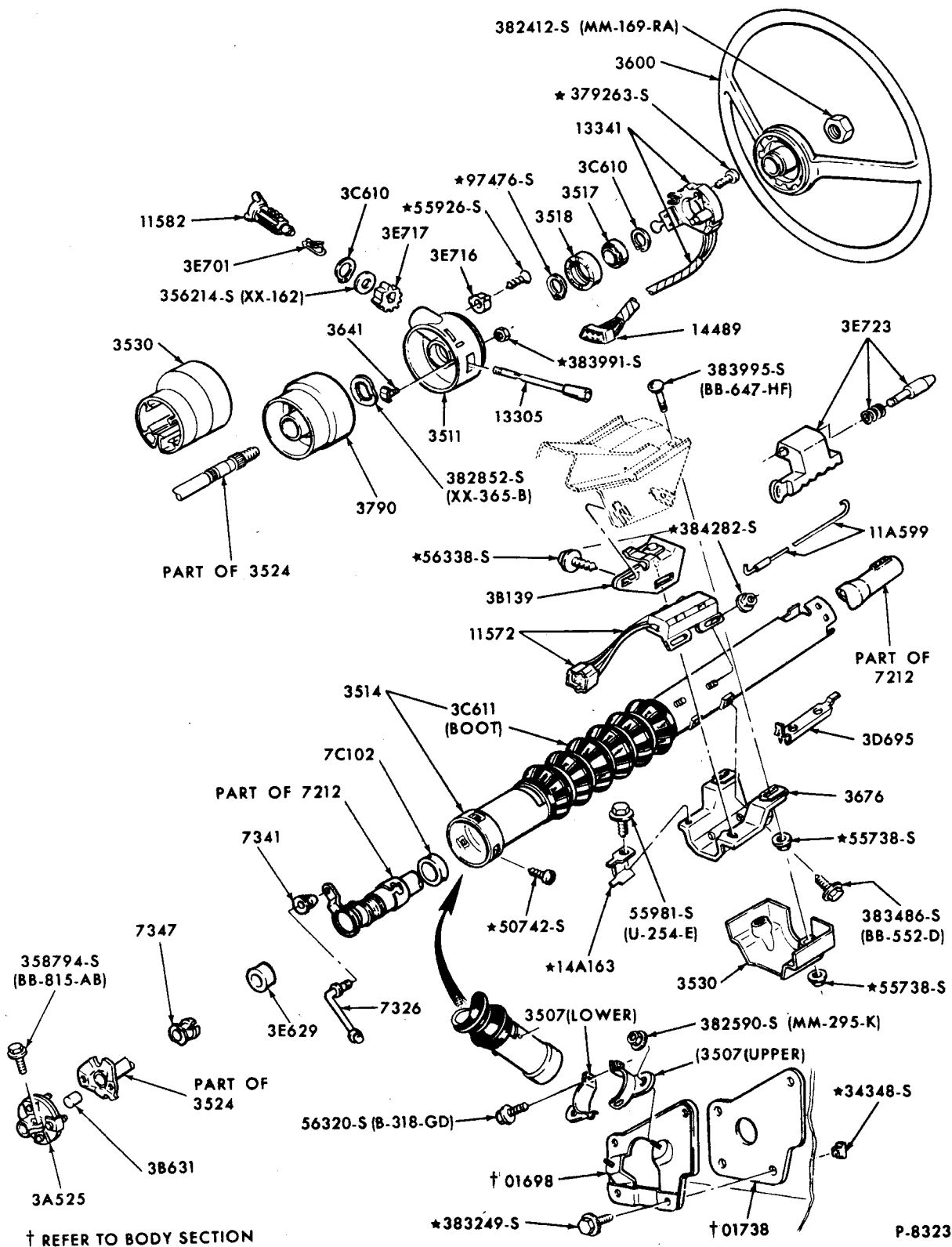
STEERING COLUMN FOR FLOOR SHIFT 1971/72 MAVERICK
