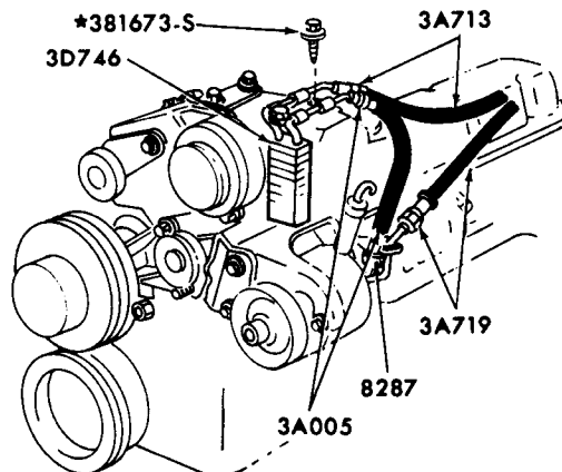
POWER STEERING WITH AIR CONDITIONING
