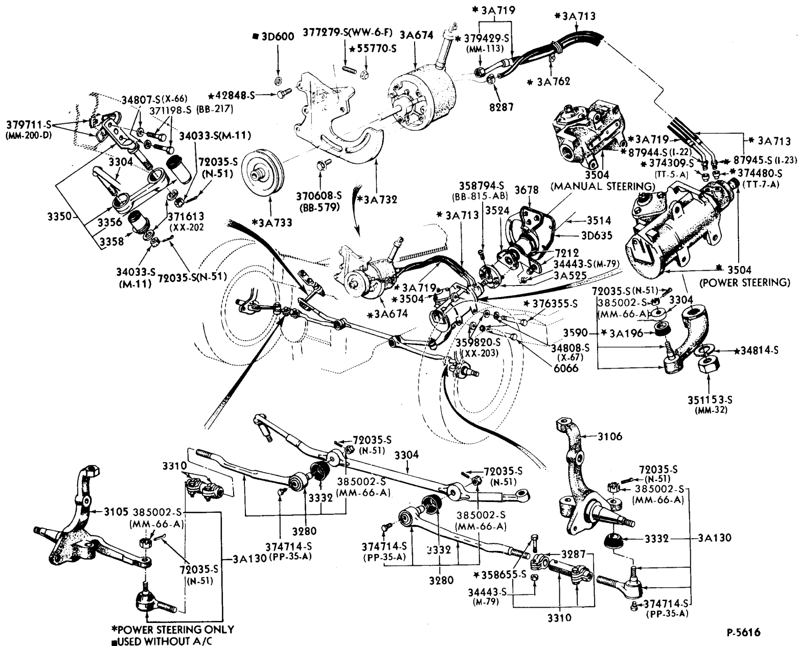
POWER STEERING SYSTEM (TYPICAL FOR MANUAL STEERING LINKAGE) 1967-69 FORD - 6 CYL.
