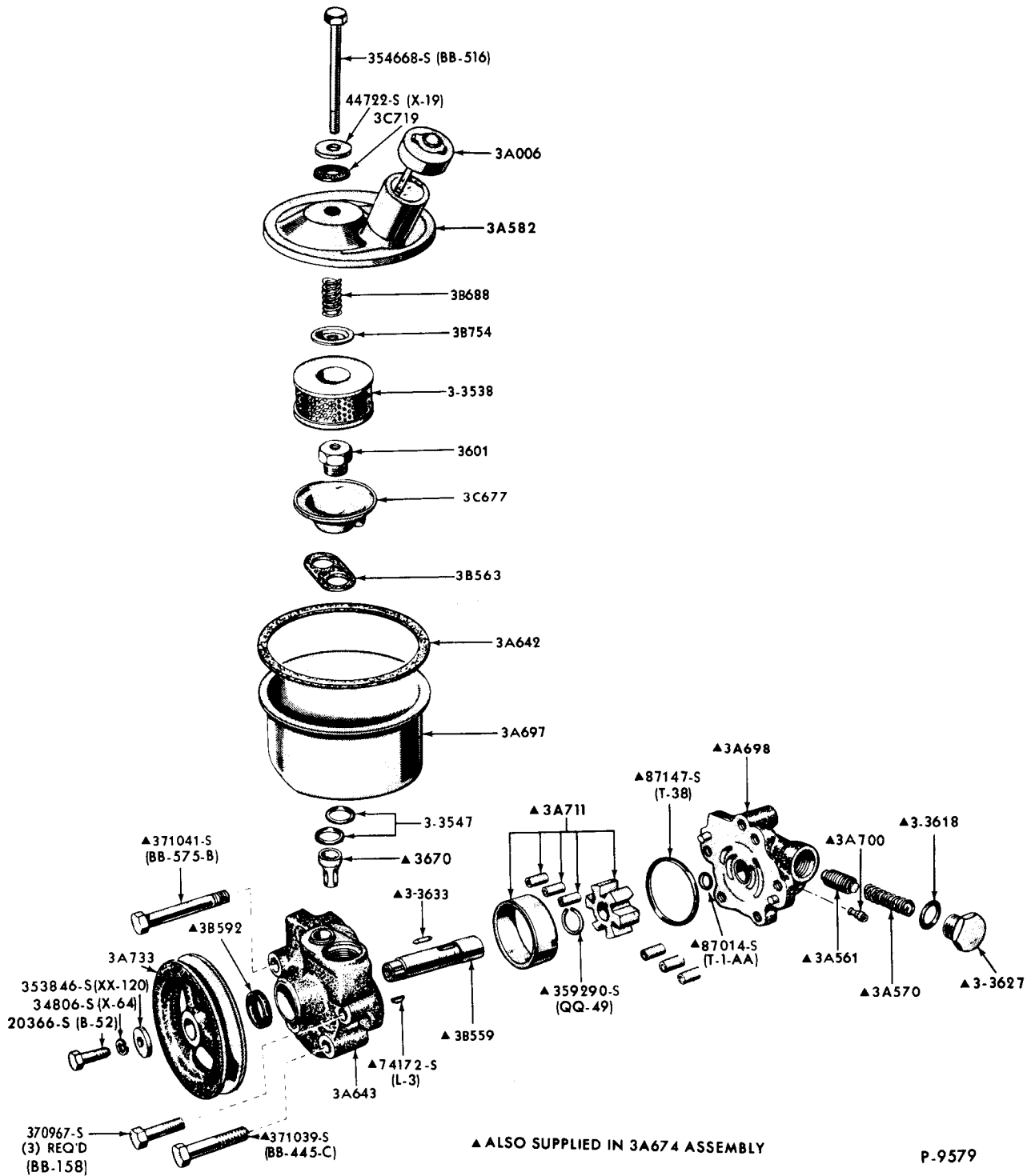
POWER STEERING PUMP & RELATED PARTS - (EATON TYPE) 1965 FORD, FAIRLANE, FALCON, MUSTANG & THUNDERBIRD
