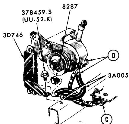
MUSTANG 302 "BOSS" ENGINE POWER STEERING OIL COOLER
