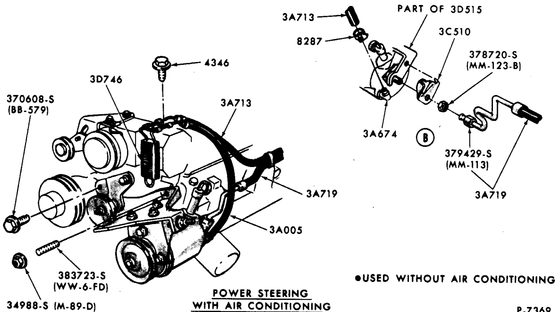
POWER STEERING PUMP INSTALLATION - TYPICAL 1970/72 FORD 8 CYL. 351, 400, 429, 1970/72 THUNDERBIRD 8 CYL. 400, (429 w/o A/C)
