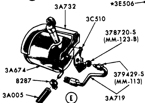
MUSTANG 302 "BOSS" ENGINE POWER STEERING OIL COOLER
