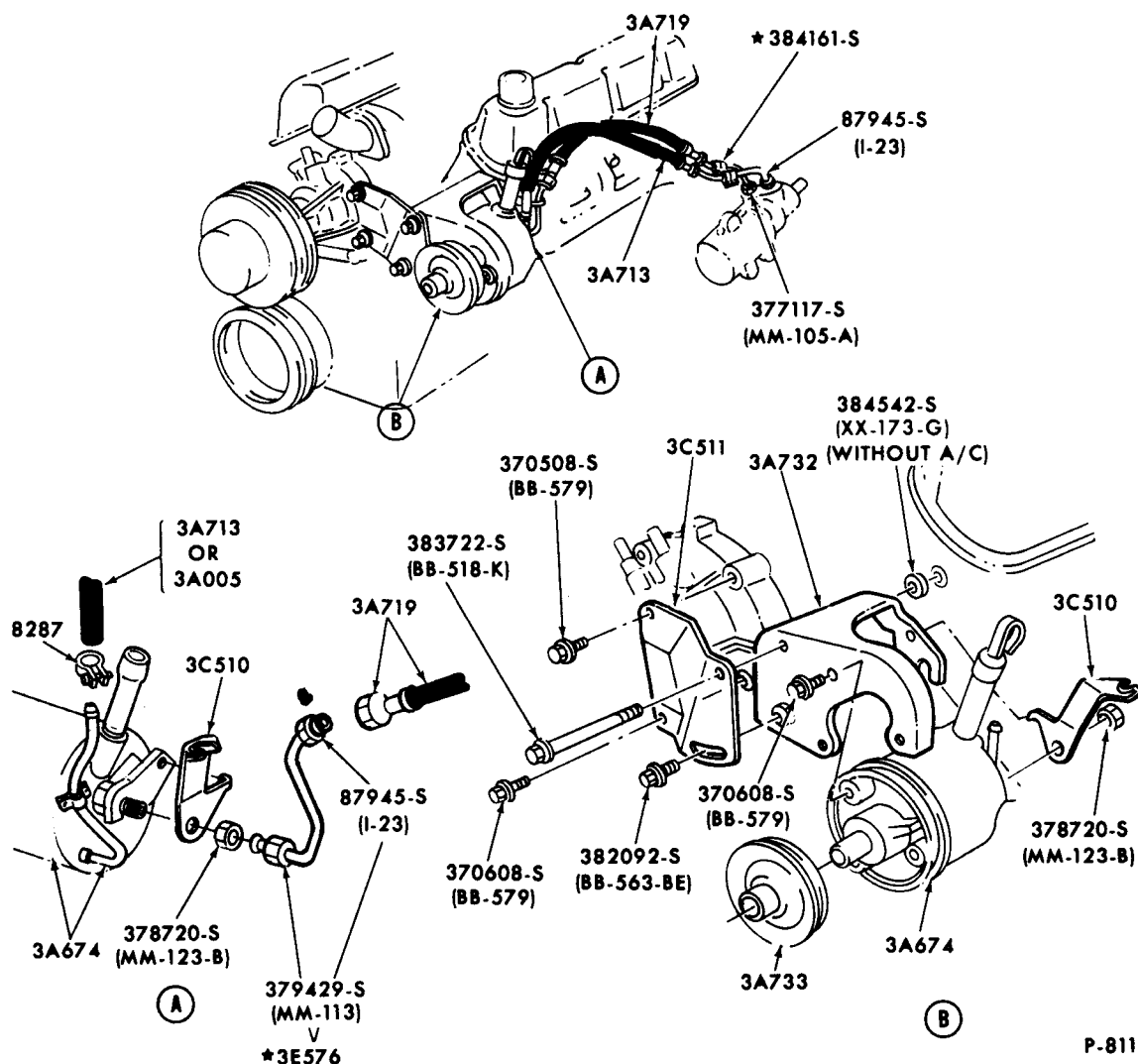
POWER STEERING WITHOUT AIR CONDITIONING
