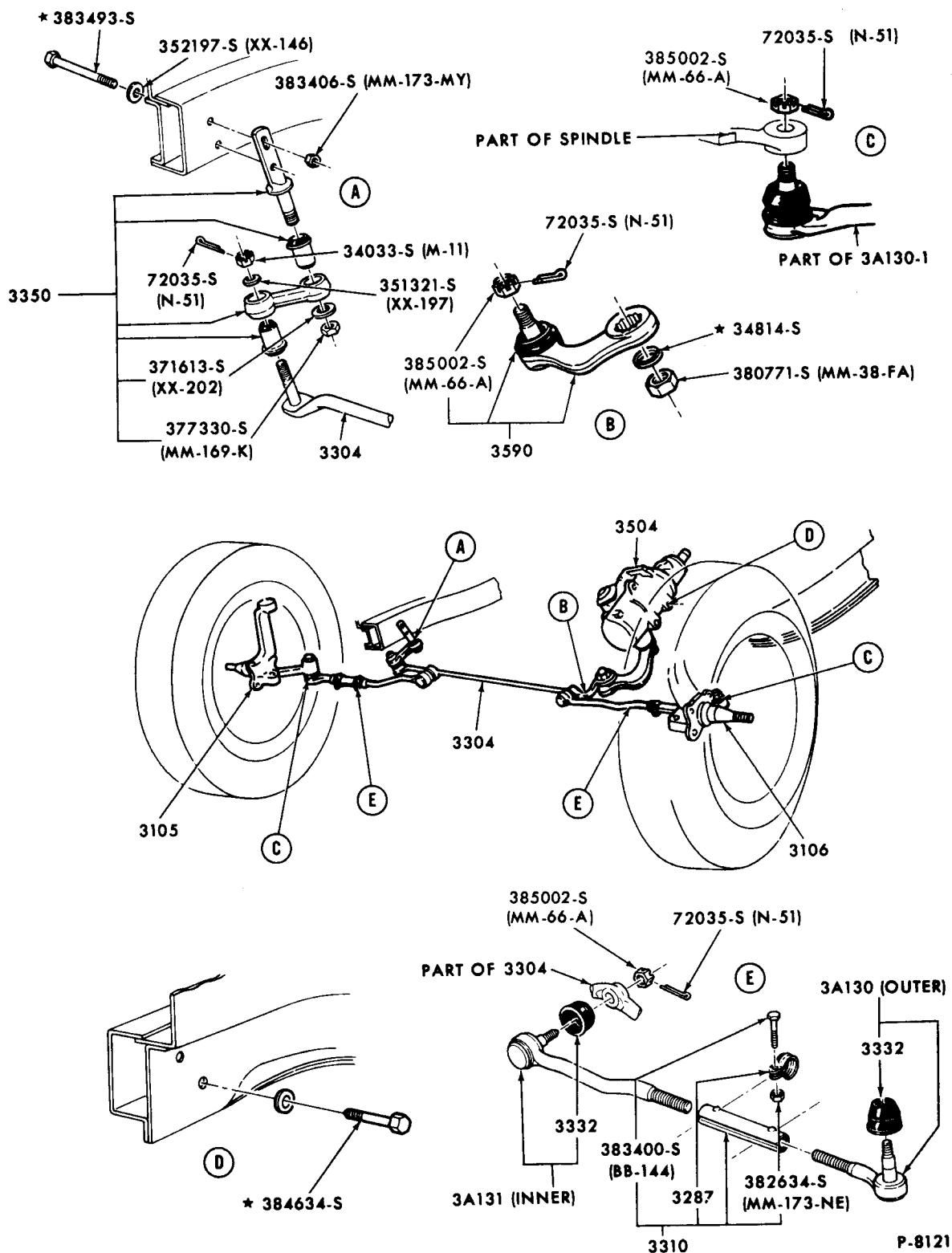
STEERING LINKAGE (POWER & MANUAL) - TYPICAL 1971/72 MUSTANG, 1972 THUNDERBIRD & TORINO
