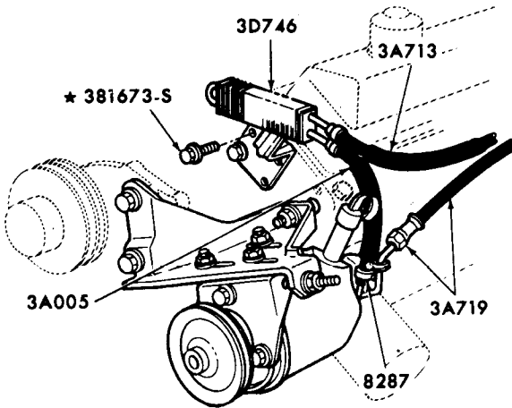
POWER STEERING WITHOUT AIR CONDITIONING
