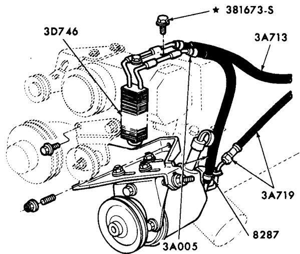
POWER STEERING WITH AIR CONDITIONING
