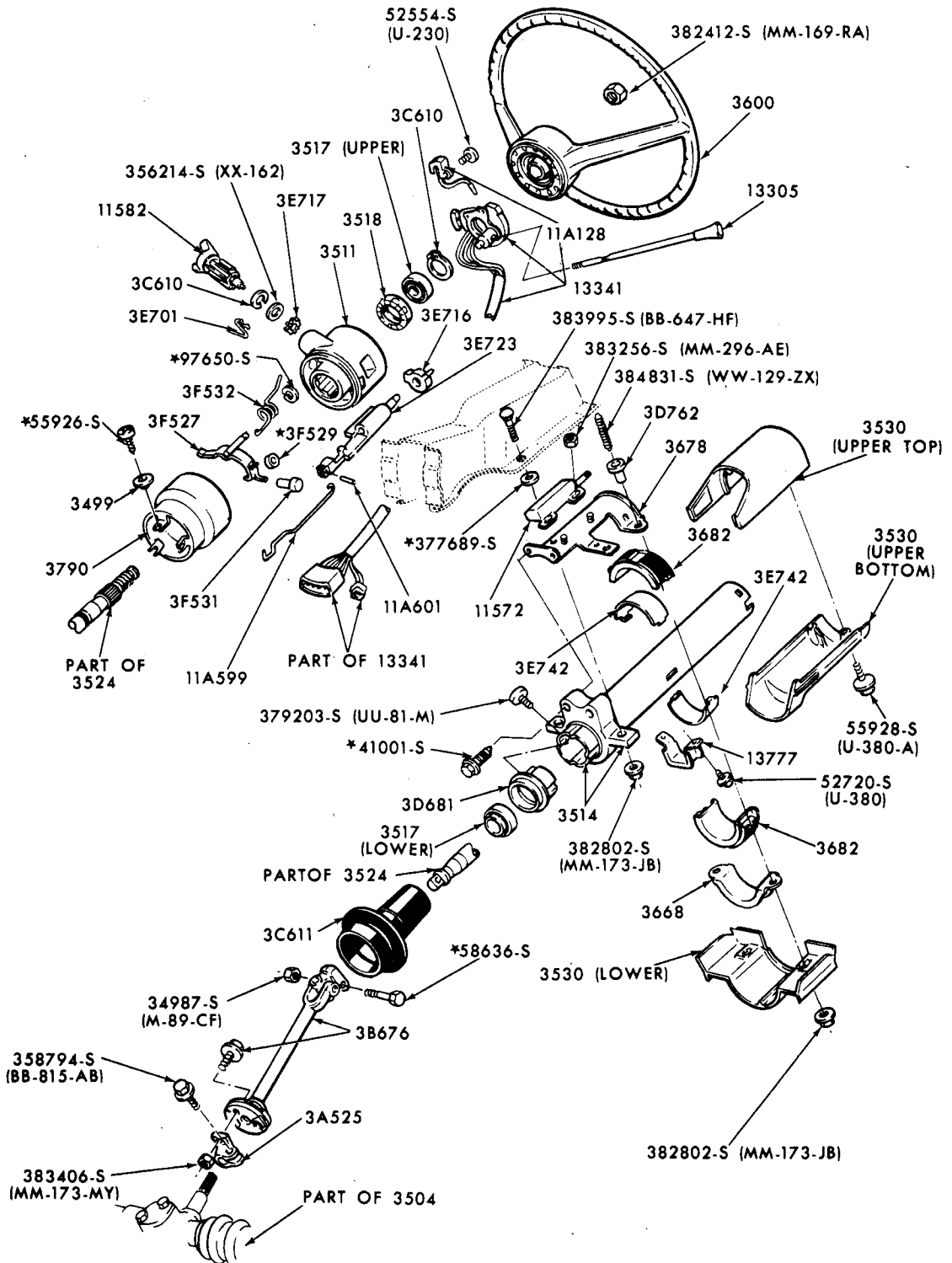
STEERING COLUMN FOR FLOOR SHIFT 1972 PINTO - "FROM 1/7/72"
