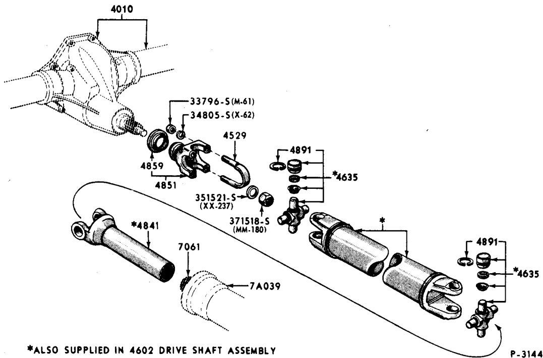
DRIVE SHAFT - TYPICAL 1965/72 MUSTANG, FAIRLANE/TORINO & 1965/70 FALCON 1970/72 MAVERICK, 1971/72 PINTO
