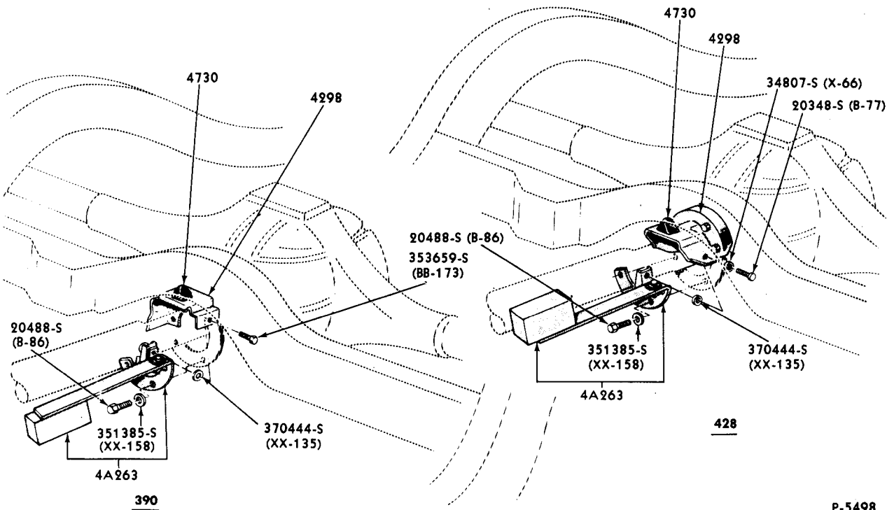
VIBRATION DAMPER - DRIVELINE 1966/67 FORD
