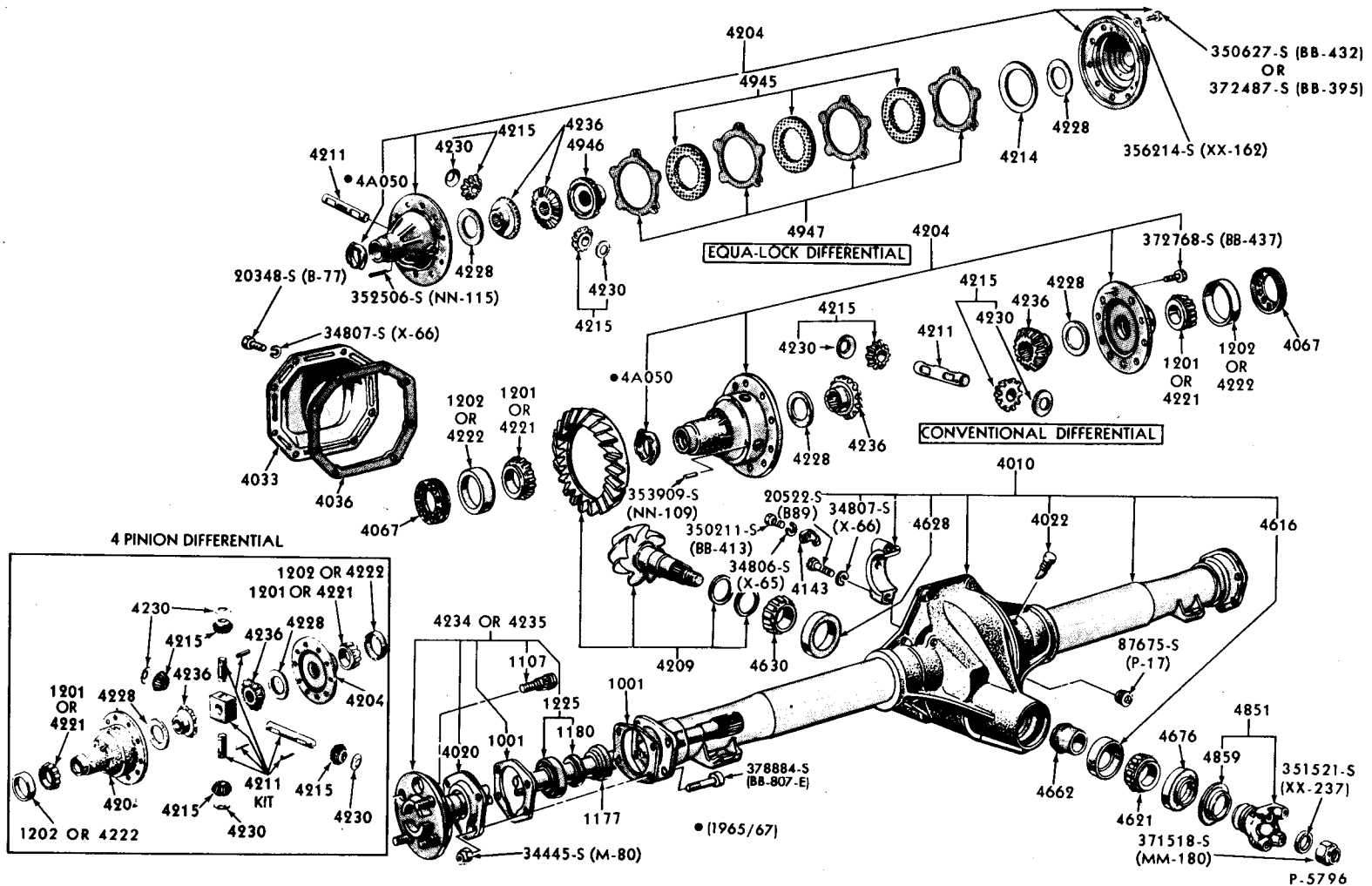
REAR AXLE - LOCKING (EQUA LOCK) & NON-LOCKING WITH INTEGRAL CARRIER - TYPICAL 6 3/4", 7 1/4" RING GEARS 1965/70 FALCON, 1971/72 MAVERICK, 1965/70 MUSTANG, 1971/72 PINTO
