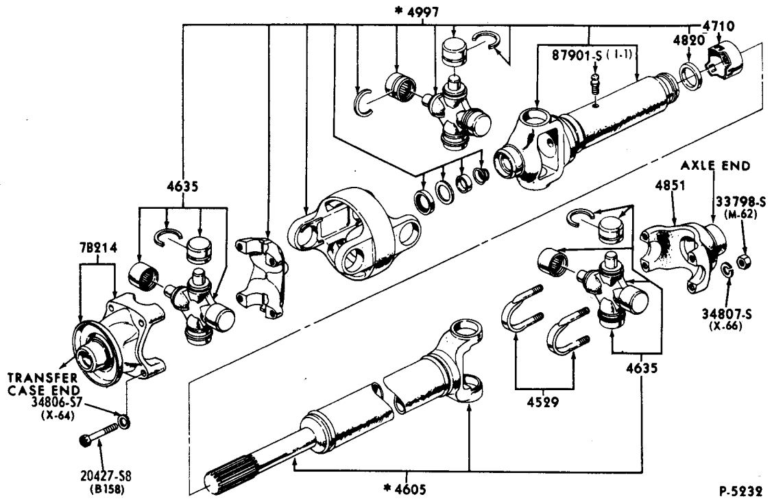
DRIVE SHAFT - MECHANICS TYPE 1966/70 BRONCO - "BEFORE SER. G70,001"
