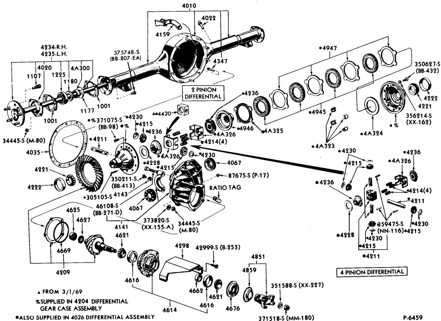
REAR AXLE-LOCKING (TRACTION LOK)-TYPICAL
