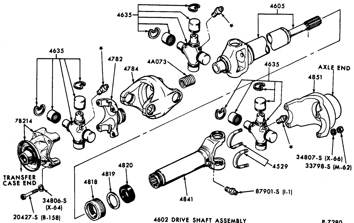
DRIVE SHAFT - DANA TYPE 1970/72 BRONCO - FROM SER. G70,001
