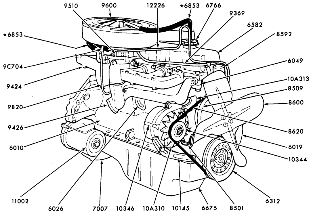
RIGHT-FRONT VIEW
