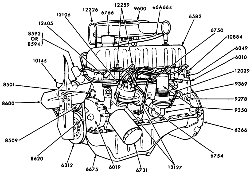
LEFT-FRONT VIEW
