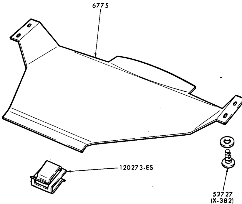
ENGINE SPLASH SHIELD 1971/72 PINTO
