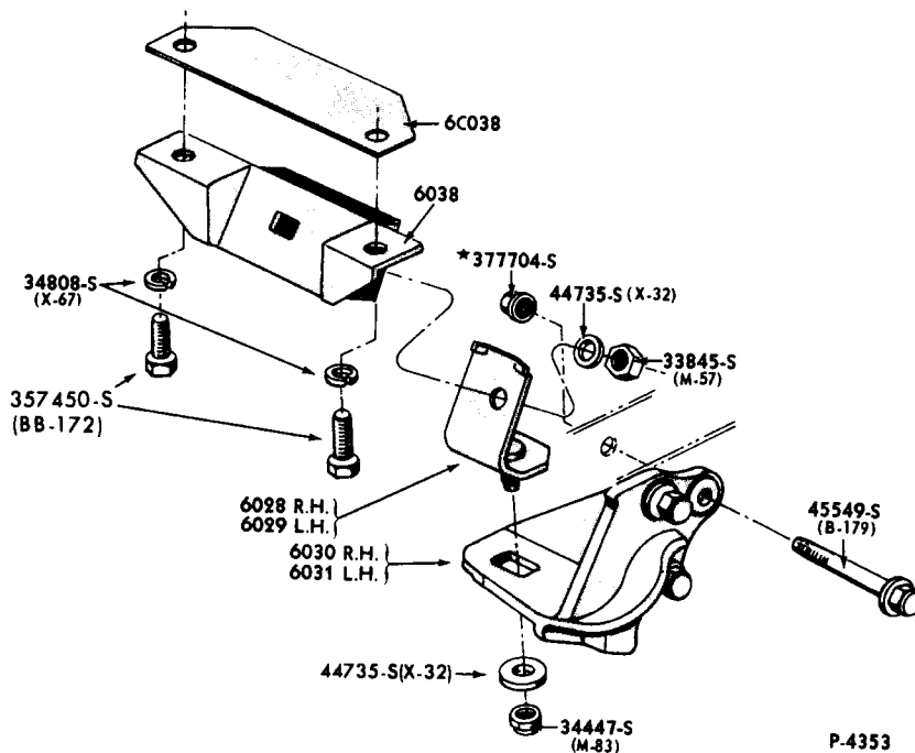
ENGINE SUPPORTS, INSULATORS and RELATED PARTS - FRONT 1965 FALCON - 8 CYLINDER 289
