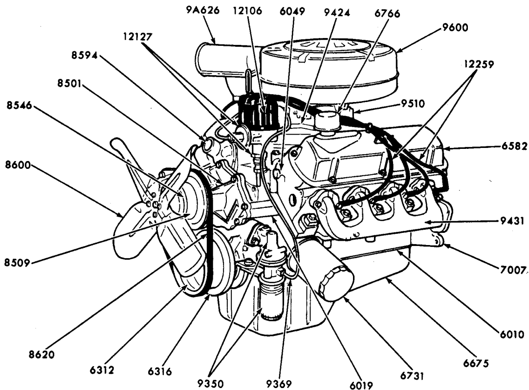
LEFT-FRONT VIEW
