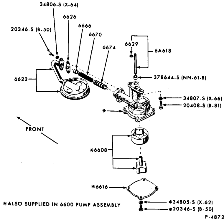
ENGINE OIL PUMP and RELATED PARTS 1965/72 6 CYLINDER 240
