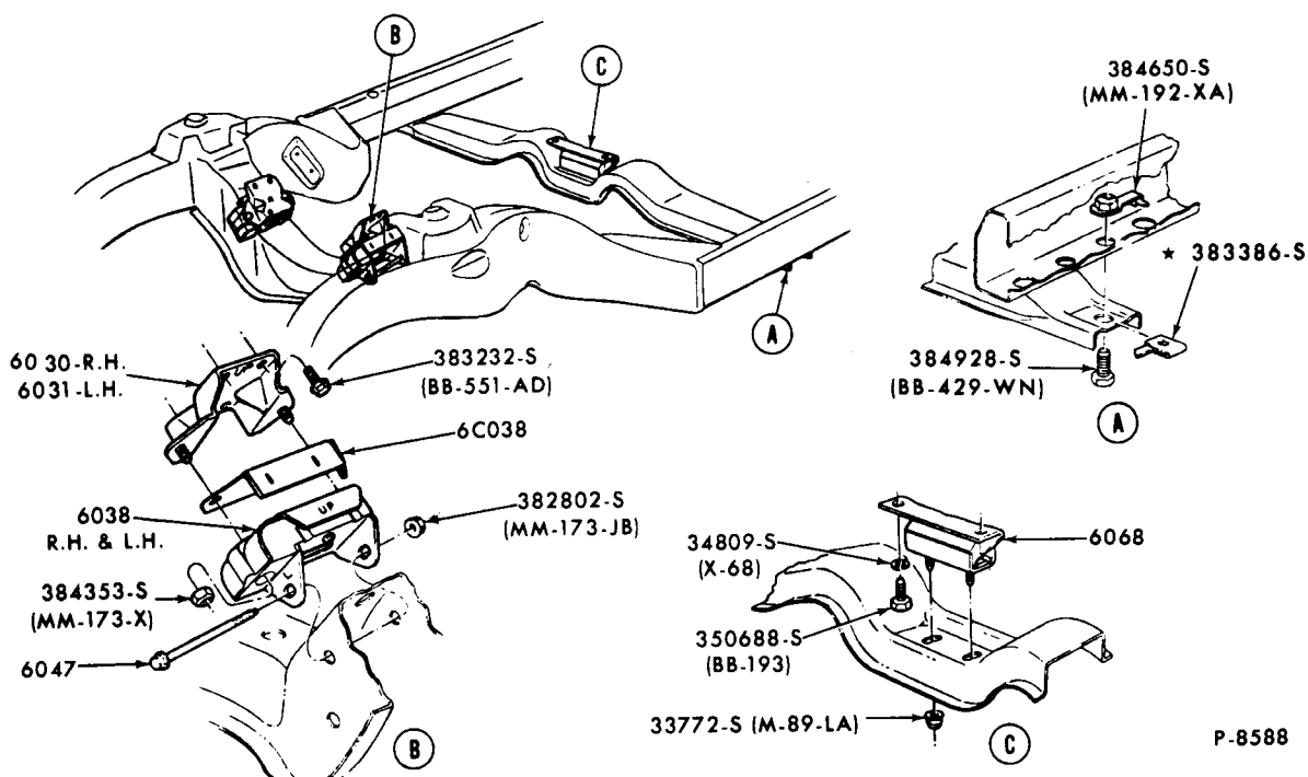
ENGINE SUPPORTS, INSULATORS and RELATED PARTS - FRONT and REAR 1972 TORINO - 8 CYLINDER 429
