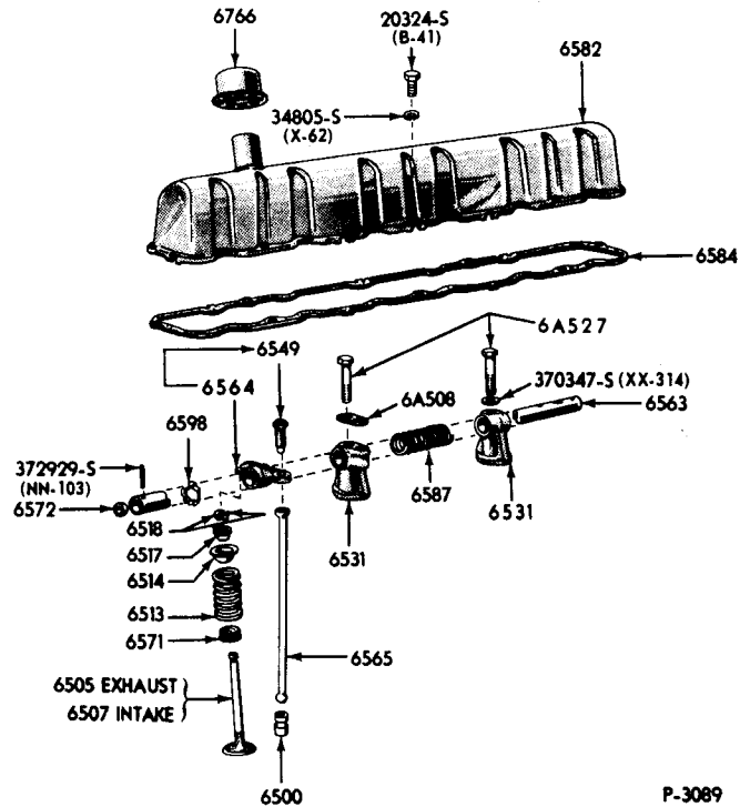
ENGINE VALVES, PUSH RODS, ROCKER ARM COVER and RELATED PARTS -- TYPICAL 1965/72 6 CYLINDER 170, 200 and 250
