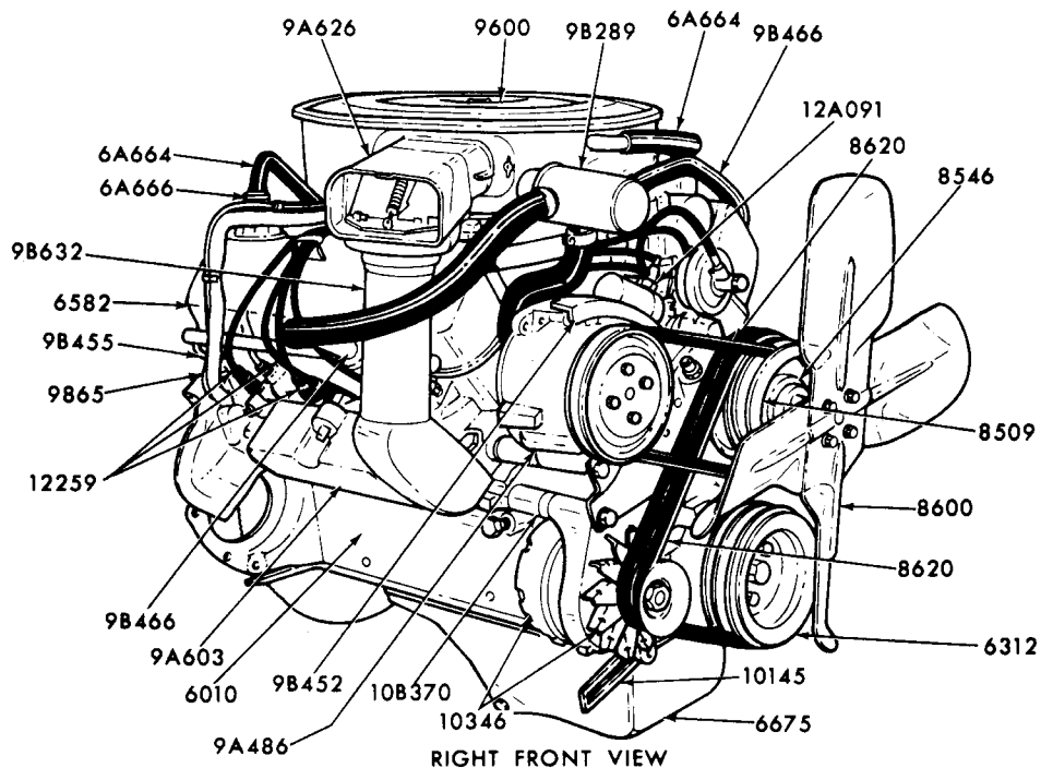
ENGINE ASSEMBLY - 8 CYLINDER 390 and 428 - TYPICAL 1968/71
