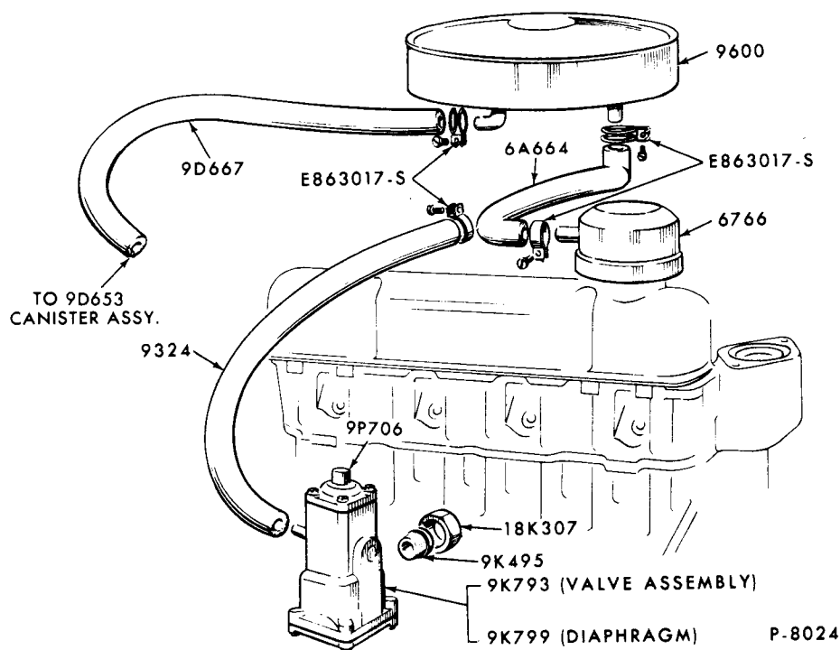
ENGINE EMISSION SYSTEM 1971/72 4 CYLINDER 122 (2000cc)
