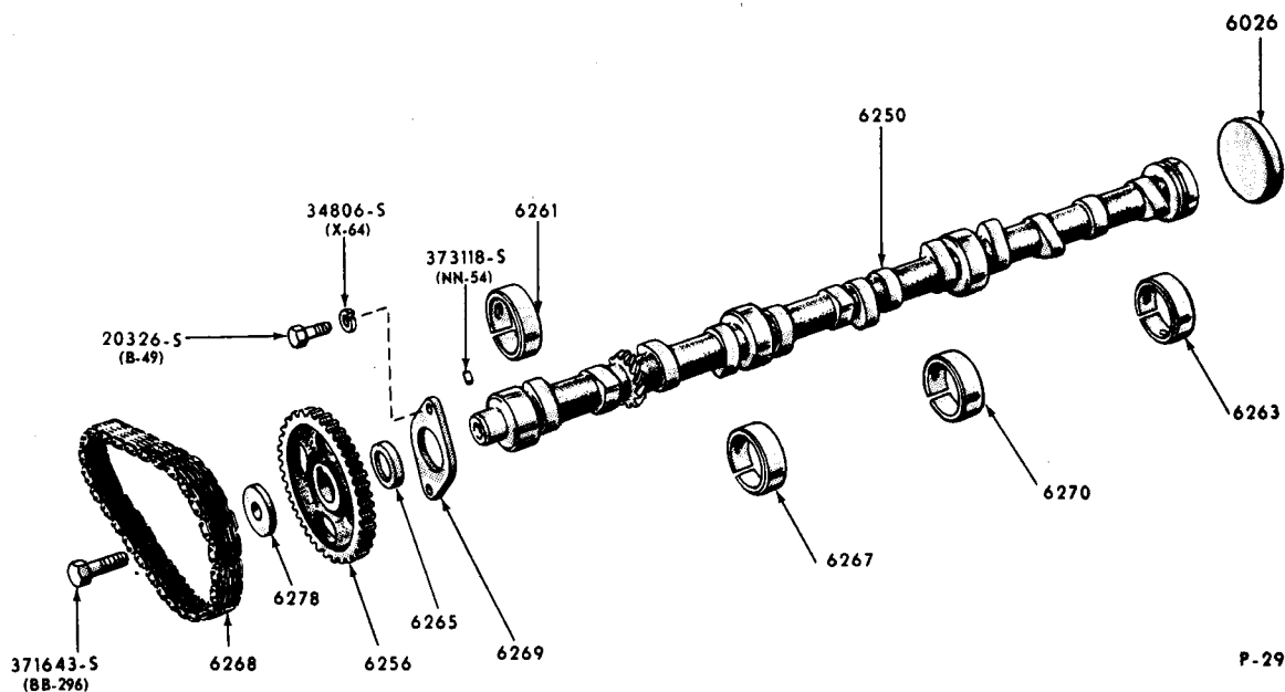
ENGINE CAMSHAFT, GEAR, BEARINGS and RELATED PARTS -- TYPICAL 1965/72 6 CYLINDER 170, 200 and 250
