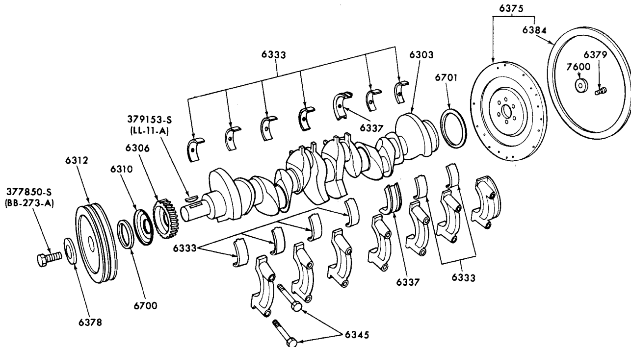
ENGINE CRANKSHAFT, FLYWHEEL and RELATED PARTS -- TYPICAL 1965/72 6 CYLINDER 240
