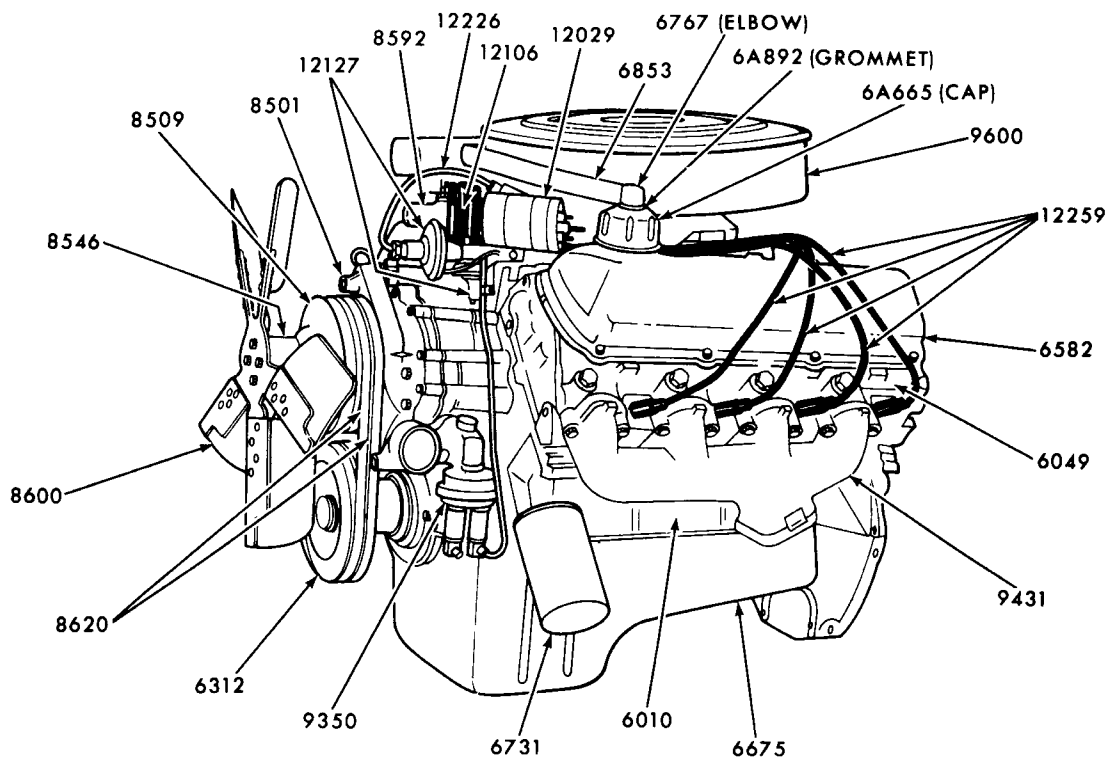
LEFT-FRONT VIEW
