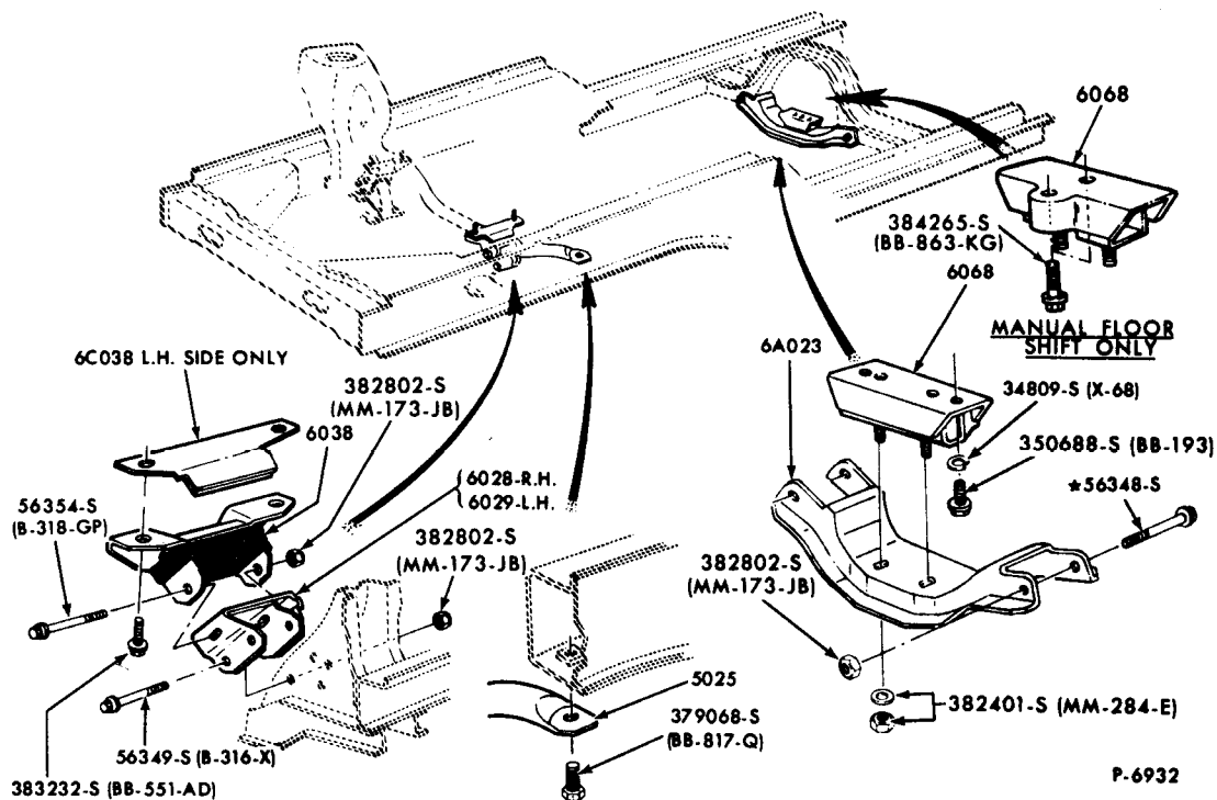
ENGINE SUPPORTS, INSULATORS and RELATED PARTS - FRONT and REAR 1971/72 MAVERICK - 8 CYLINDER 302
