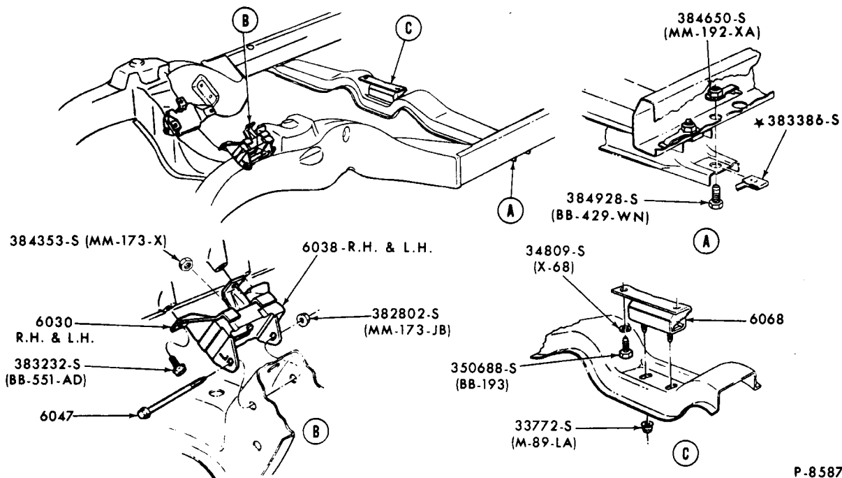
ENGINE SUPPORTS, INSULATORS and RELATED PARTS - FRONT and REAR 1972 TORINO - 8 CYLINDER 400
