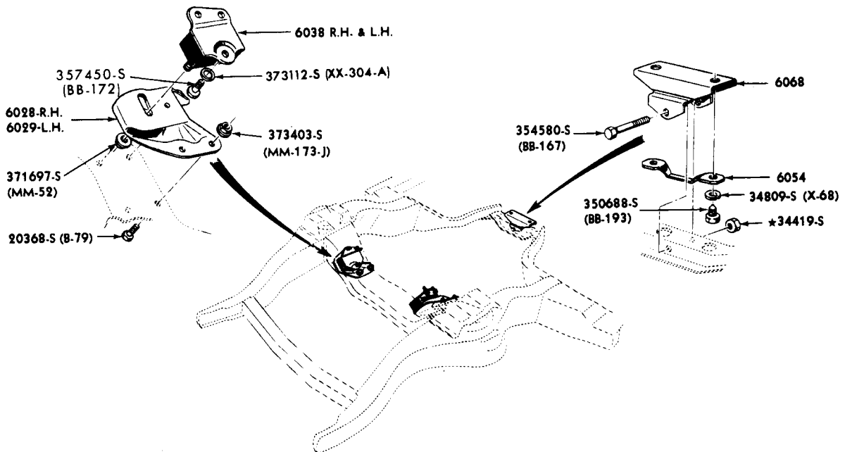
ENGINE SUPPORTS, INSULATORS and RELATED PARTS - FRONT and REAR 1987 THUNDERBIRD - 8 CYLINDER 390, 428
