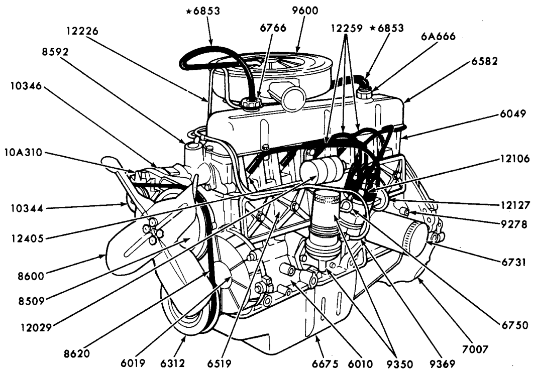
LEFT-FRONT VIEW
