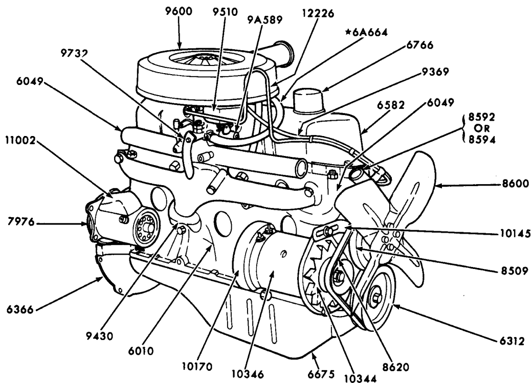
RIGHT-FRONT VIEW
