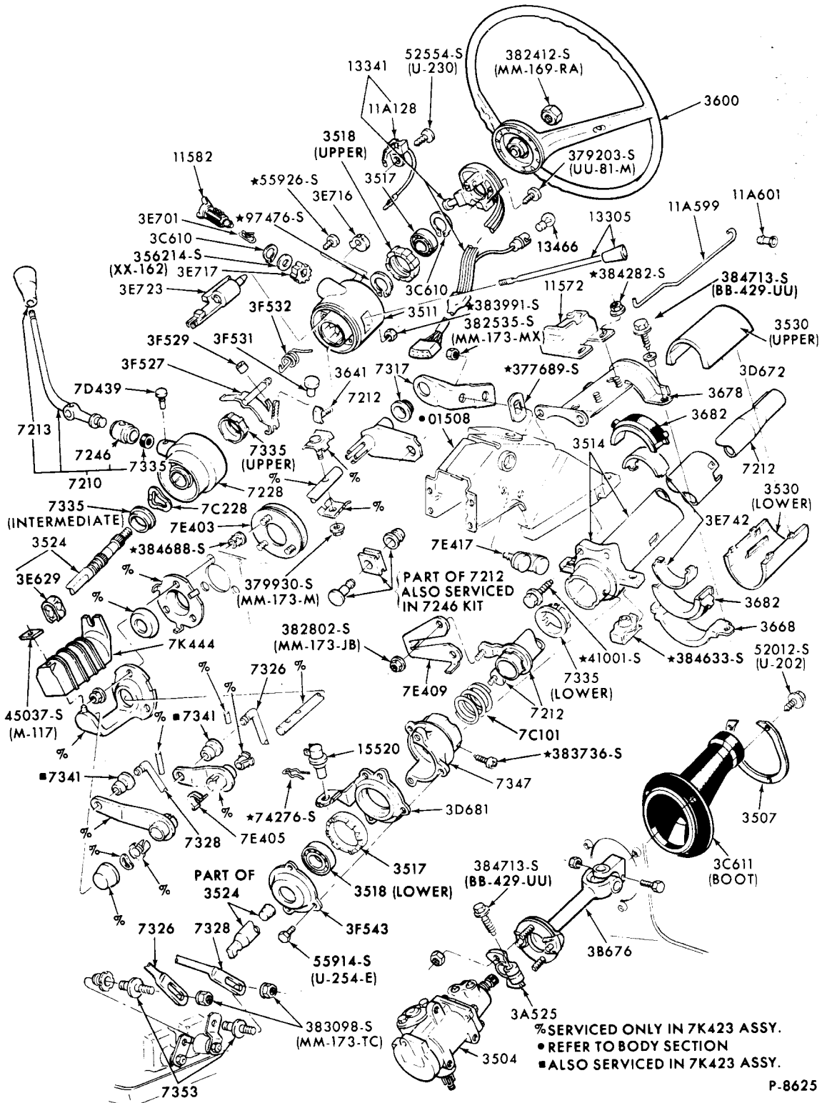
STEERING COLUMN and SHIFT MECHANISM - LOCKING 3 SPEED MANUAL TRANSMISSION 1972 TORINO
