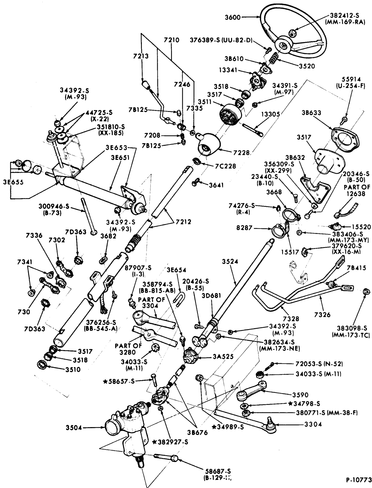
STEERING COLUMN AND SHIFT MECHANISM-POWER STEERING 1972 BRONCO
