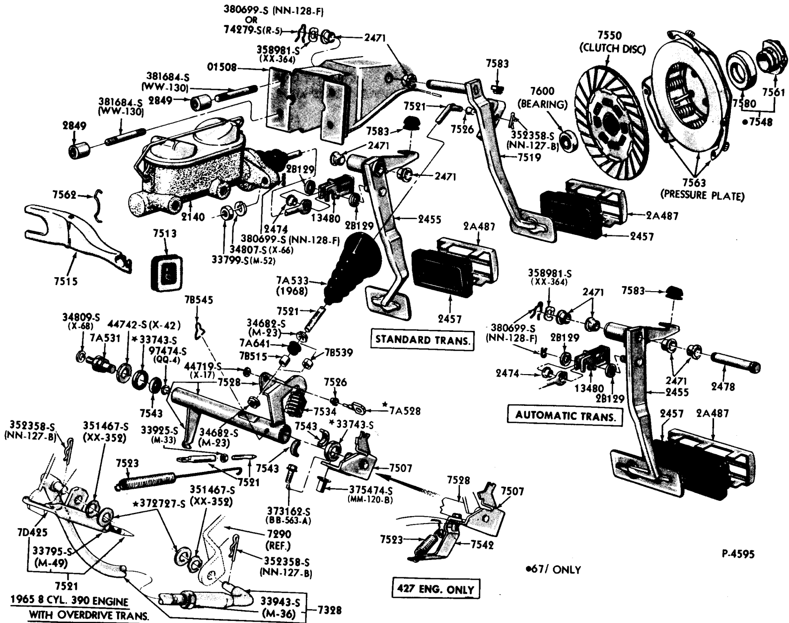
CLUTCH, CLUTCH PEDAL, and BRAKE PEDAL
