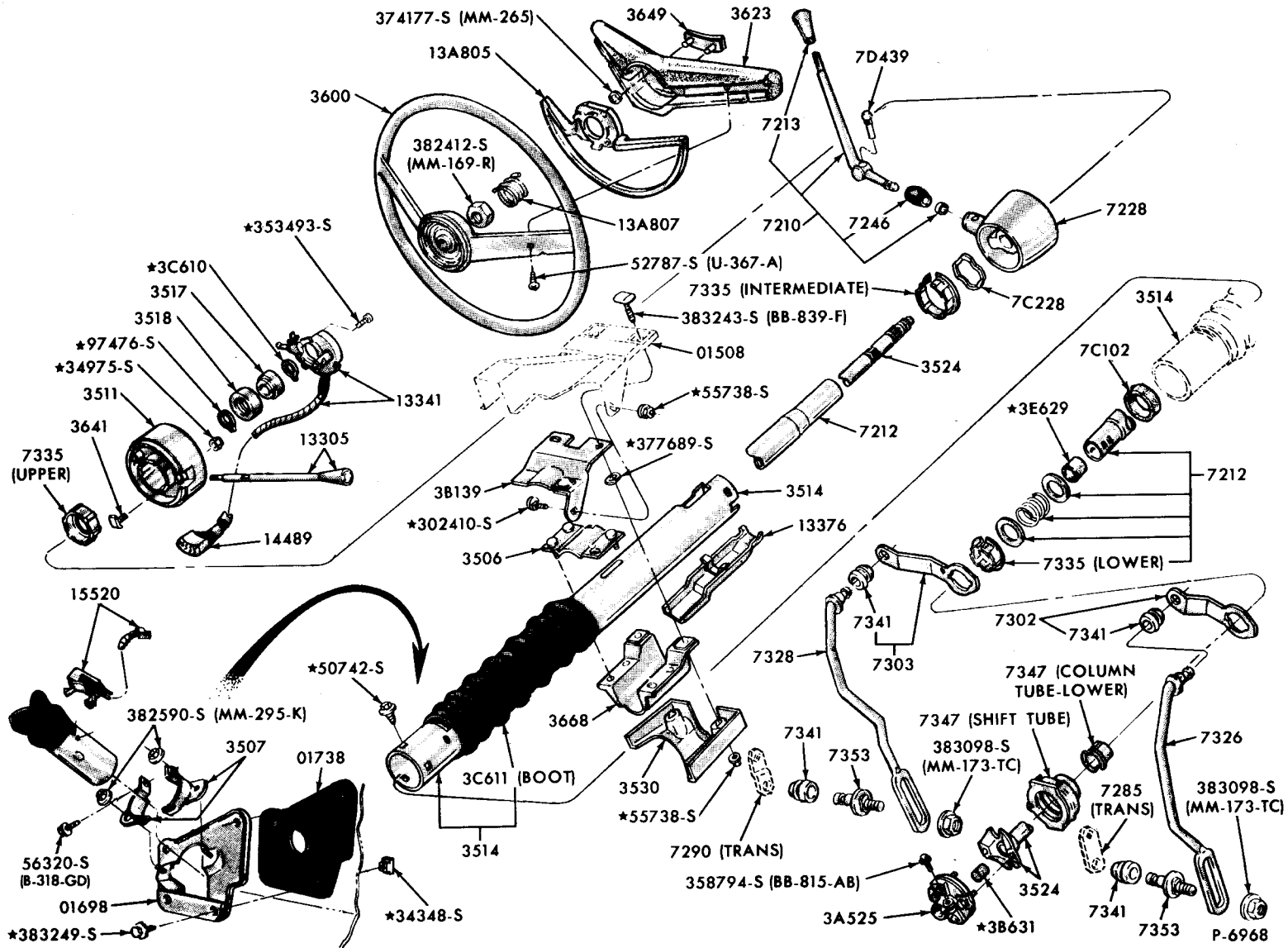
STEERING COLUMN & SHIFT MECHANISM - NON LOOKING 3 SPEED MANUAL TRANSMISSION 1970 MAVERICK
