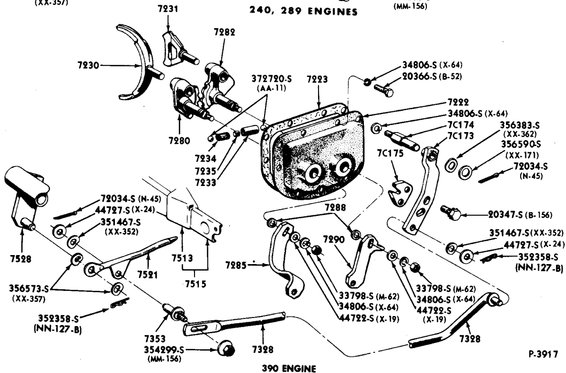
GEAR SHIFT & INTERLOCK LINKAGE - TYPICAL OVERDRIVE TRANSMISSION 1965/67 FORD - 6 & 8 CYL.
