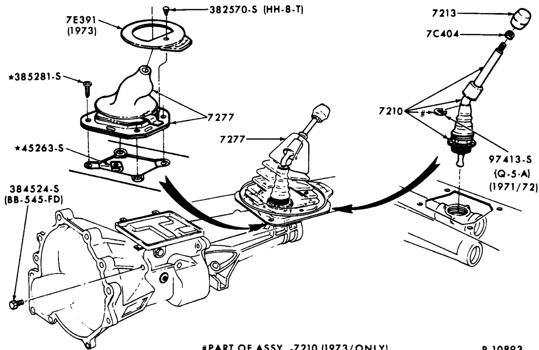
GEAR SHIFT MECHANISM 4 SPEED MANUAL TRANSMISSION 1971/72 PINTO
