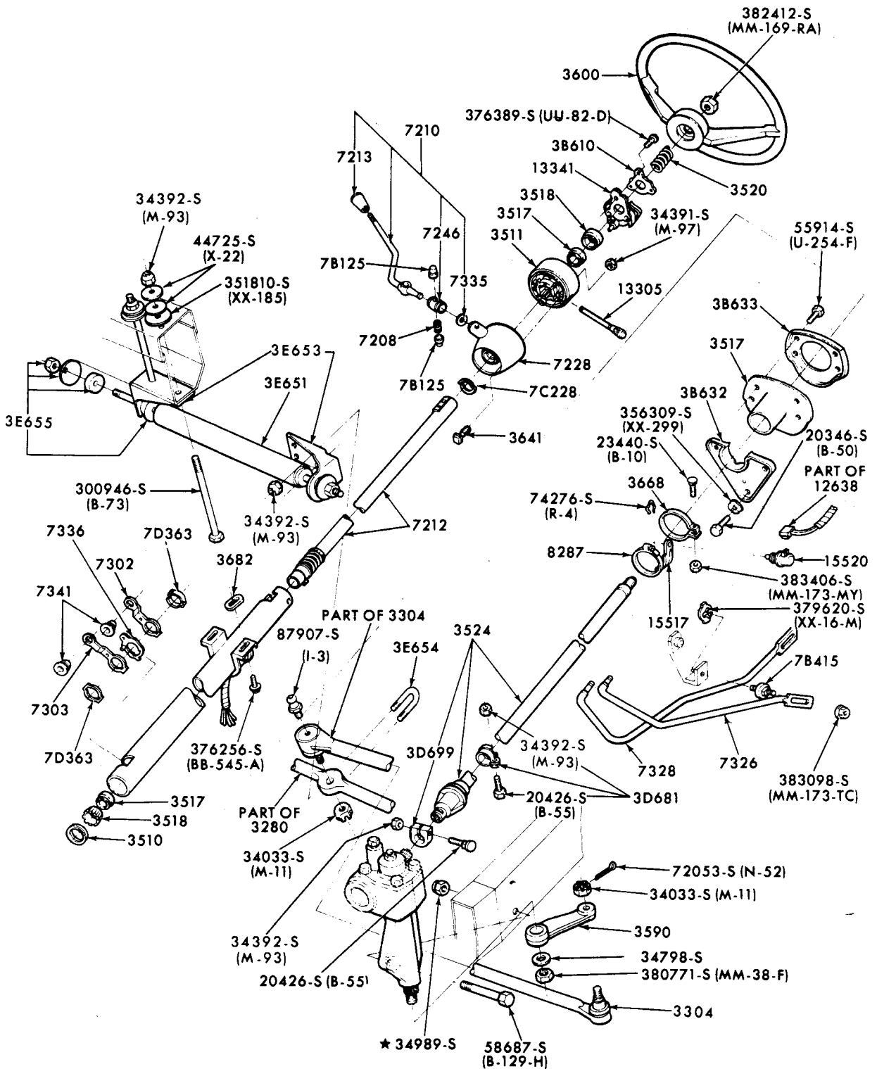
STEERING COLUMN AND SHIFT MECHANISM-MANUAL STEERING 1972 BRONCO
