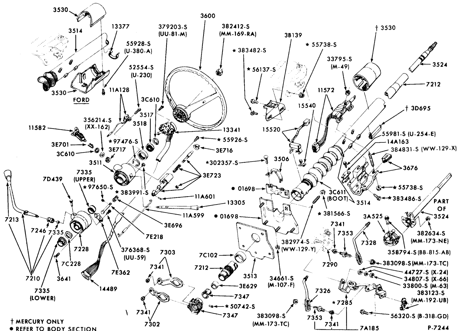
STEERING COLUMN & SHIFT MECHANISM - LOCKING 3 SPEED MANUAL TRANSMISSION 1970/71 FORD
