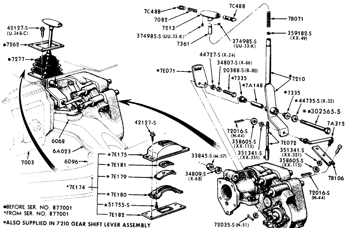
TRANSFER CASE SHIFT LINKAGE 1966/72 BRONCO - FROM SER. 830,001
