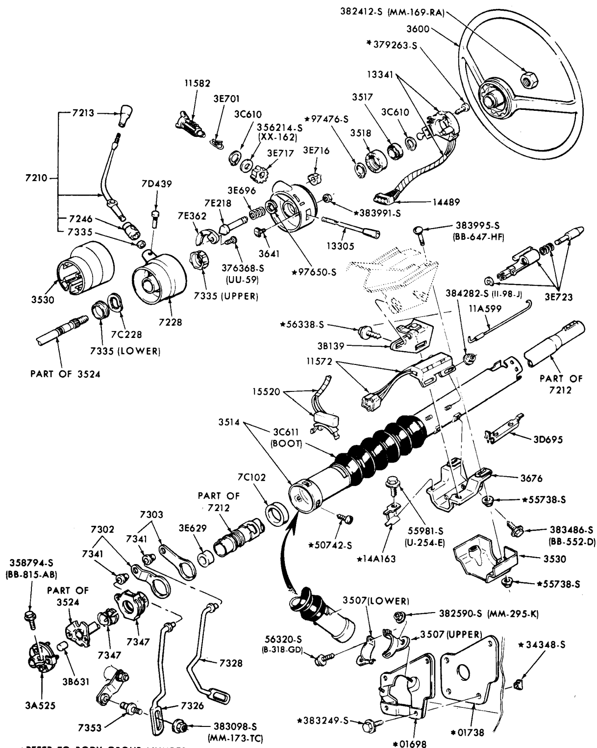
STEERING COLUMN & SHIFT MECHANISM - LOCKING 3 SPEED MANUAL TRANSMISSION 1970/72 MAVERICK
