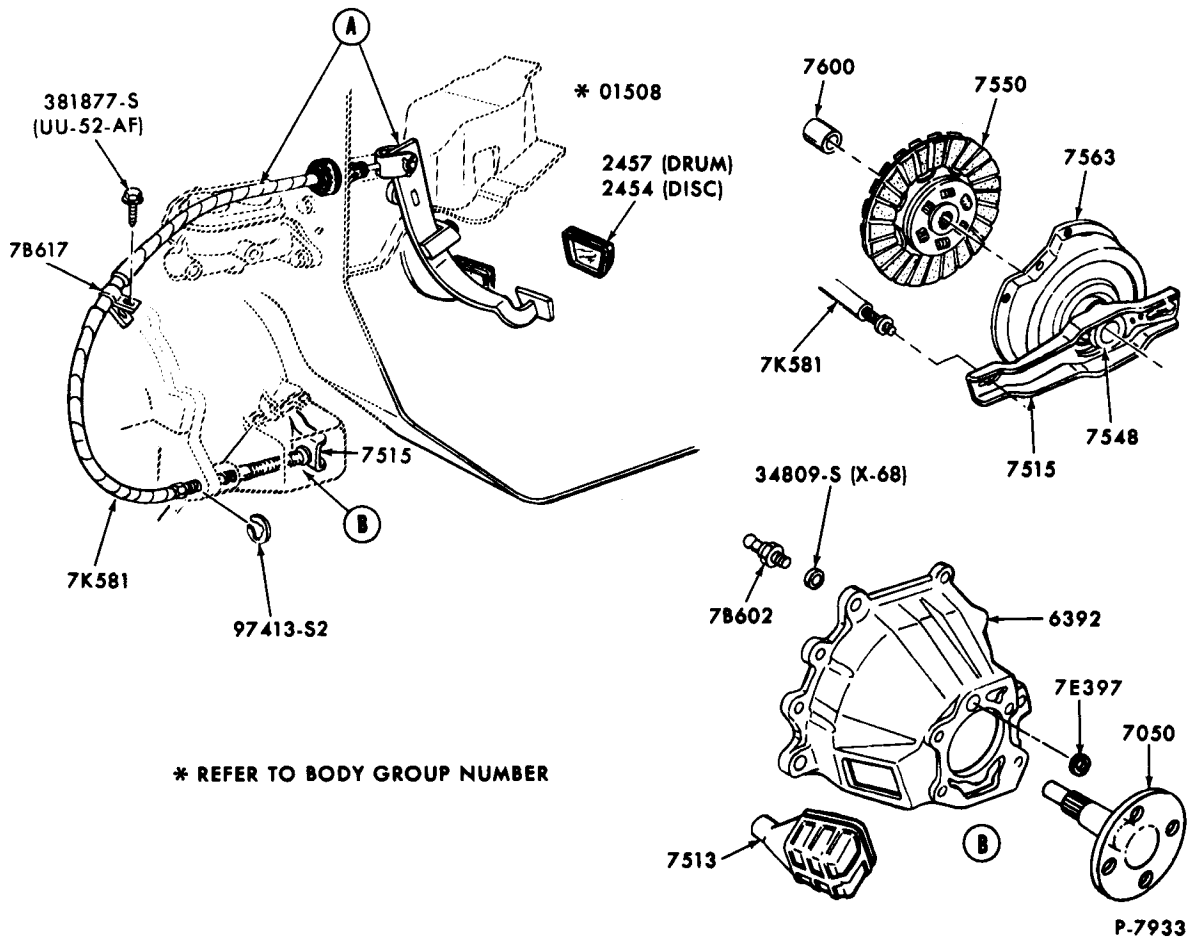
CLUTCH, CLUTCH PEDAL and BRAKE PEDAL 1971/72 PINTO
