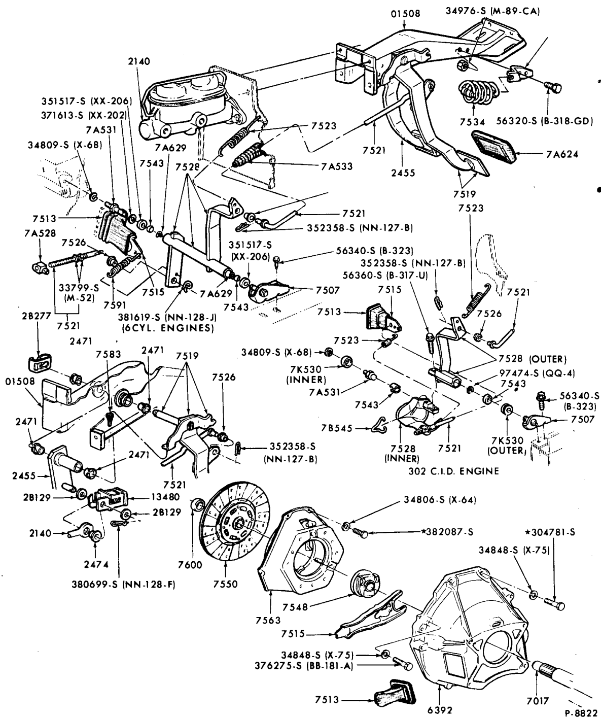
CLUTCH, CLUTCH PEDAL and BRAKE PEDAL 1970/72 MAVERICK
