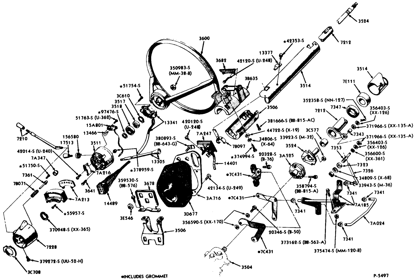
STEERING COLUMN &amp; SHIFT CONTROL SELECTOR MECHANISM
