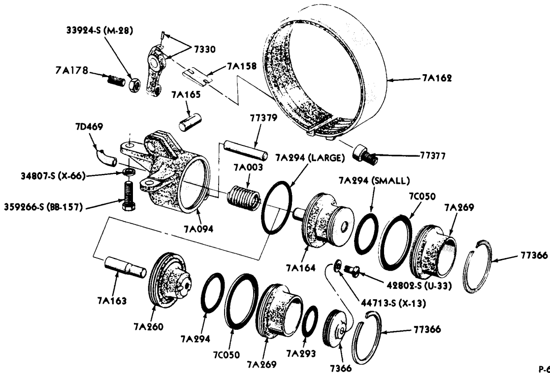
FRONT SERVO & BAND-TYPICAL 1968/72 FORD, 1969/72 FAIRLANE/TORINO & MUSTANG
