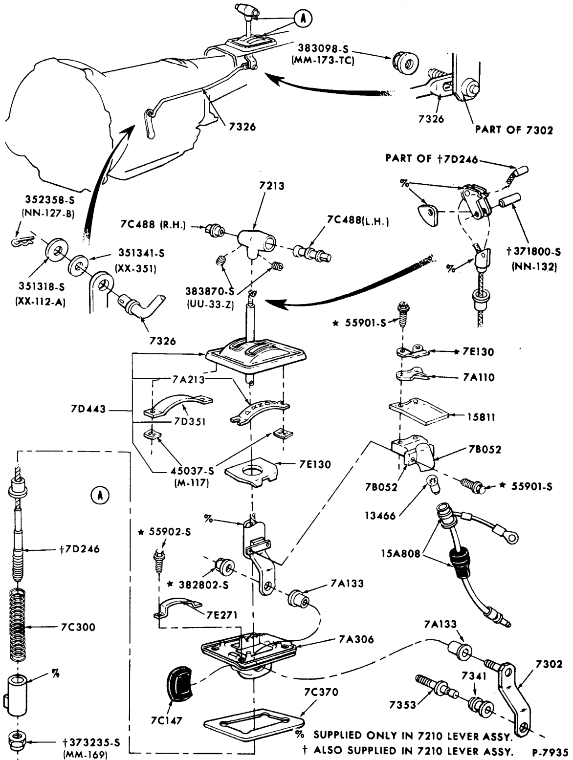
SHIFT CONTROL SELECTOR MECHANISM - FLOOR MOUNTED 1971/72 PINTO
