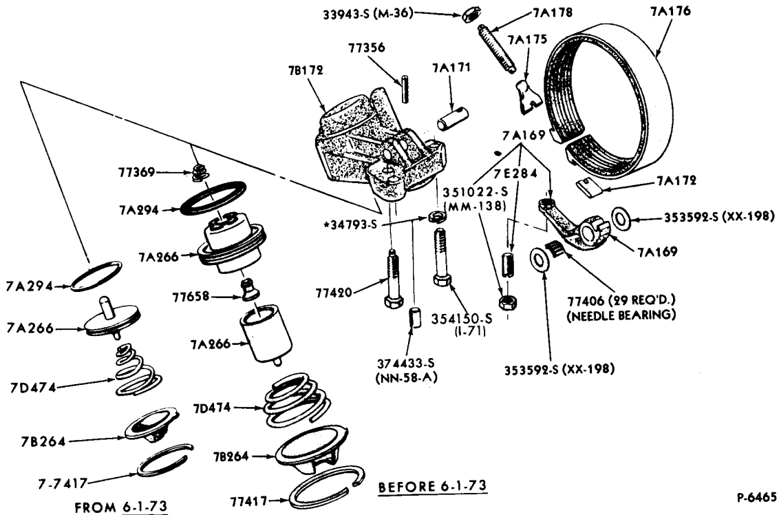
REAR SERVO & BAND-TYPICAL 1968/72 FORD, 1969/72 FAIRLANE/TORINO & MUSTANG
