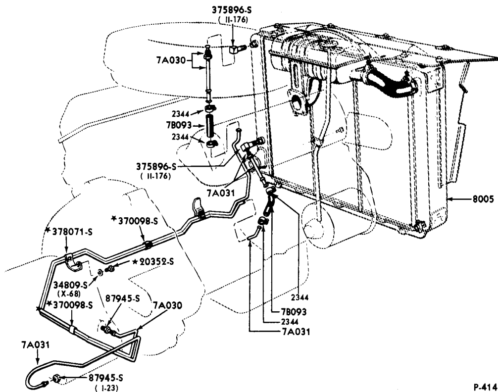
TRANSMISSION OIL COOLING SYSTEM-TYPICAL 1965/66 THUNDERBIRD
