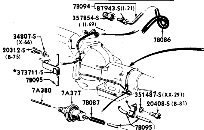
8 CYLINDER 302 & 351 ENGINES WITH C/M & C4 TRANSMISSIONS
