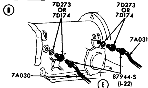
8 CYLINDER 429 ENGINE
