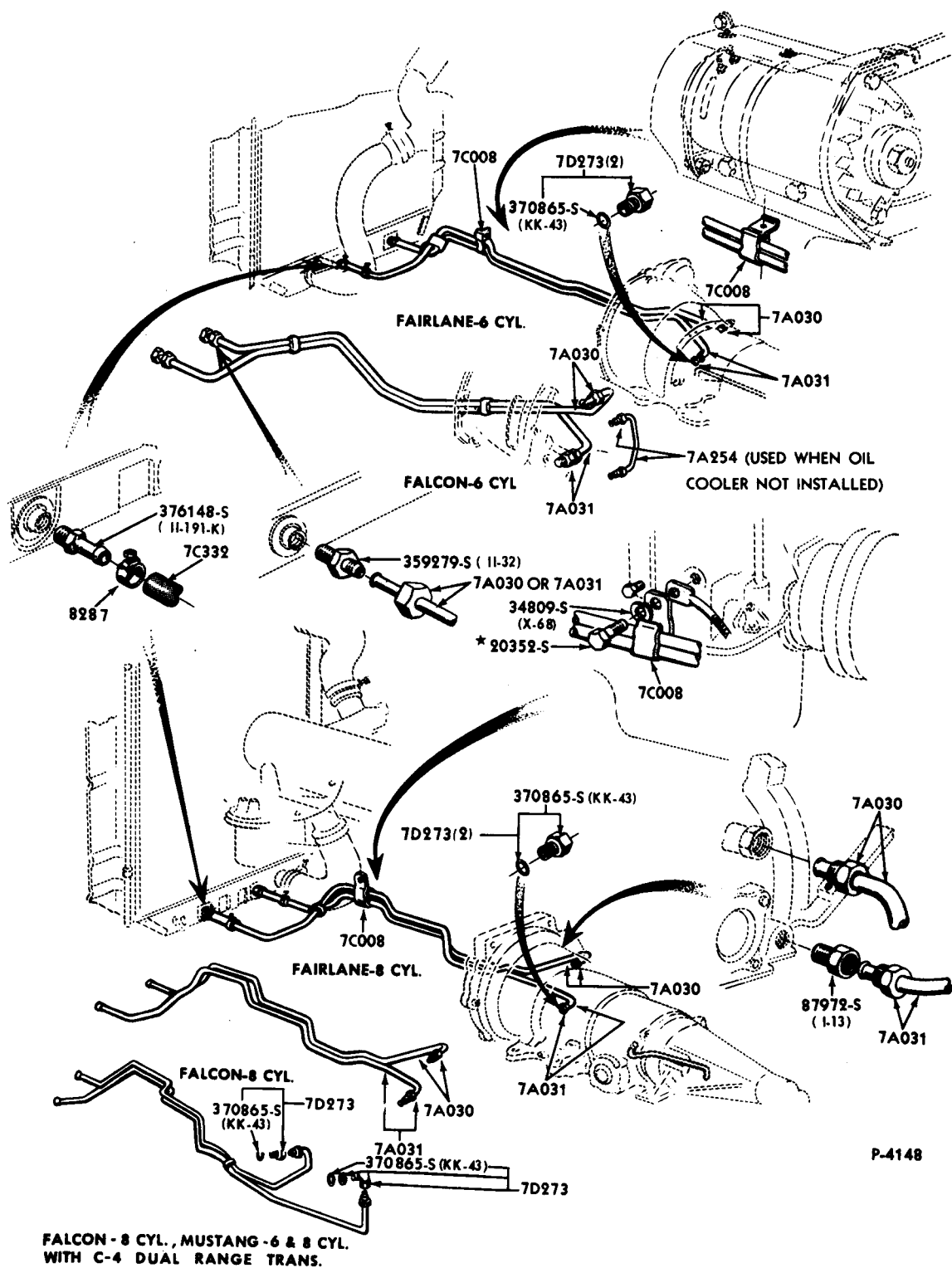
TRANSMISSION OIL COOLING SYSTEM-TYPICAL 1965 FAIRLANE, MUSTANG & FALCON
