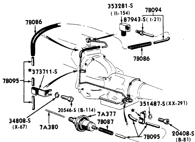
8 CYLINDER 400, 429 & 460 ENGINES WITH C/M & C/6 TRANSMISSIONS
