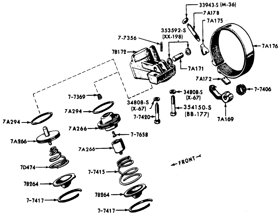
REAR SERVO & BAND-TYPICAL 1965/68 FORD, 1965/66 THUNDERBIRD
