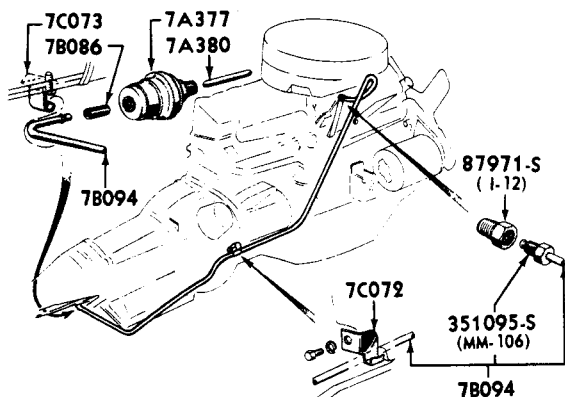
6 CYLINDER 200 & 250 ENGINES
