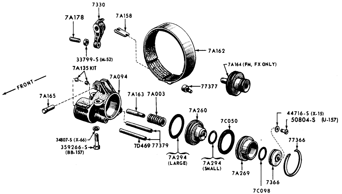
FRONT SERVO & BAND-TYPICAL 1965/68 FORD, 1965/66 THUNDERBIRD
