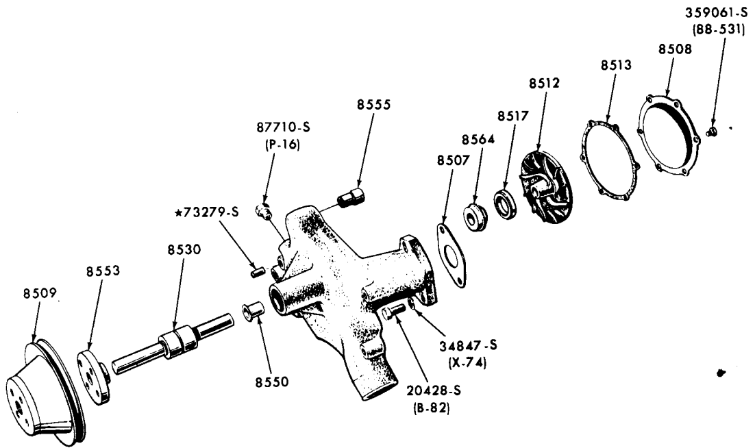
WATER PUMP 1965/71 8 CYLINDER 352,390,427 and 428
