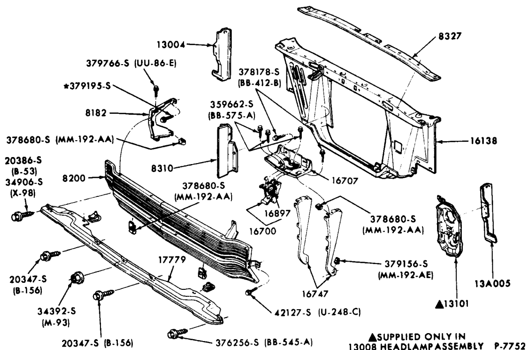
RADIATOR GRILLE and RELATED PARTS 1966 FORD - BODY TYPES 54A, E, 57B, 62B, E, 63B, 71B, C, D, 76A
