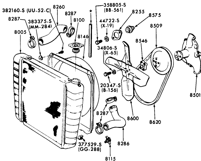
COOLING SYSTEM and RELATED PARTS - TYPICAL 1967/72 FORD, THUNDERBIRD - 6 CYLINDER 240 & 8 CYLINDER 289, 302, 351, 390, 400, 428, 429 ENGINES
