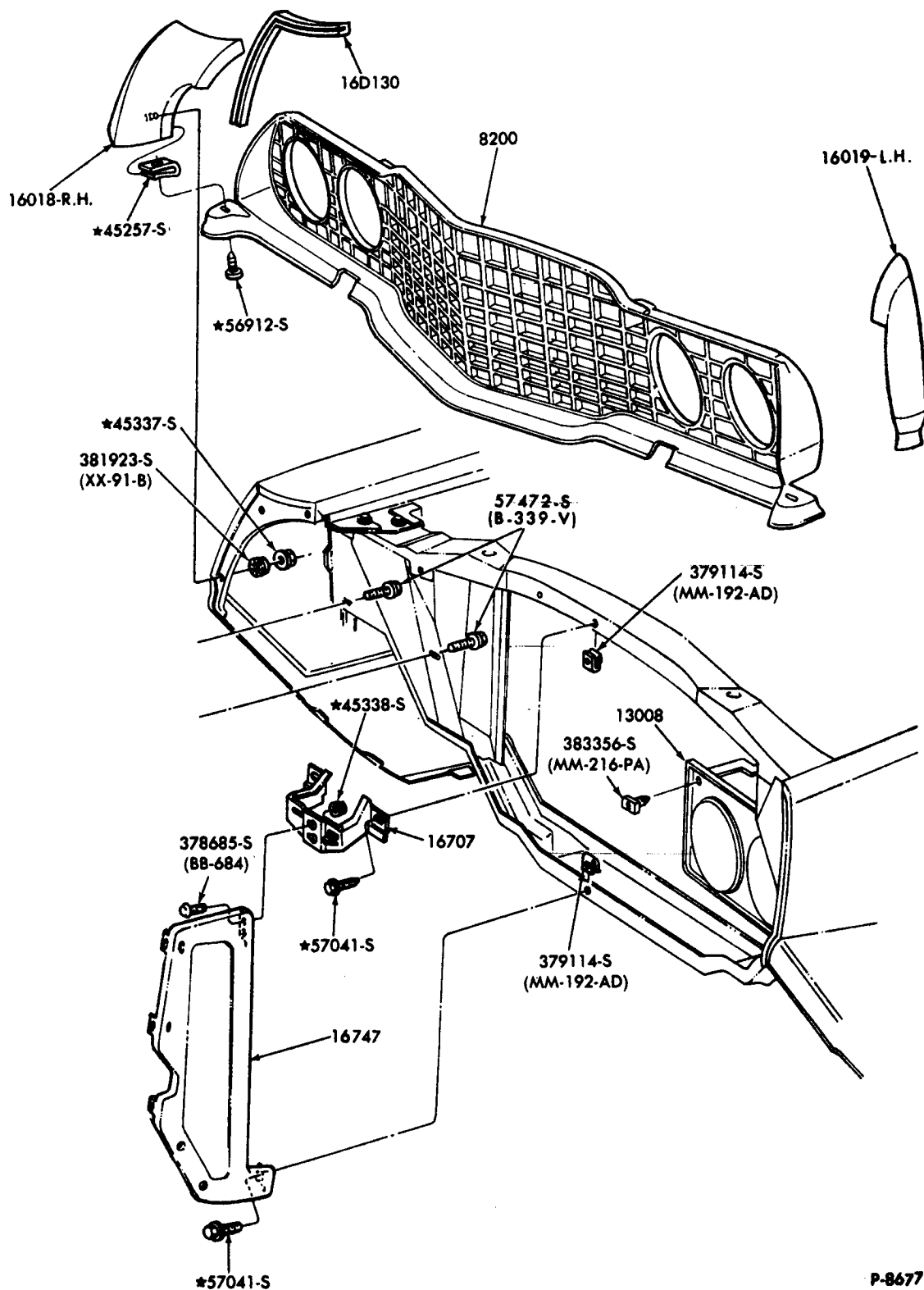
RADIATOR GRILLE and RELATED PARTS 1972 TORINO-BODY TYPES 53B, 65B, 71B
