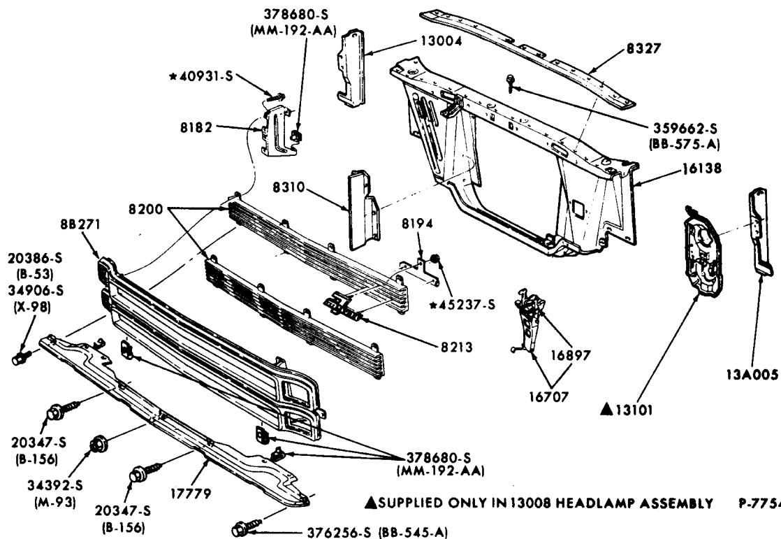
RADIATOR GRILLE and RELATED PARTS 1966 FORD - BODY TYPES 57F, 63C, D, F, 71A, F, 76B, 76D
