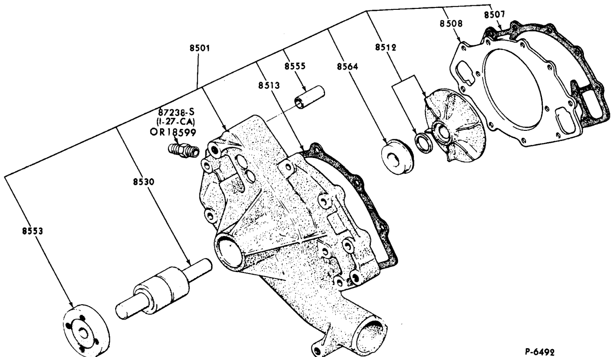
WATER PUMP 1968/72 8 CYLINDER 351C,400,429 and 460
