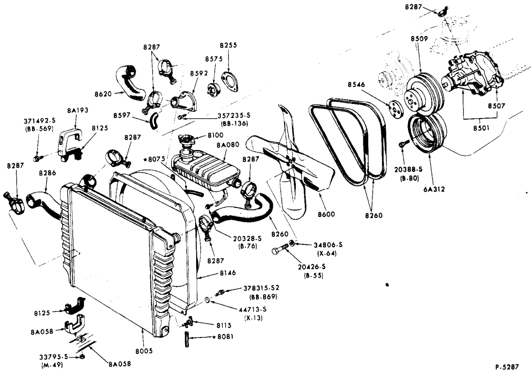
COOLING SYSTEM and RELATED PARTS 1966/72 BRONCO - 8 CYLINDER 289, 302
