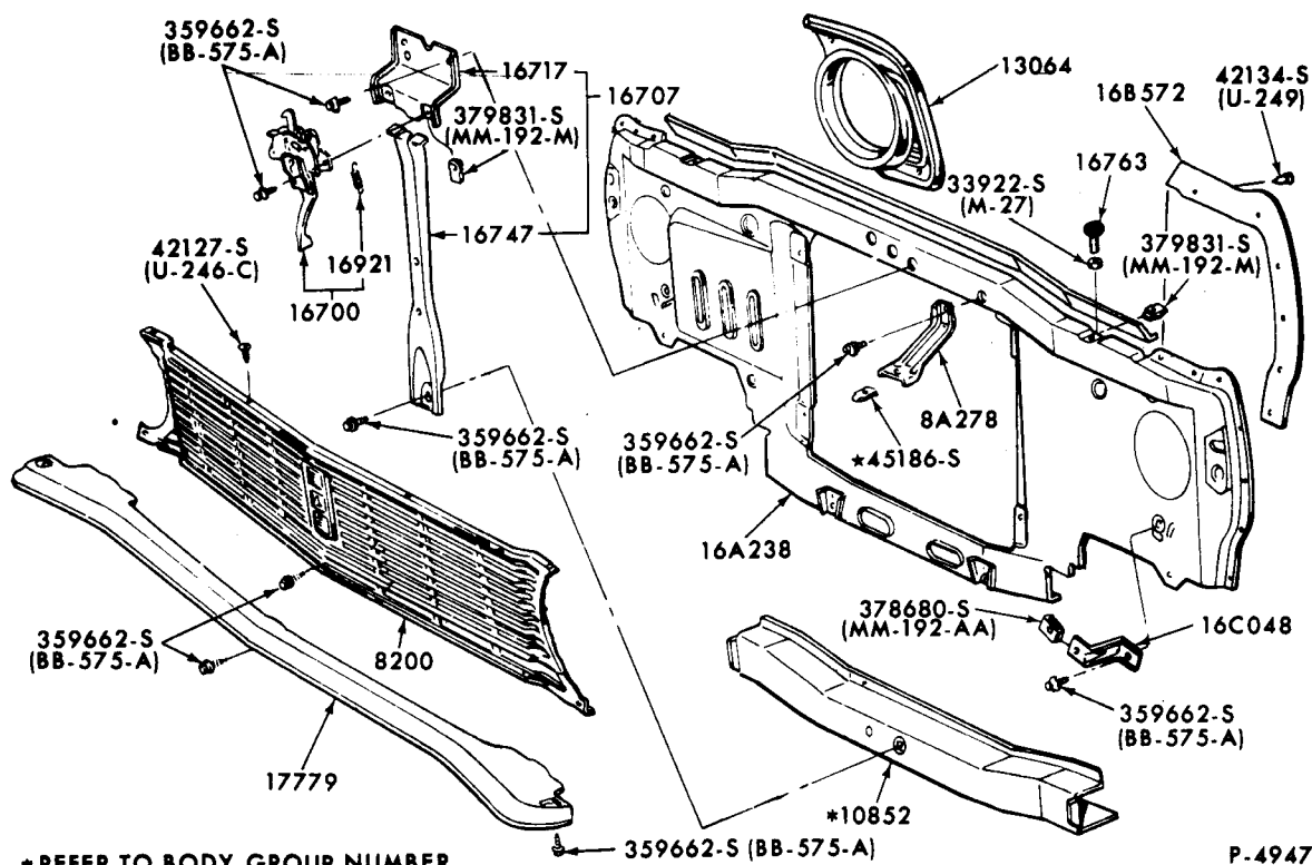
RADIATOR GRILLE and RELATED PARTS 1966/70 FALCON
