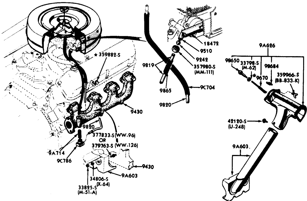
THERMOSTATIC CHOKE CONTROL TUBES and RELATED PARTS 1965/66 FAIRLANE, MUSTANG, FALCON, FORD (8 CYLINDER 260,289 ENGINE - except HIGH PERFORMANCE)
