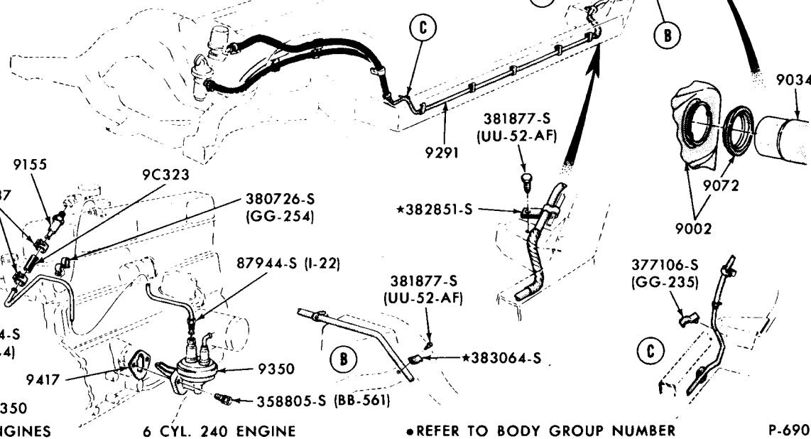
6 CYL. 240 ENGINE
