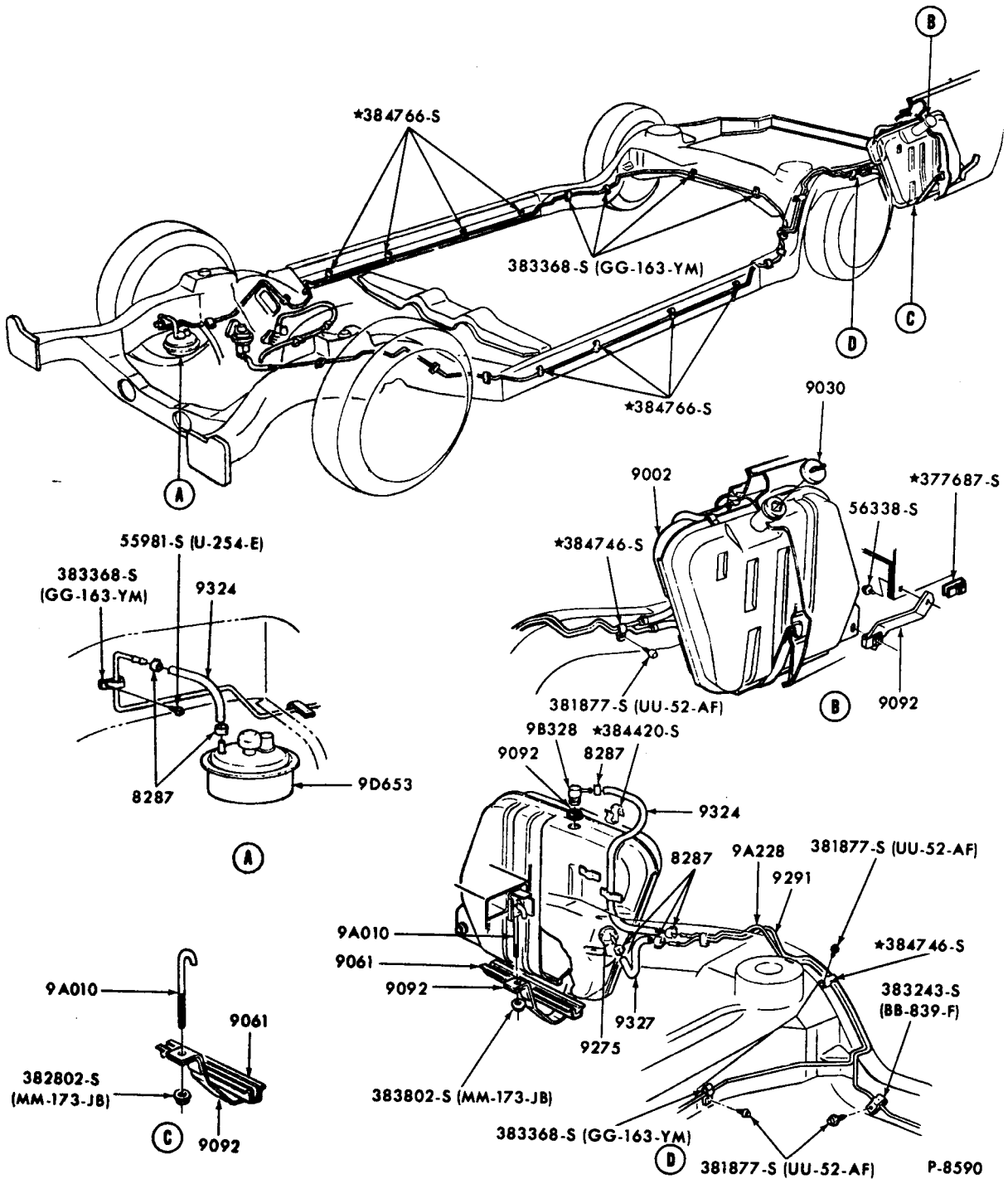
FUEL SYSTEM and RELATED PARTS 1972 TORINO - BODY TYPE 71
