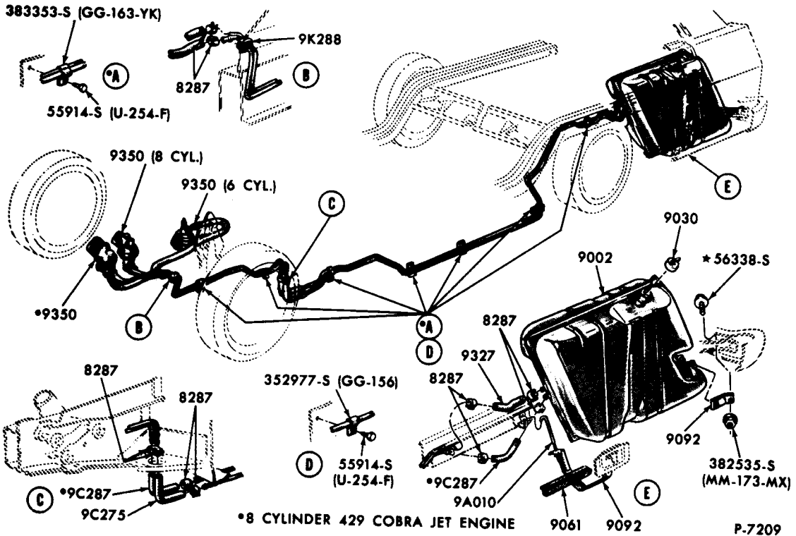
FUEL SYSTEM and RELATED PARTS--(WITHOUT EVAPORATIVE EMISSION CONTROL) 1970 FAIRLANE/TORINO, FALCON - STATION WAGON
