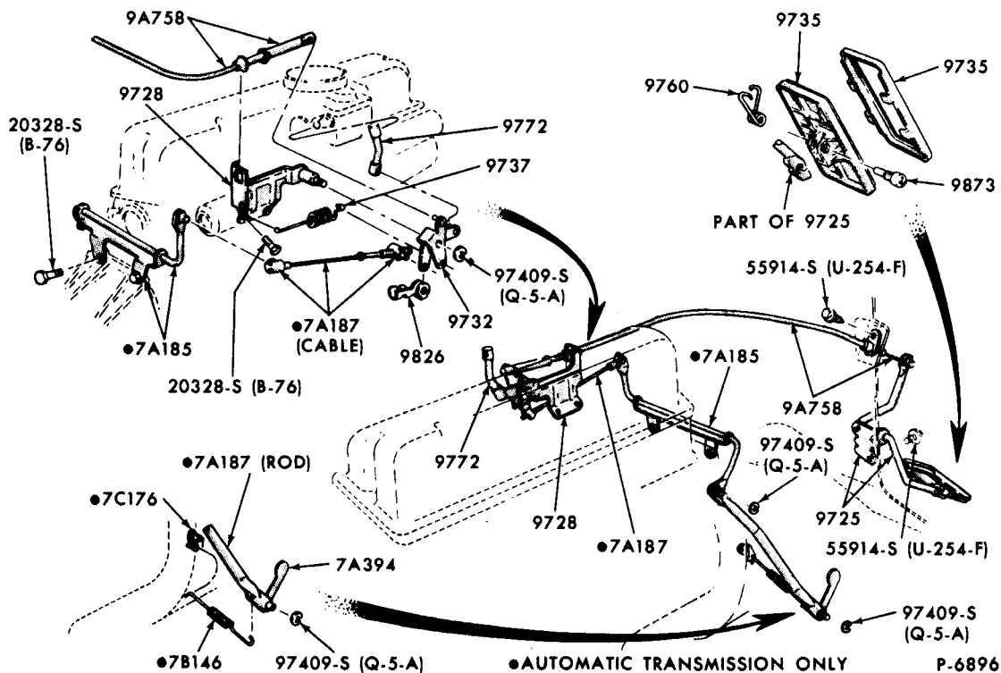
ACCELERATOR LINKAGE 1969/70 MUSTANG (6 CYLINDER 200, 250 ENGINES)
