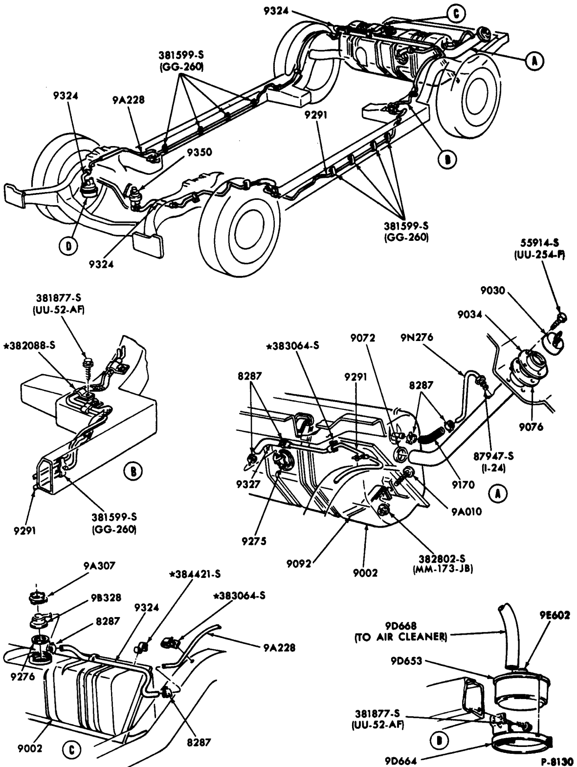
FUEL SYSTEM and RELATED PARTS
