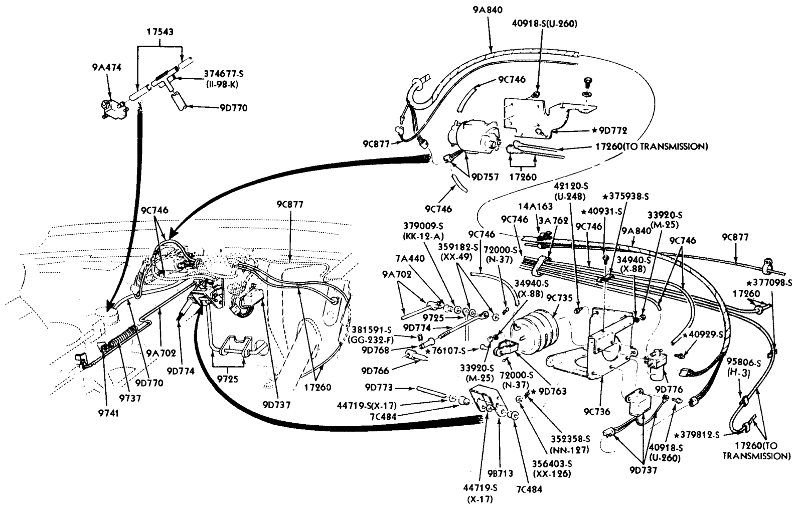
SPEED CONTROL - ENGINE COMPARTMENT 1967 MUSTANG
