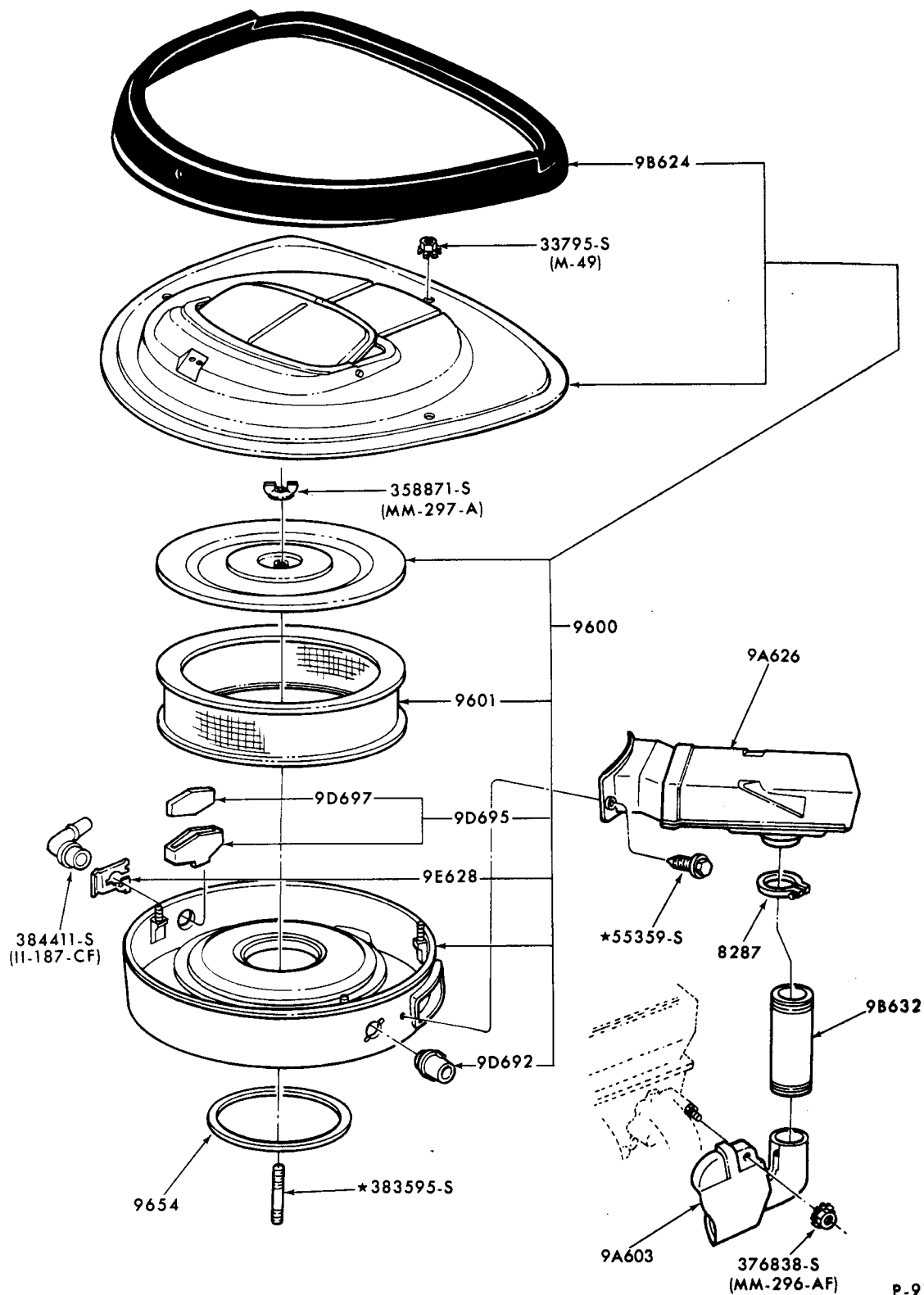
AIR CLEANER - 8 CYLINDER - RAM AIR 1972 TORINO (429 ENGINE)
