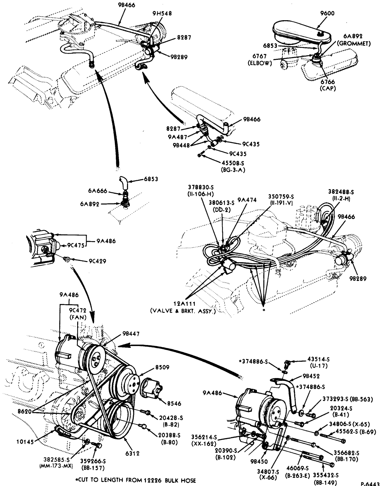
TERMACTOR EMISSION CONTROL SYSTEM 1968 BRONCO ( 8 CYLINDER 289 ENGINE )
