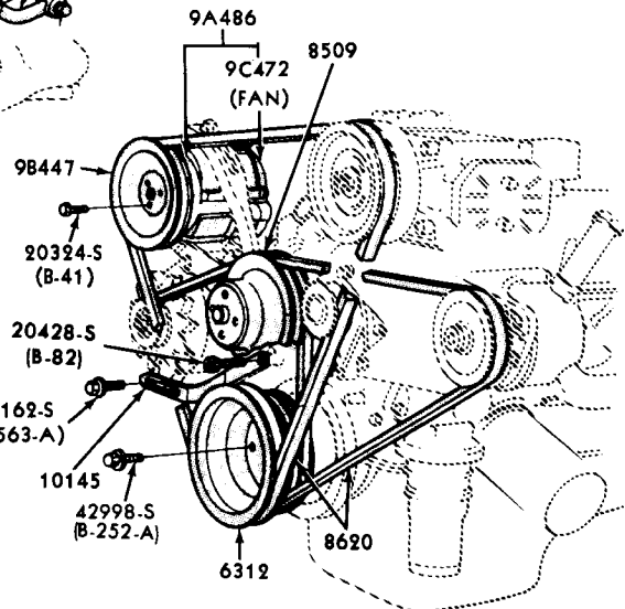
THERMACTOR WITH AIR CONDITIONING AND AUTOMATIC TRANSMISSION
