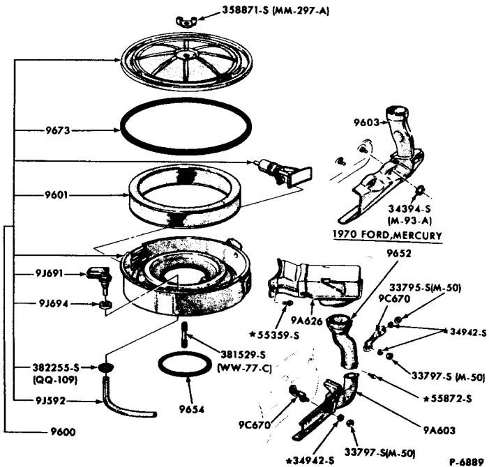
AIR CLEANER - 8 CYLINDER - except RAM AIR 1968/70 FAIRLANE/TORINO, MUSTANG (428 ENGINE) 1970 FORD (428 PC ENGINE)
