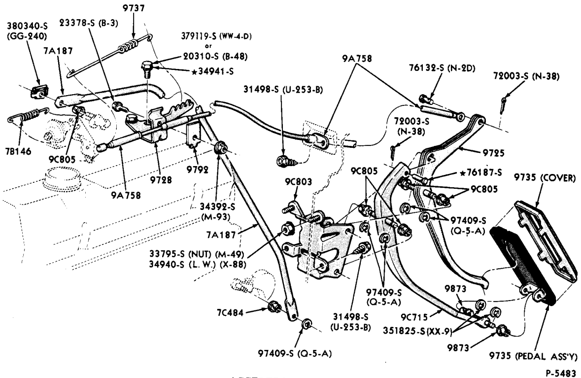
1967 THUNDERBIRD (8 CYLINDER 390, 428 ENGINES)
