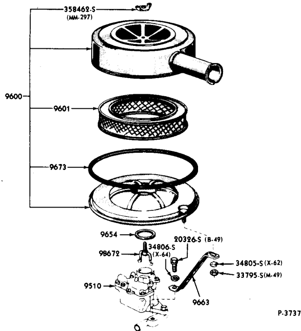
AIR CLEANER - 6 CYLINDER 1965/67 FAIRLANE, FALCON and MUSTANG 1966 BRONCO
