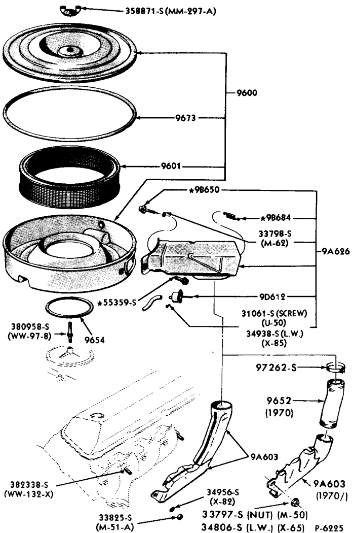
AIR CLEANER - 8 CYLINDER 1968/70 THUNDERBIRD, FAIRLANE/TORINO (429 ENGINE) 1970/71 FORD (429-2V, 4V ENGINES)
