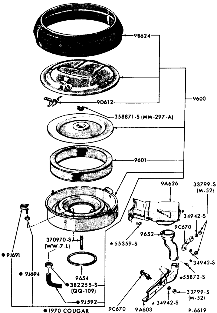
AIR CLEANER - 8 CYLINDER - RAW AIR 1969 FAIRLANE/TORINO (428 COBRA JET ENGINE) 1969/70 MUSTANG (428 COBRA JET ENGINE)
