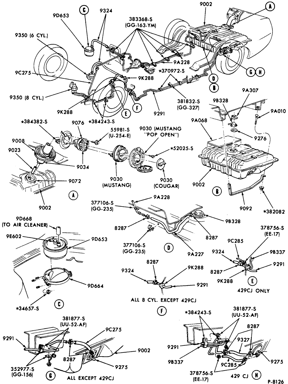
FUEL SYSTEM and RELATED PARTS 1971/72 MUSTANG
