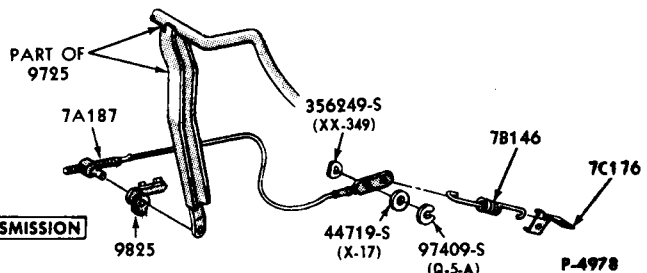
ACCELERATOR LINKAGE 1966/69 FAIRLANE/TORINO (6 CYLINDER) 1966/70 FALCON (6 CYLINDER)
