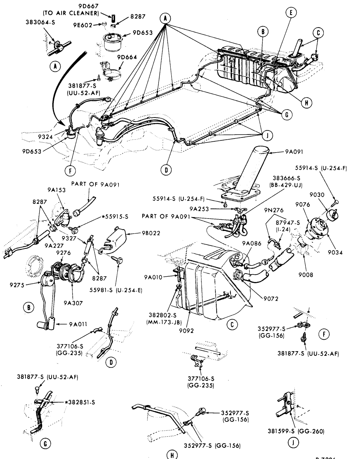
FUEL SYSTEM and RELATED PARTS--(WITH EVAPORATIVE EMISSION CONTROL) 1970 FORD - EXCEPT STATION WAGON
