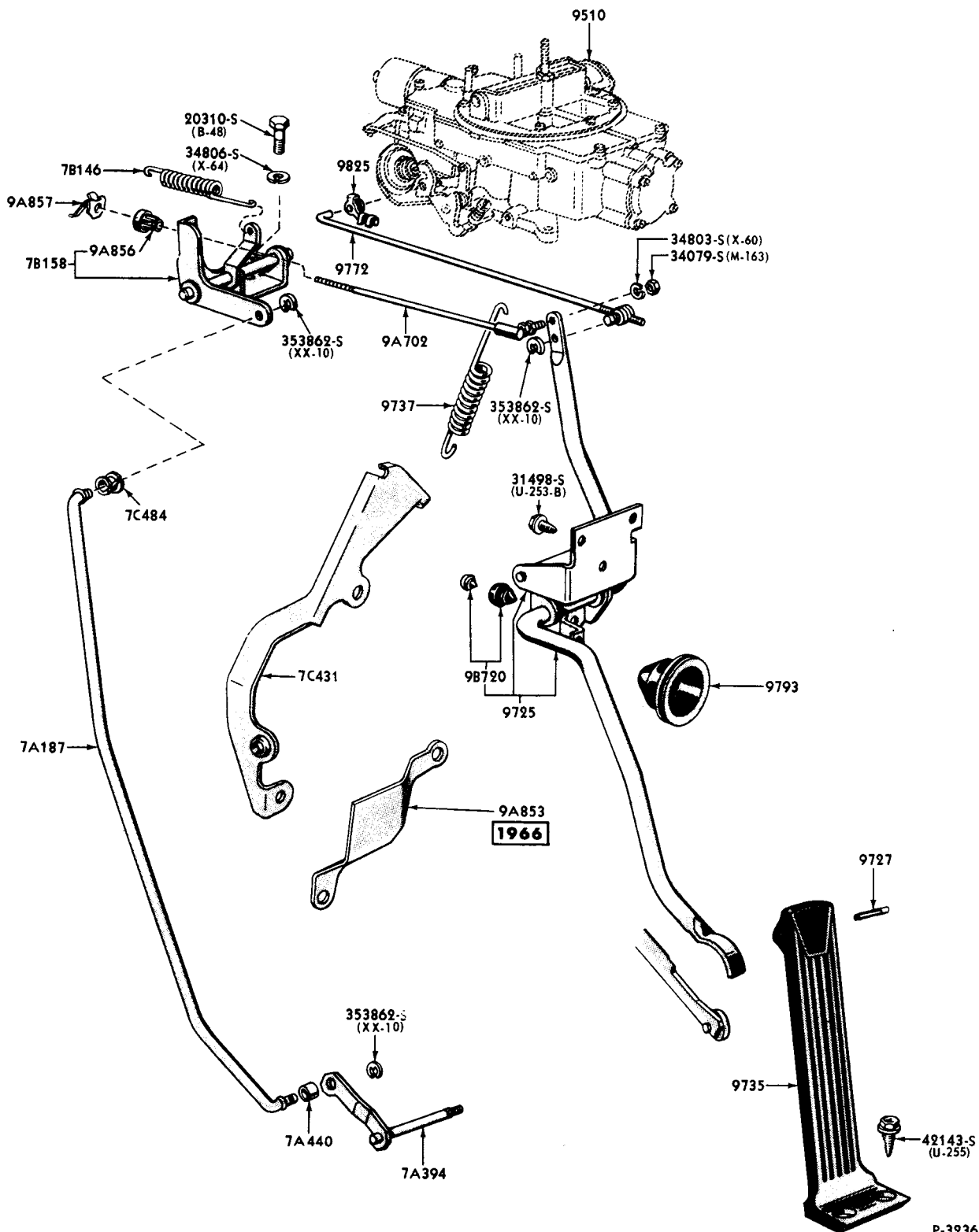
ACCELERATOR LINKAGE 1965/66 THUNDERBIRD (8 CYLINDER 390, 428 ENGINES)
