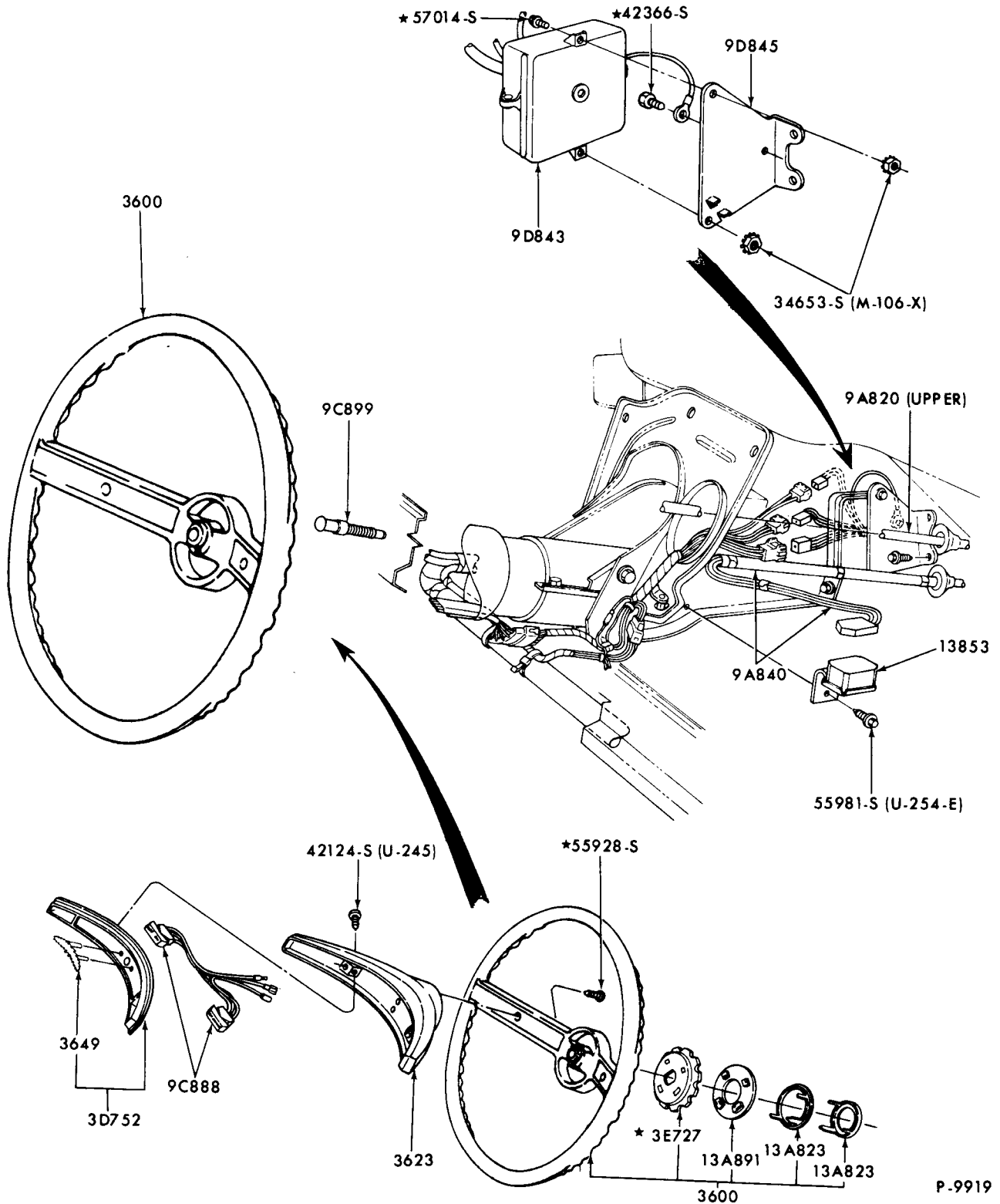
SPEED CONTROL - PASSENGER COMPARTMENT 1972 THUNDERBIRD
