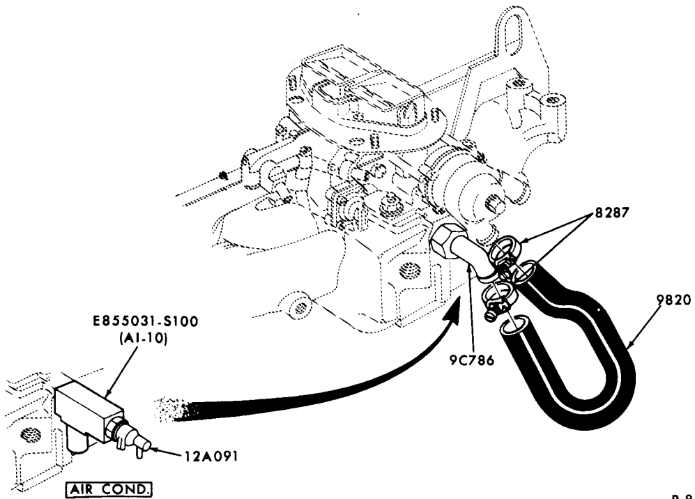
THERMOSTATIC CHOKE CONTROL TUBES and RELATED PARTS 1971/72 PINTO (122 2000 cc ENGINE)
