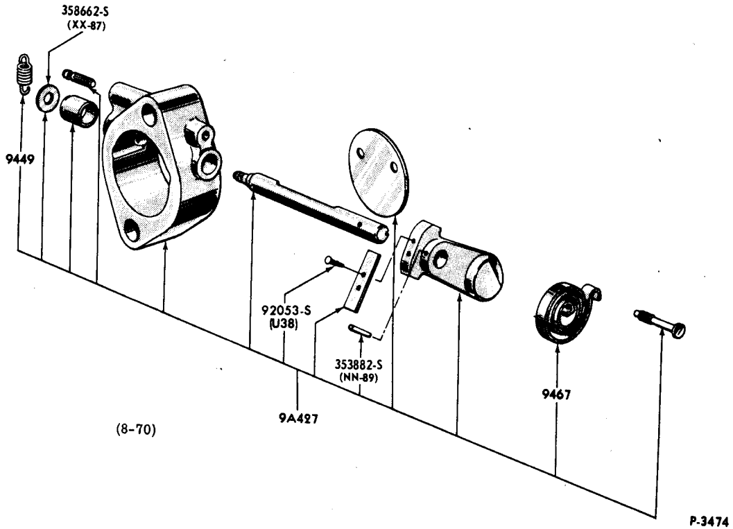
VALVE ASSY. (EXHAUST THERMOSTAT CONTROL) - 8 CYLINDER (ARM COUNTERWEIGHT) - TYPICAL
