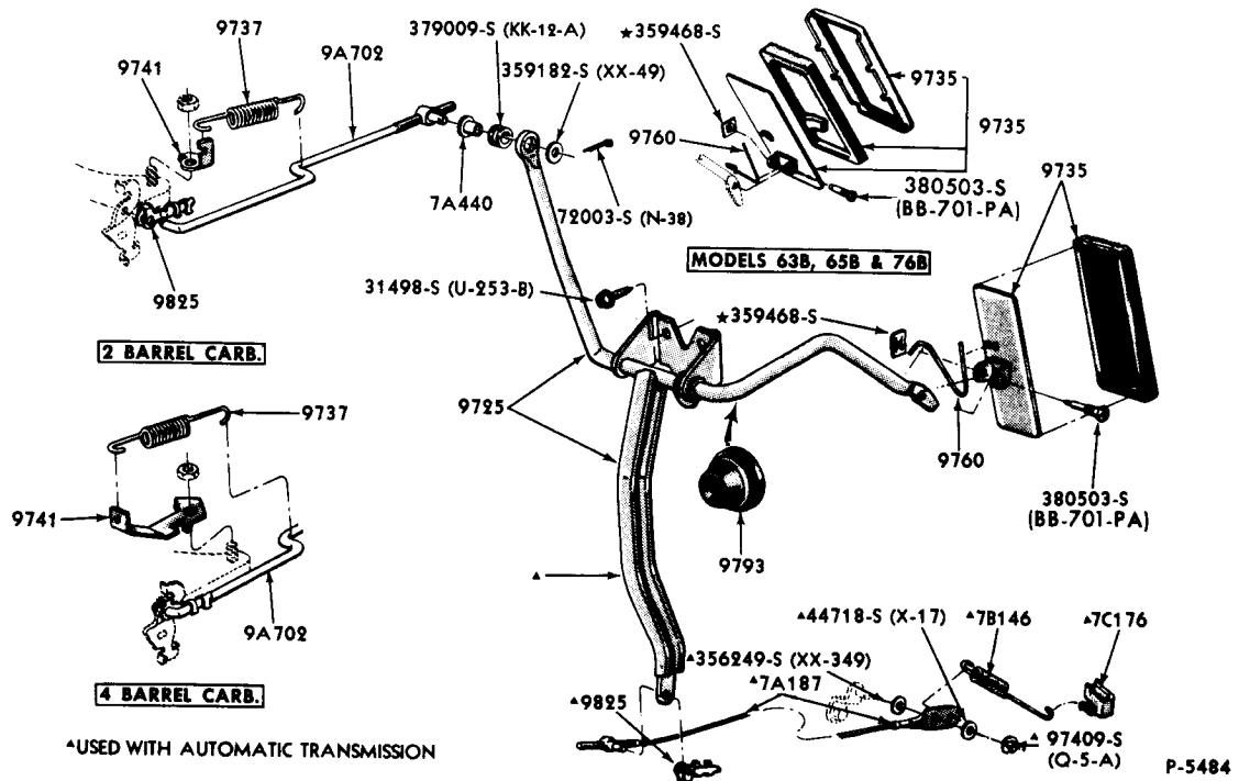
ACCELERATOR LINKAGE 1967/68 MUSTANG (8 CYLINDER 289,302,390,427,428 ENGINES)
