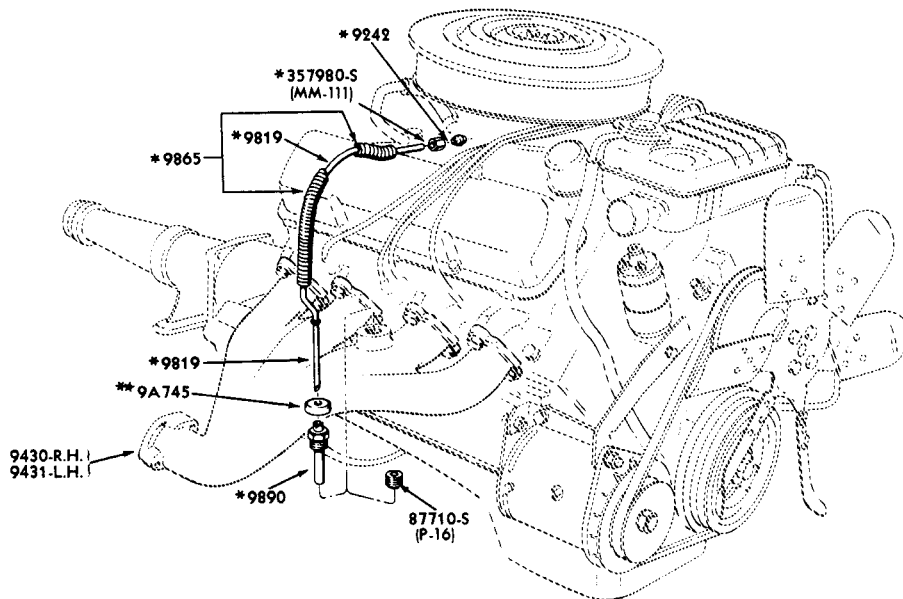
*TYPICAL INSTALLATION FOR 4 BARREL CARBURETOR.
