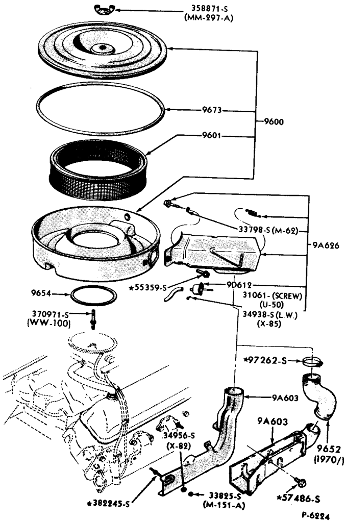
AIR CLEANER - 8 CYLINDER 1968/71 FALCON, FORD, MAVERICK (289, 302, 351 ENGINES) 1968/71 FAIRLANE/TORINO, MUSTANG (289, 302 ENGINES) 1969 FAIRLANE, MUSTANG (351 ENGINE)
