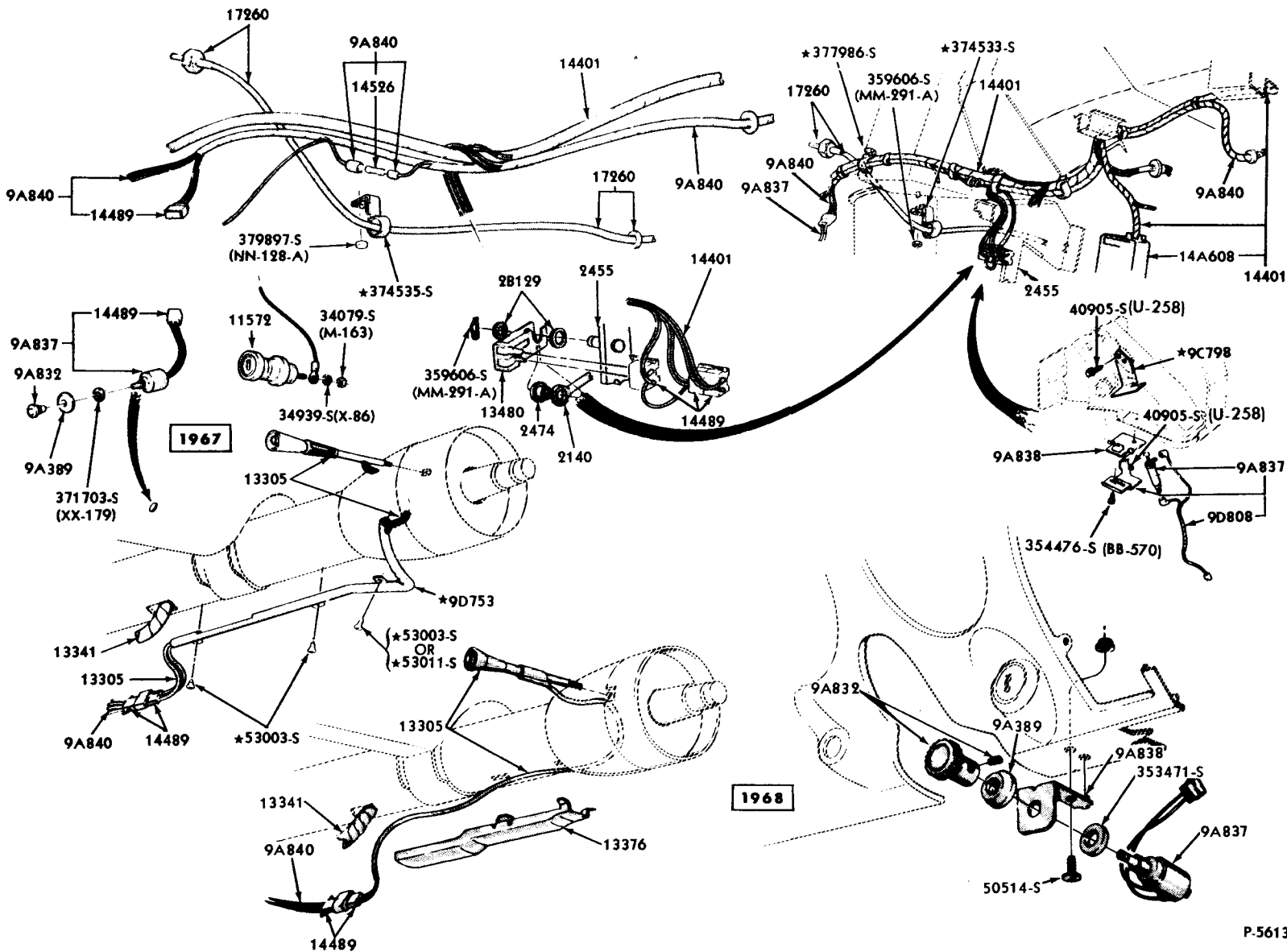
SPEED CONTROL - PASSENGER COMPARTMENT
