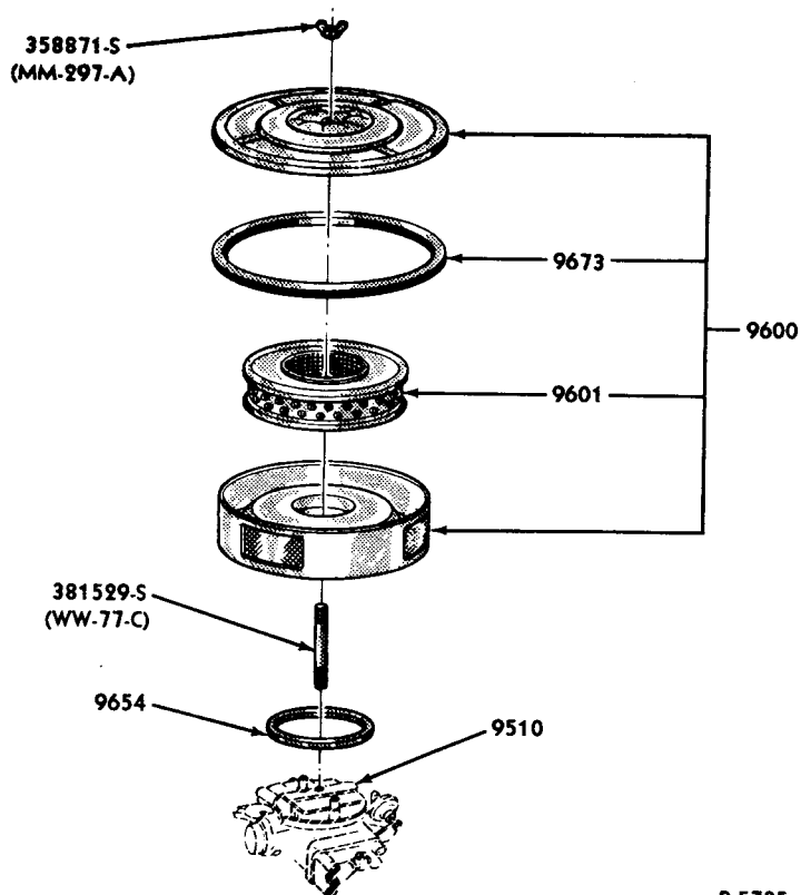
AIR CLEANER - 8 CYLINDER 1966/67 FAIRLANE, MUSTANG (390-4V, GT and GTA ENGINES)
