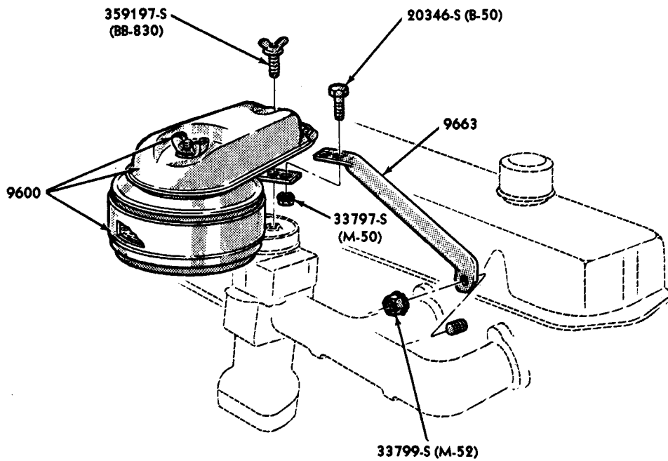
AIR CLEANER - 6 CYLINDER 1966/67 FORD (240 ENGINE except TAXI and POLICE)
