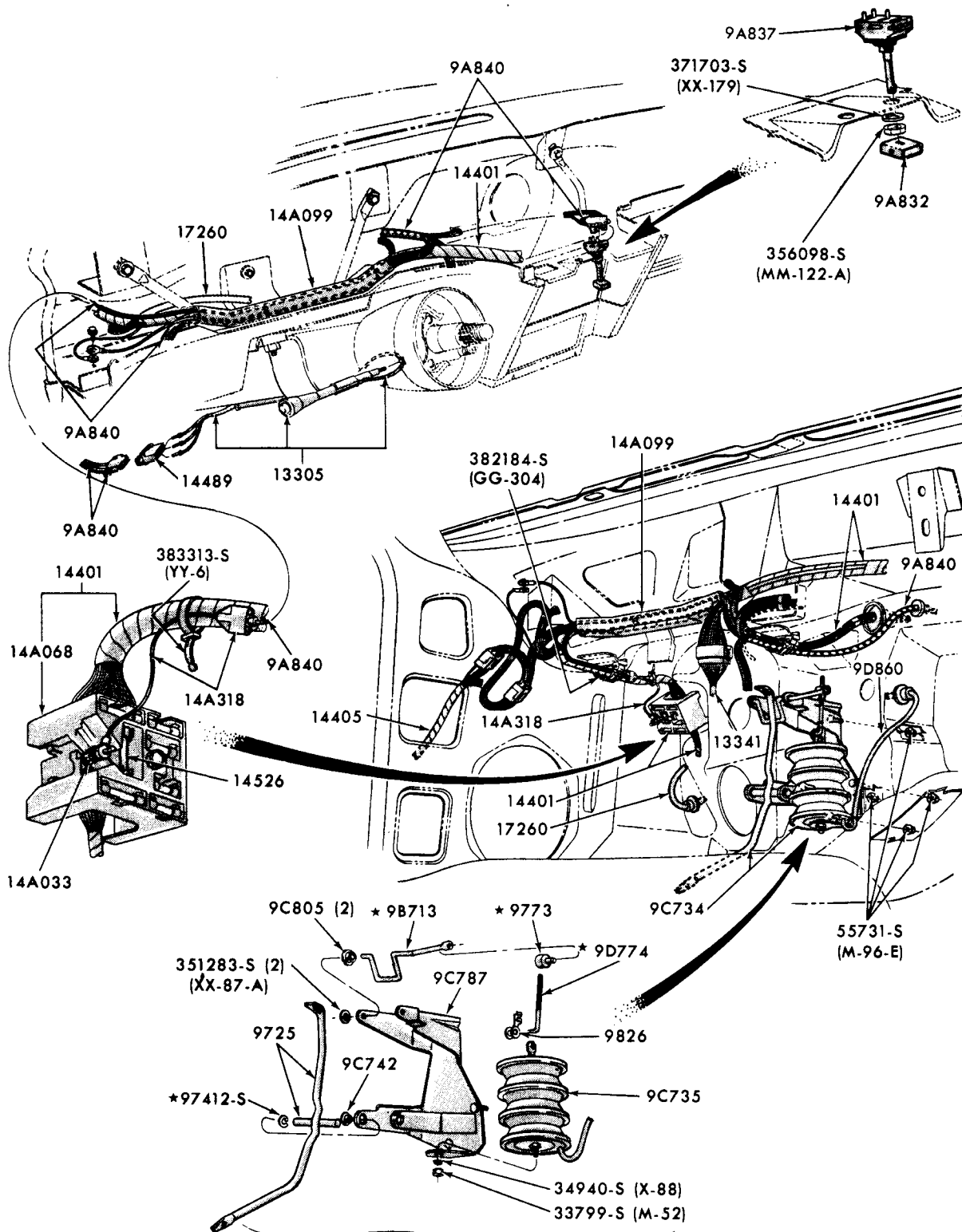
9C734 ASSEMBLY
