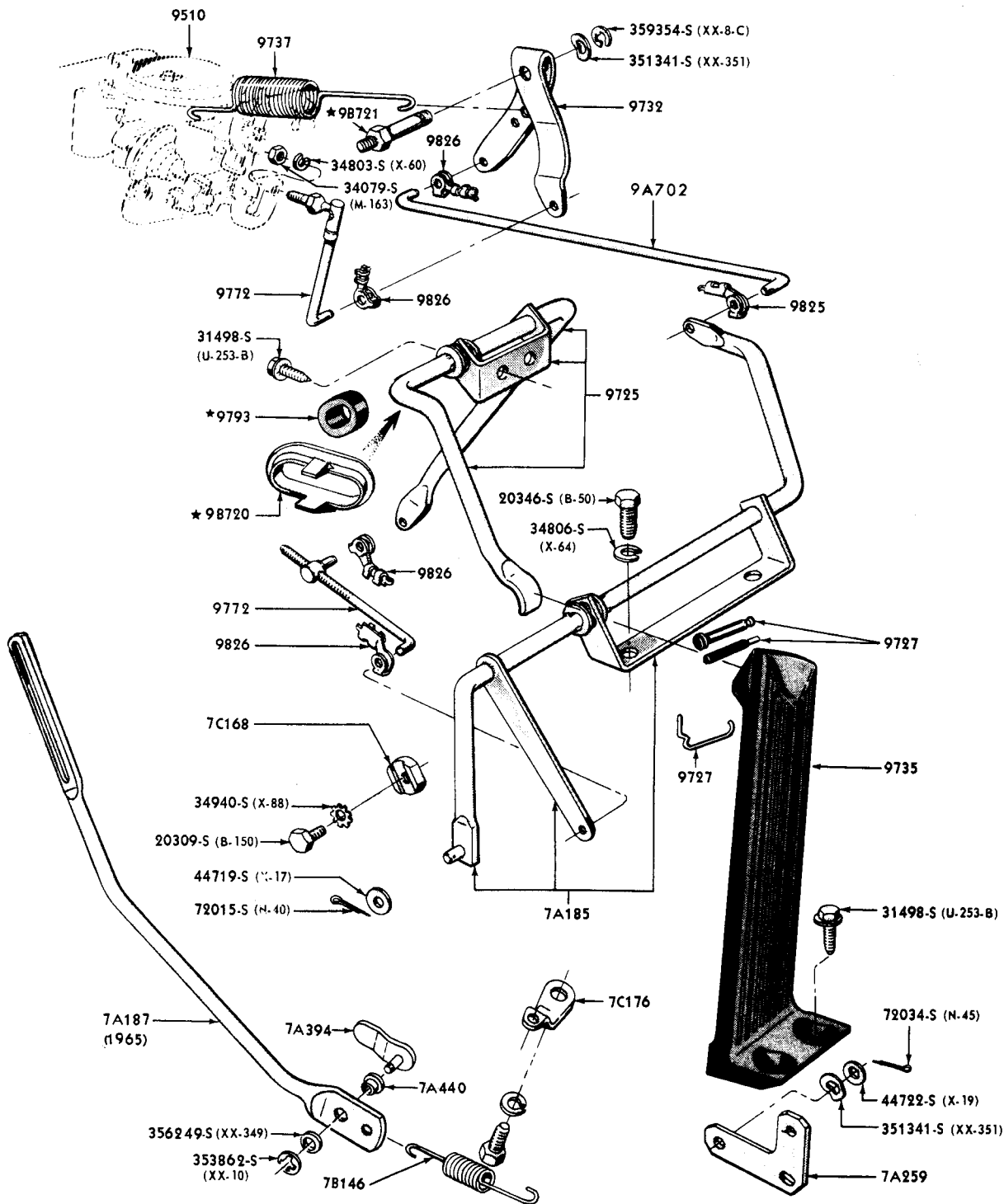
ACCELERATOR LINKAGE 1965 FALCON (6 CYLINDER) AUTOMATIC TRANSMISSION
