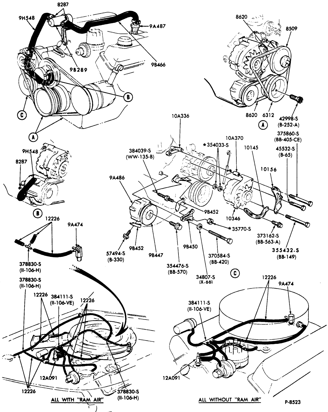
THERMACTOR EMISSION CONTROL SYSTEM 1969/72 MUSTANG 8 CYLINDER "BOSS 302" ENGINE
