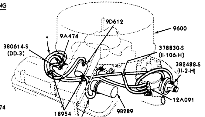
THERMACTOR WITH AIR CONDITIONING AND AUTOMATIC TRANSMISSION
