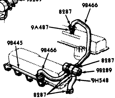
FORD WITHOUT AIR COND. AND WITH STD. TRANS.
