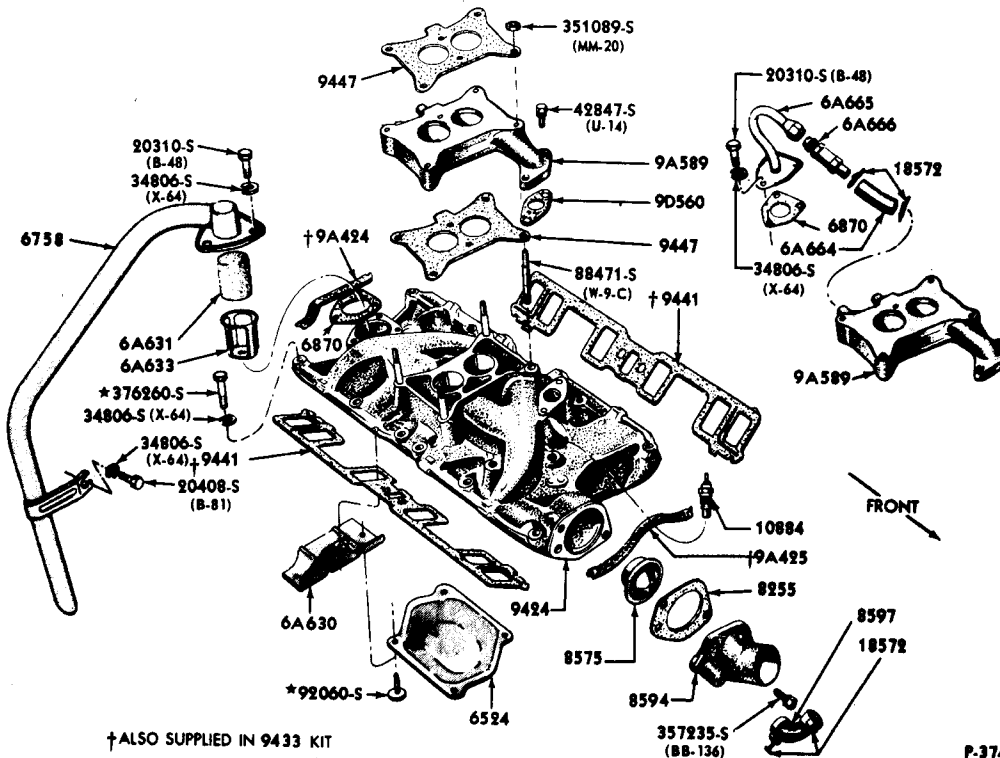
MANIFOLD and RELATED PARTS - INTAKE
