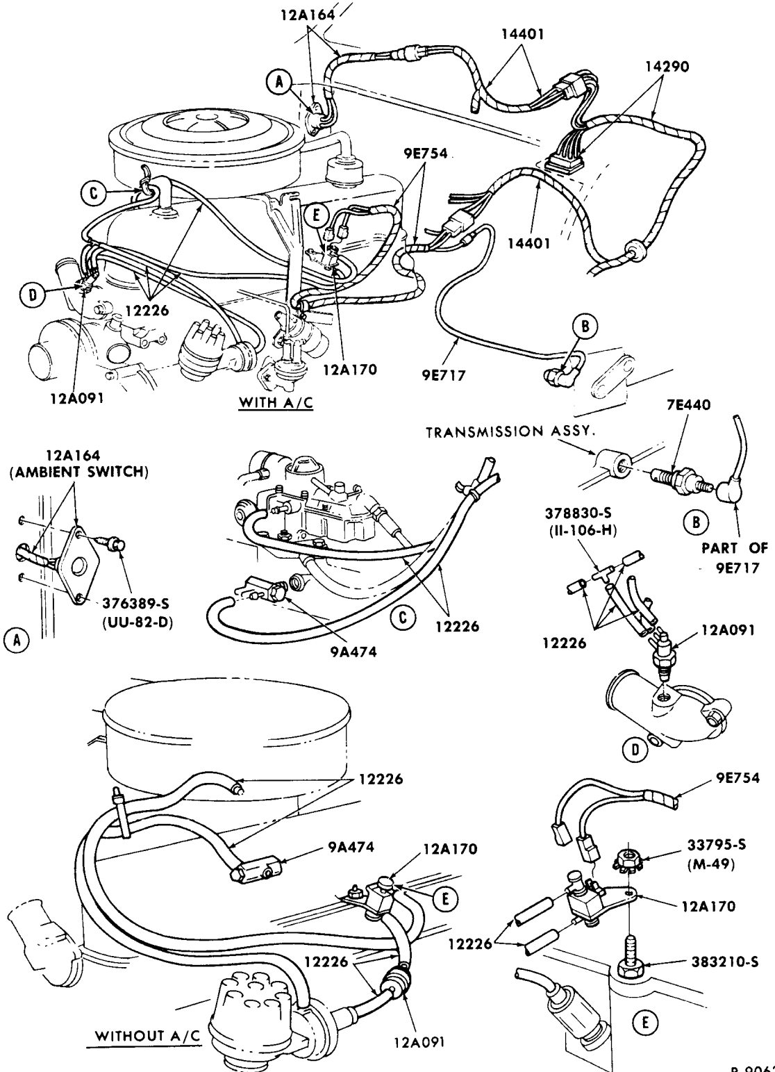
TRANSMISSION REGULATED SPARK CONTROL SYSTEM (T.R.S.)-6 CYL. 250 I.D. ENGINE 1972 MUSTANG
