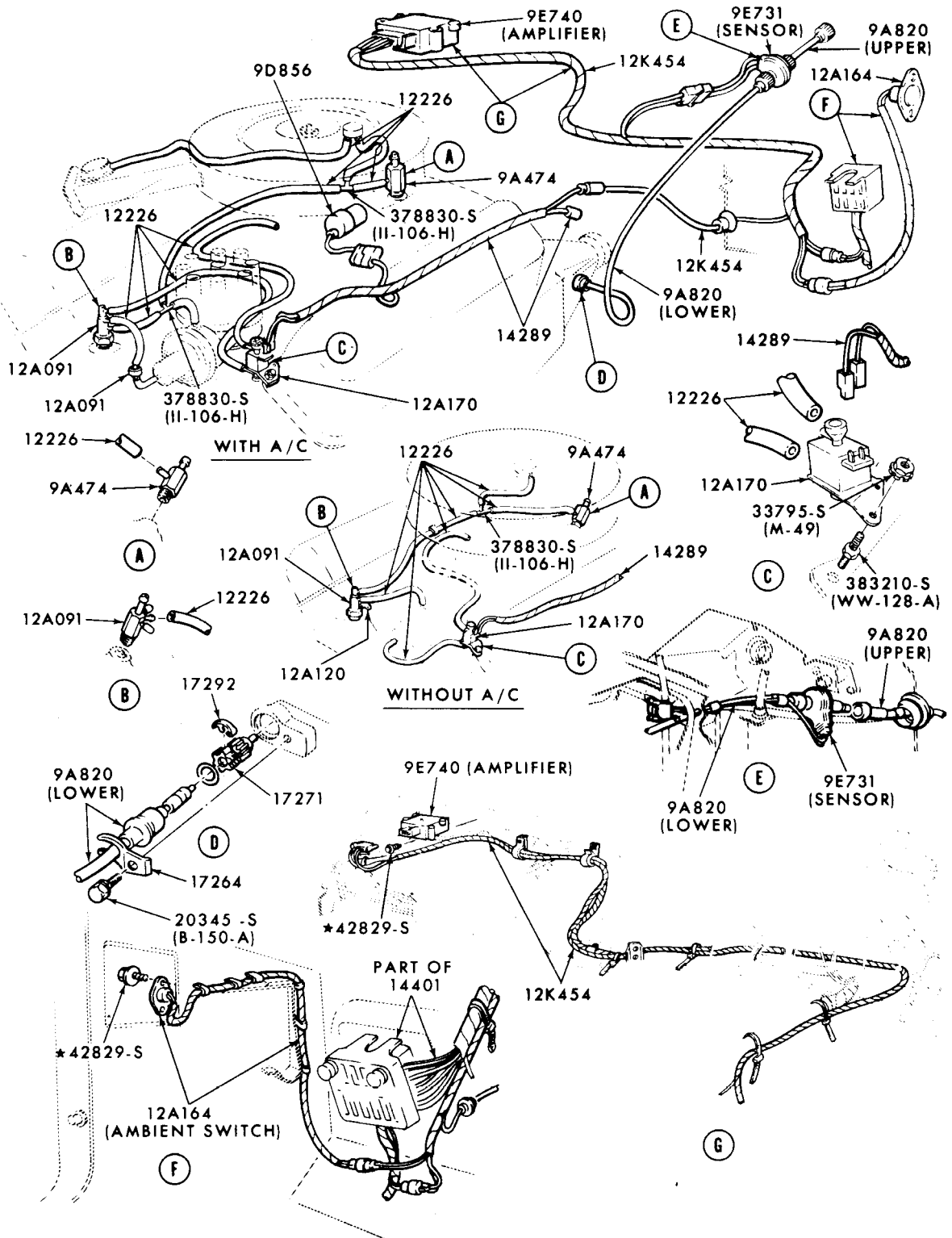
ELECTRONIC SPARK CONTROL SYSTEM (E.S.C.)-8 CYL. 302-2V C.I.D. ENGINE 1972 TORINO
