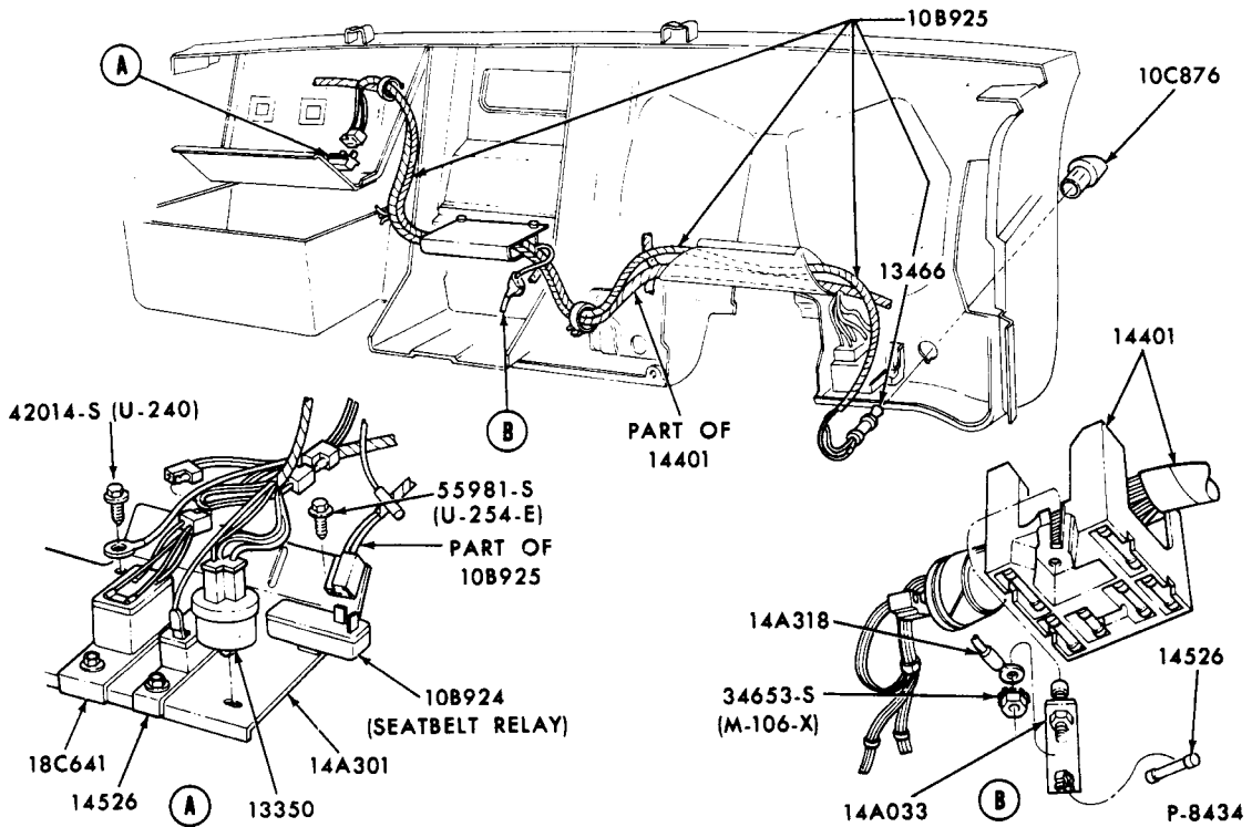
SEAT BELT WARNING LAMP INSTALLATION 1971/72 MUSTANG
