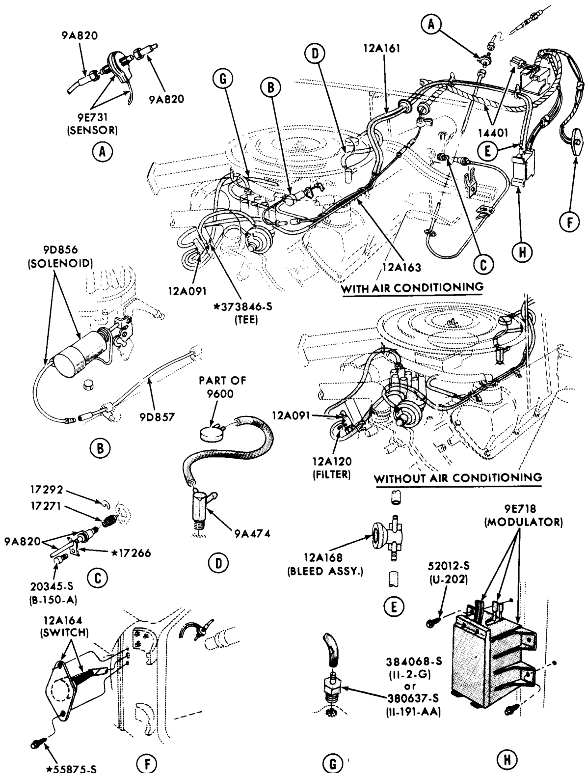
DISTRIBUTOR MODULATOR - 8 CYL. 351-4V ENGINE WITHOUT RAM AIR 1970 MUSTANG
