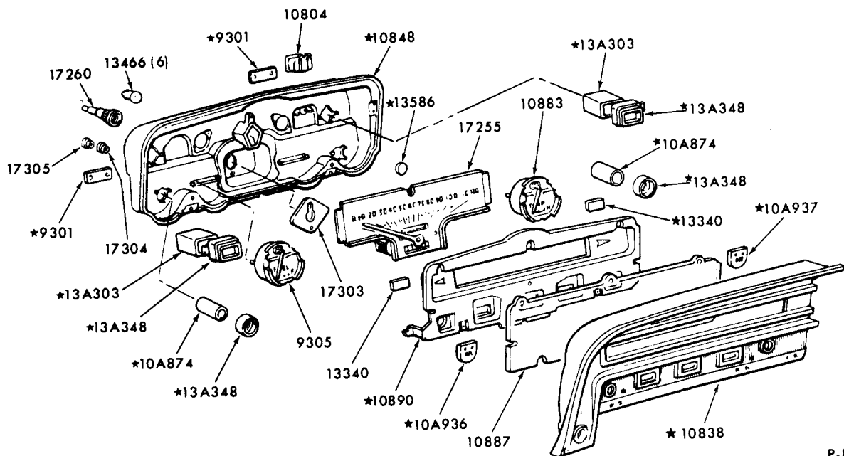
INSTRUMENT CLUSTER and RELATED PARTS 1965 FAIRLANE
