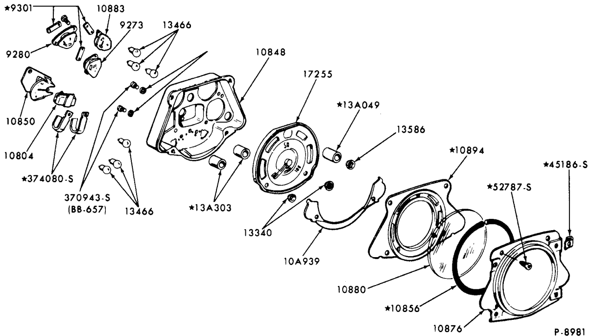
INSTRUMENT CLUSTER and RELATED PARTS 1966/67 BRONCO
