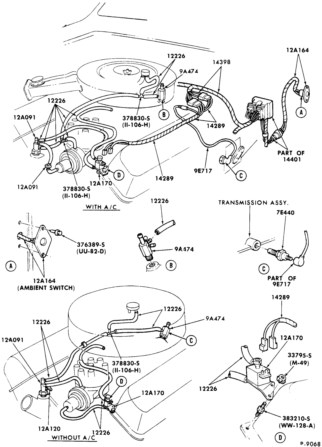
TRANSMISSION REGULATED SPARK CONTROL SYSTEM (T.R.S.)-8 CYL. 302-2V ENGINE 1972 TORINO
