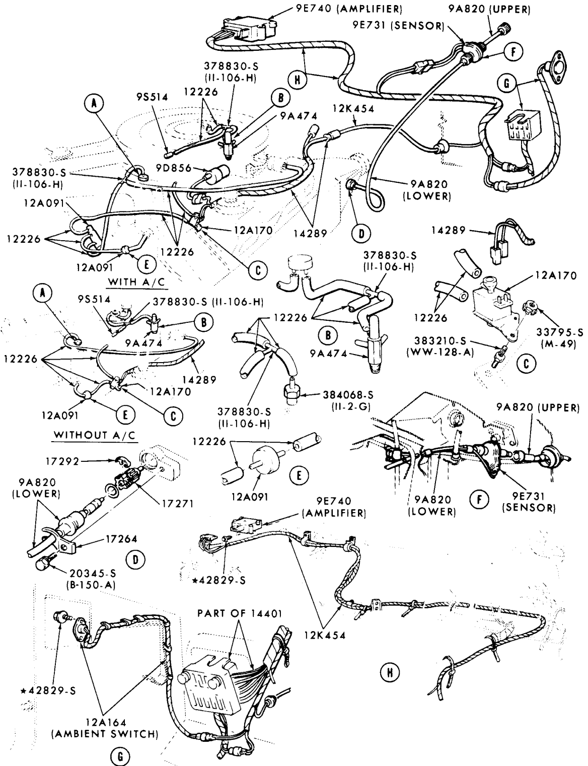
ELECTRONIC SPARK CONTROL SYSTEM (E.S.C.)-8 CYL. 351-4V CJ ENGINE 1972 TORINO - WITHOUT RAM AIR HOOD
