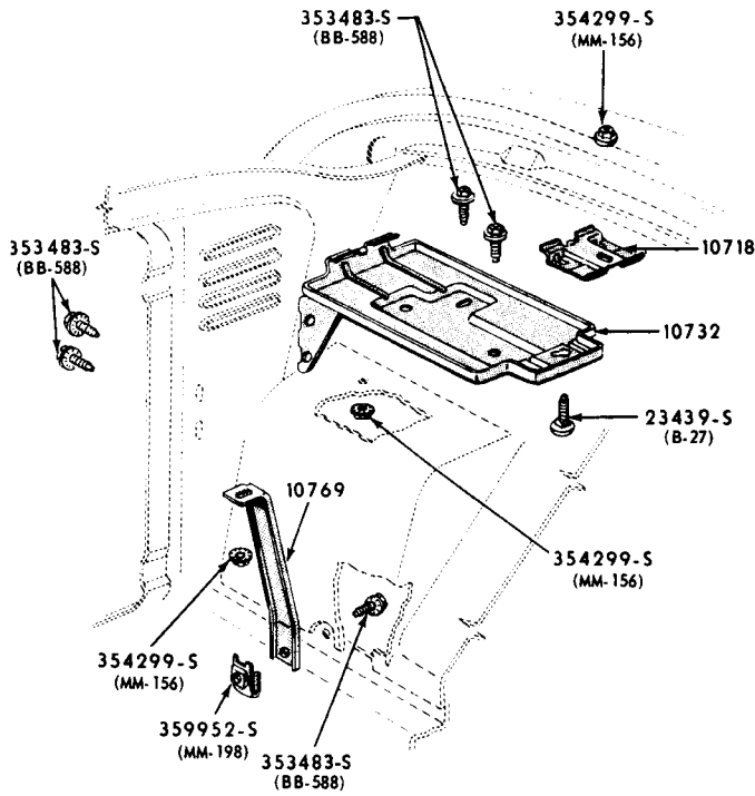
BATTERY CARRIER and RELATED PARTS 1965 FALCON
