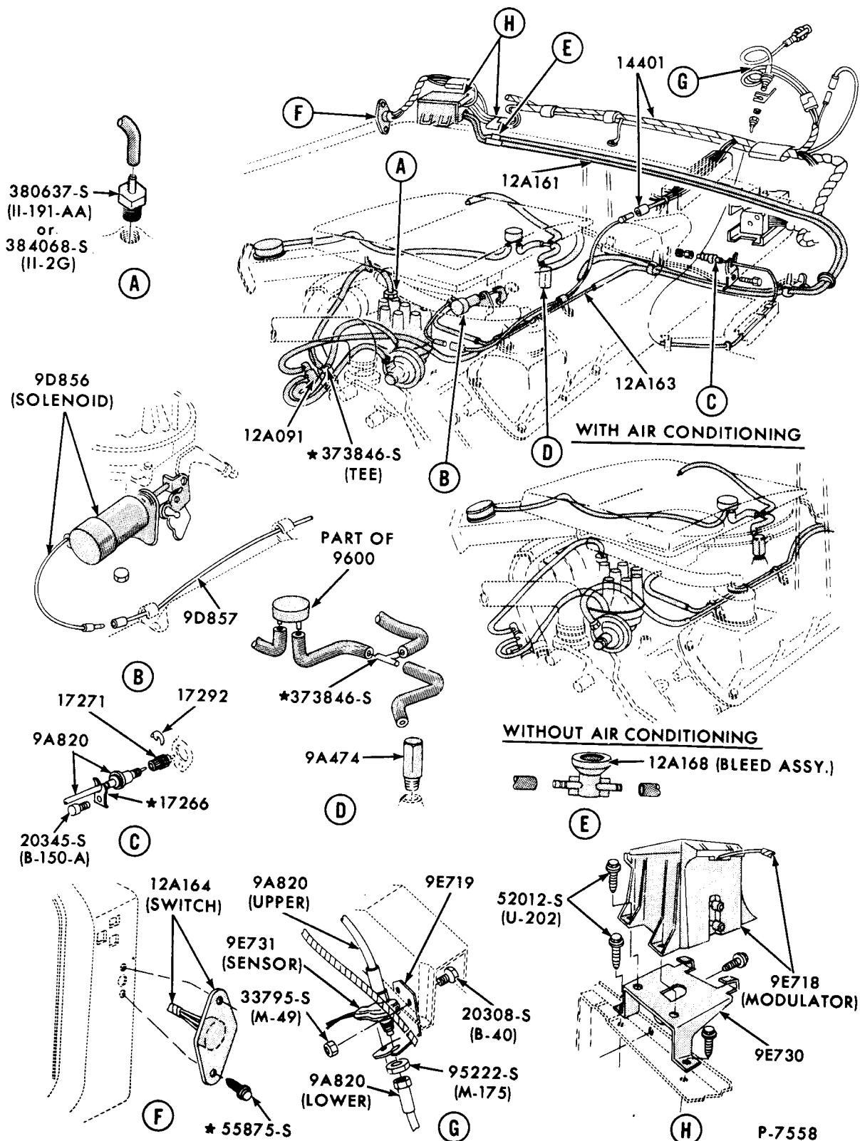
DISTRIBUTOR MODULATOR - 8 CYL. 351-4V C.I.D. ENGINE WITH RAM AIR 1970 FAIRLANE/TORINO
