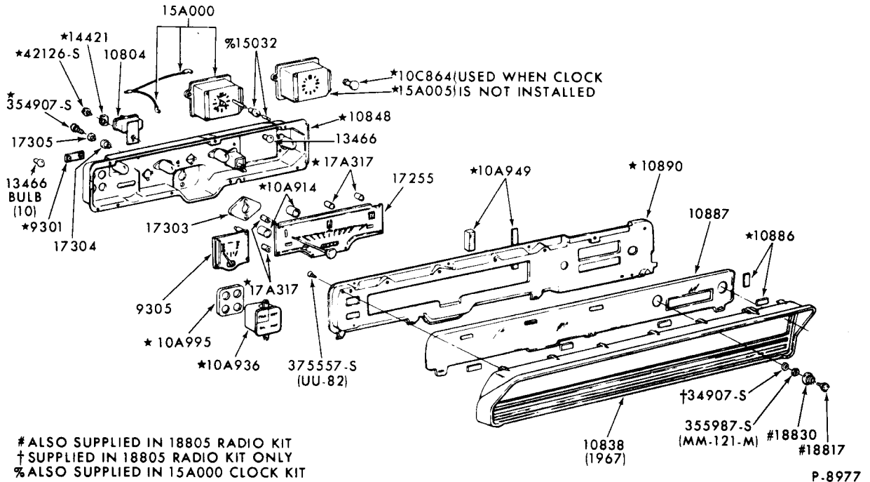
INSTRUMENT CLUSTER and RELATED PARTS 1966/67 FAIRLANE
