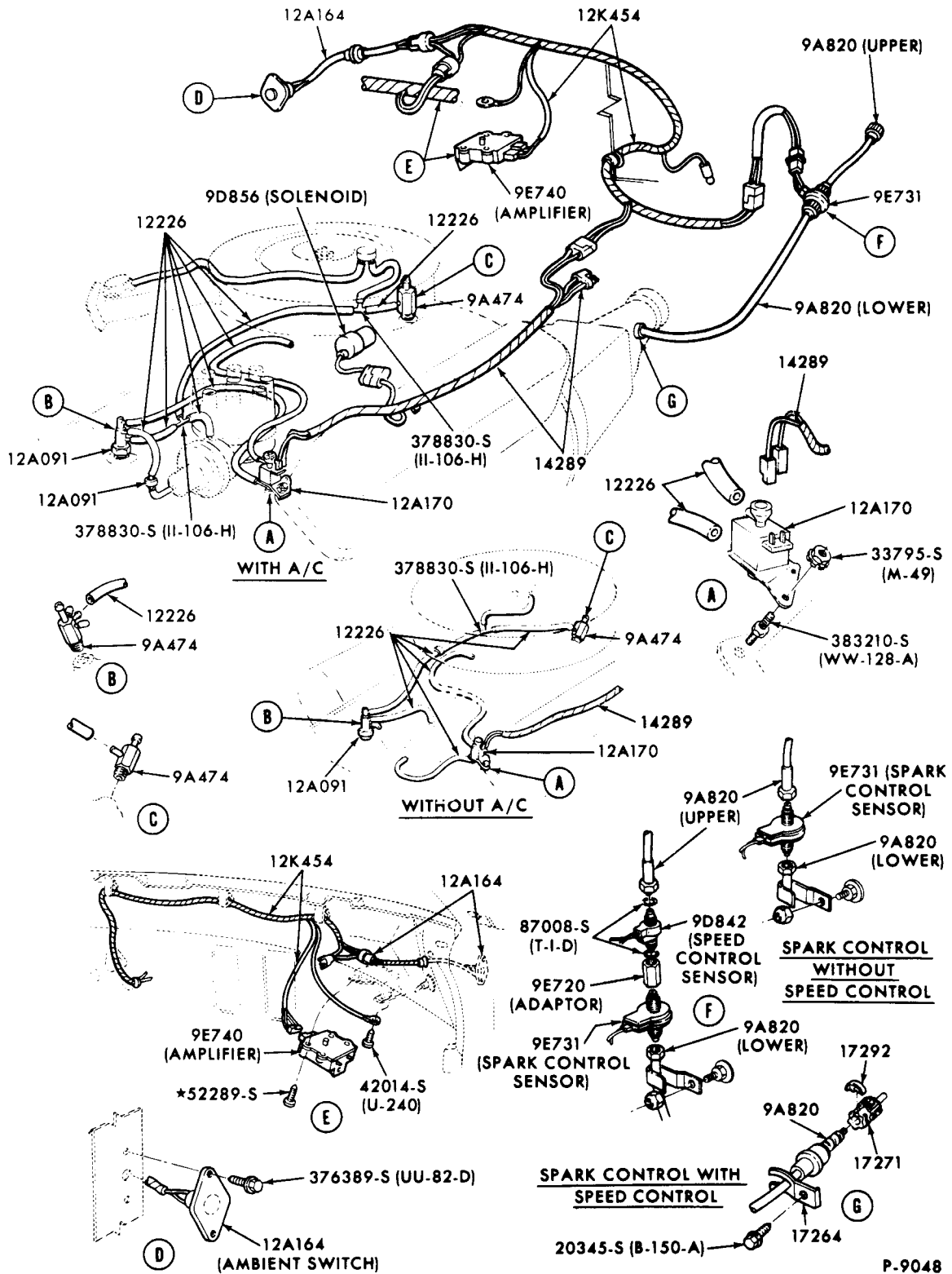
ELECTRONIC SPARK CONTROL SYSTEM (E.S.C.)-8 CYL. 302-2V C.I.D. ENGINE 1972 FORD
