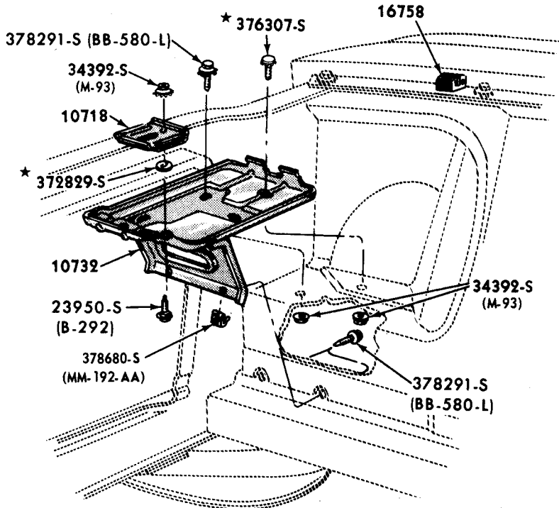
BATTERY CARRIER and RELATED PARTS 1965/68 MUSTANG
