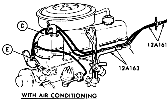
DISTRIBUTOR MODULATOR-6 CYLINDER 250 C.I.D. ENGINE 1971 MUSTANG
