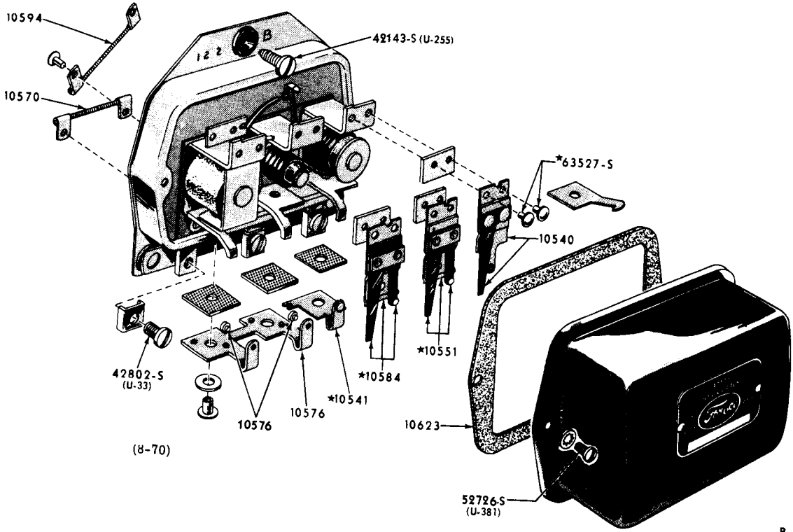
VOLTAGE REGULATOR - TYPICAL (GENERATOR) 1965
