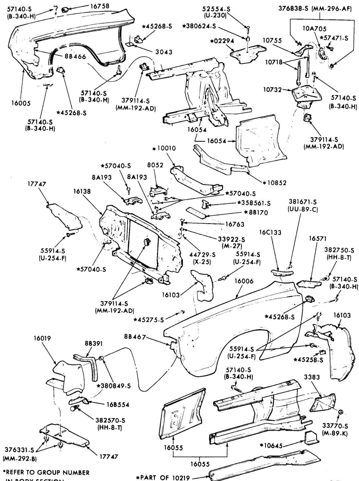
FENDERS, APRONS and RELATED PARTS 1970/71 FAIRLANE/TORINO
