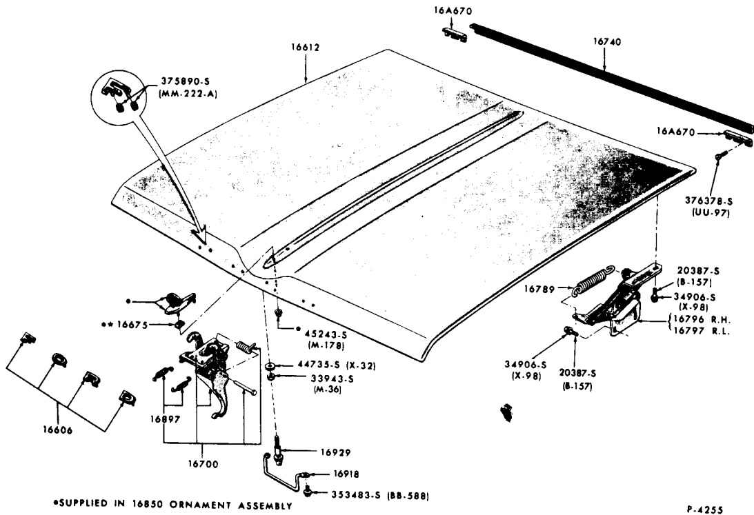
HOOD and RELATED PARTS 1965 FALCON
