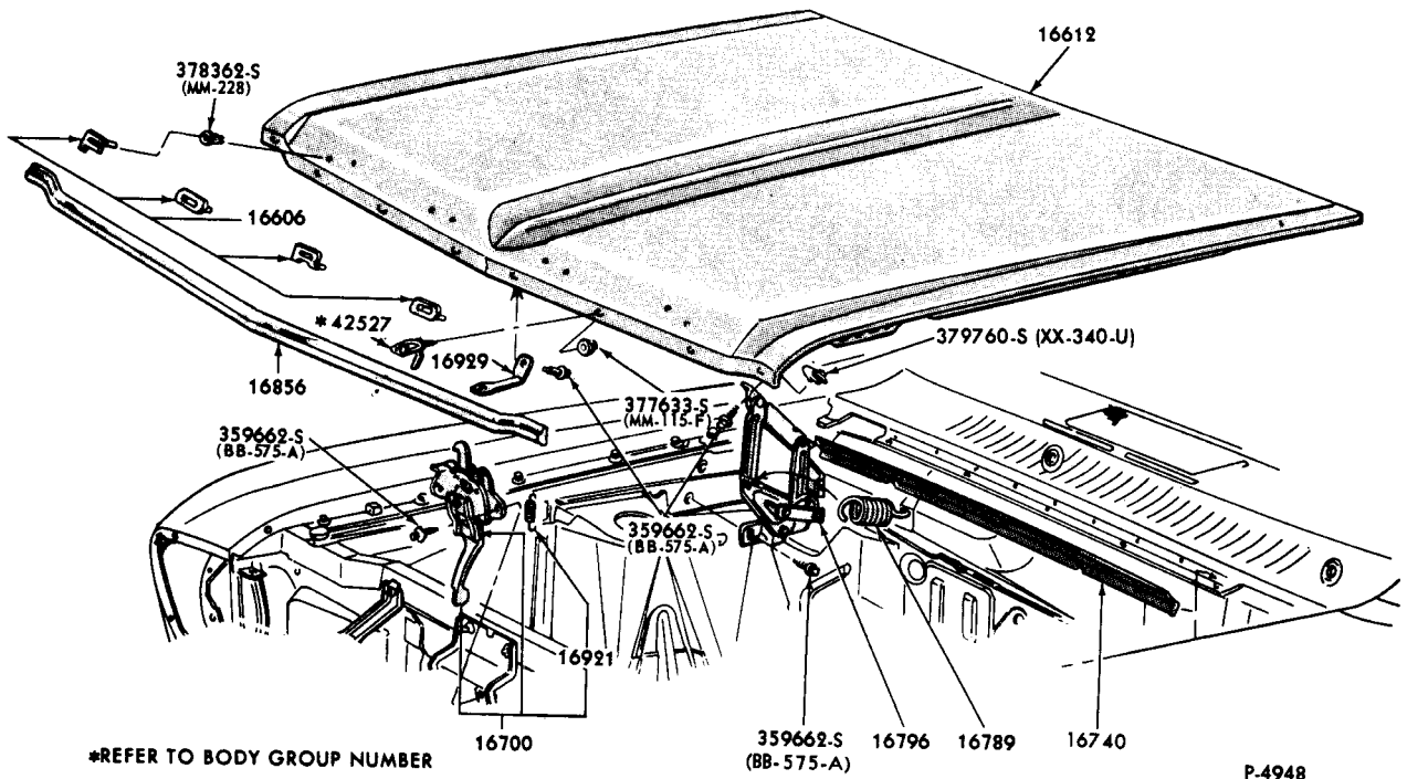
HOOD and RELATED PARTS 1966/67 FALCON
