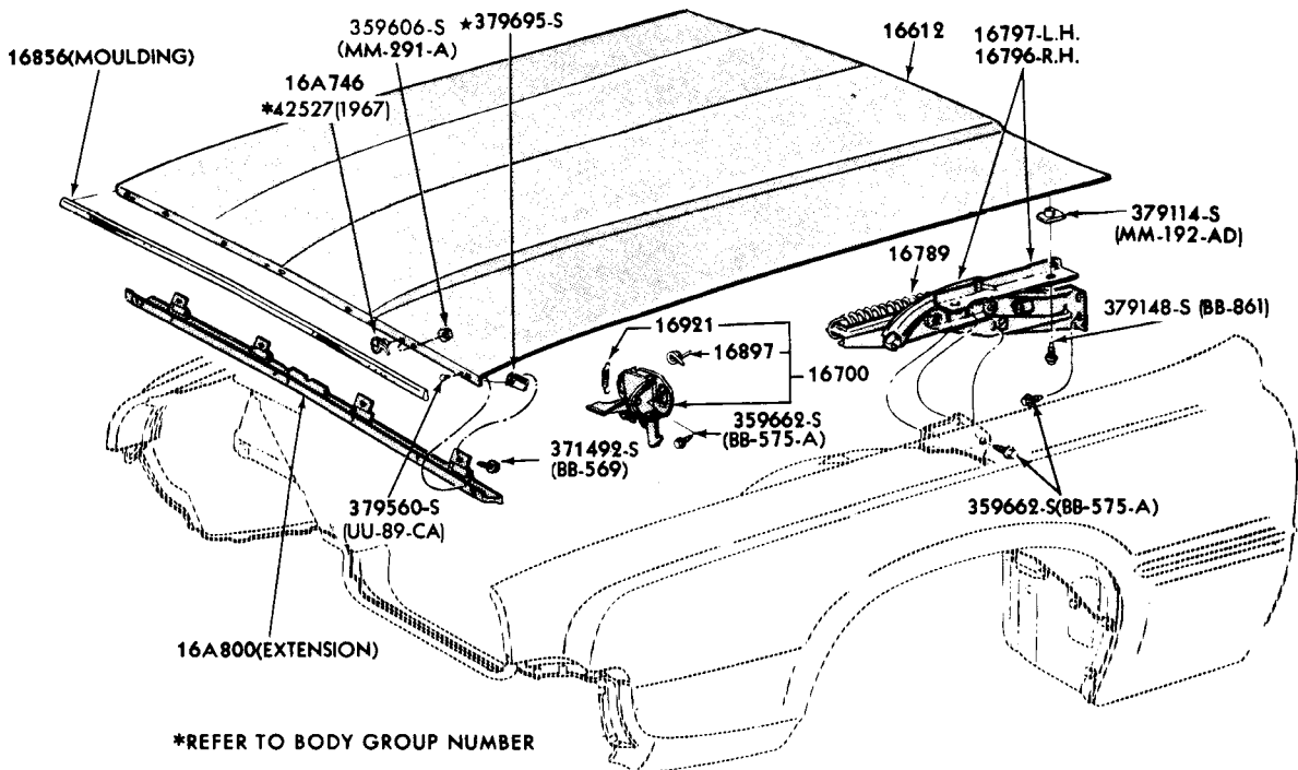
HOOD and RELATED PARTS 1967/69 THUNDERBIRD
