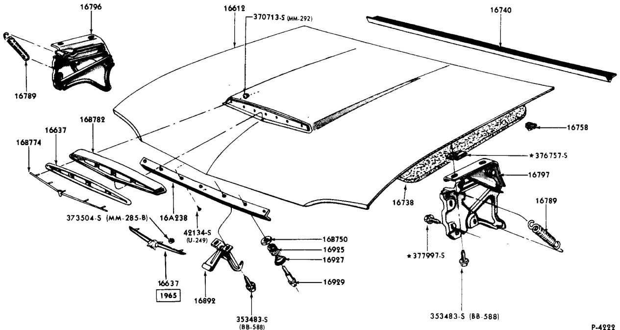
HOOD and RELATED PARTS 1965 THUNDERBIRD
