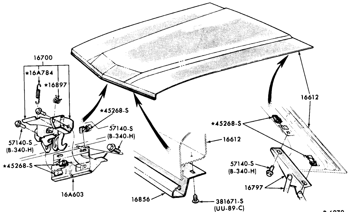
HOOD and RELATED PARTS 1970 MAVERICK
