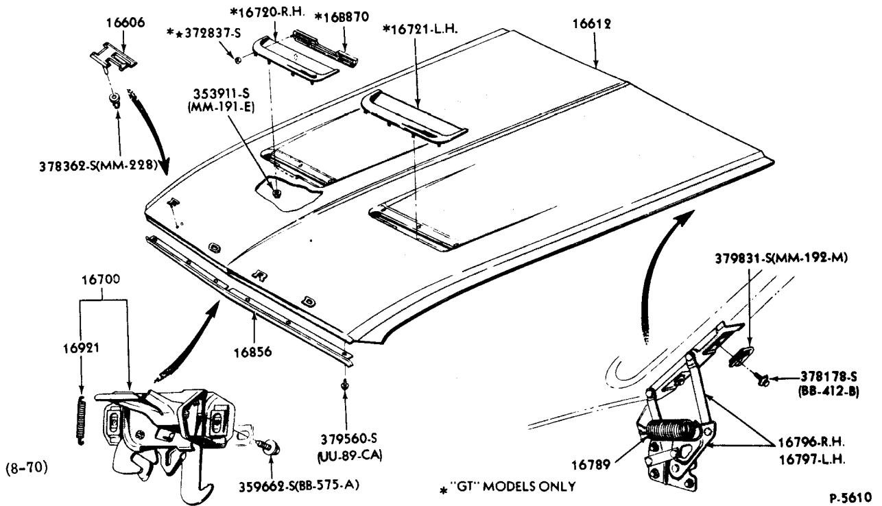
HOOD and RELATED PARTS 1967/68 MUSTANG
