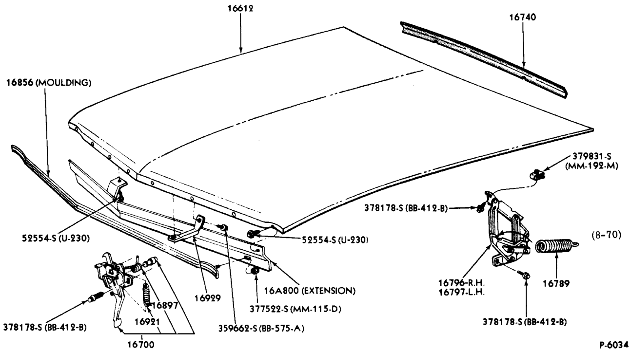
HOOD and RELATED PARTS 1968/70 FALCON
