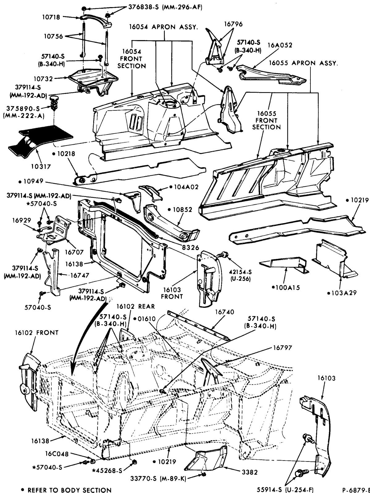
FRONT END SHEET METAL and RELATED PARTS 1970/72 MAVERICK
