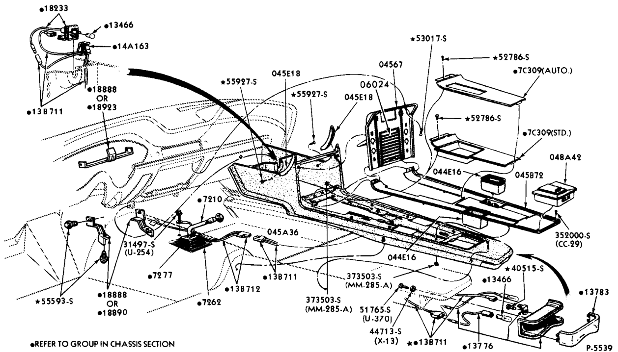
CONSOLE and RELATED PARTS 1967 MUSTANG
