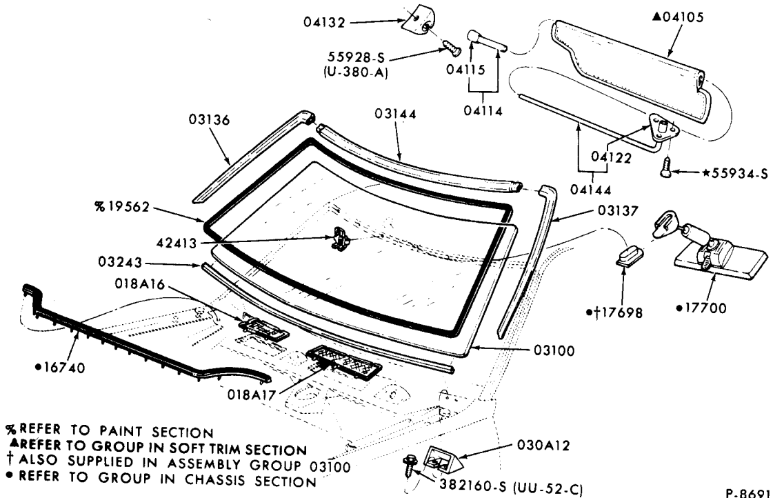
WINDSHIELD and RELATED PARTS 1972 THUNDERBIRD
