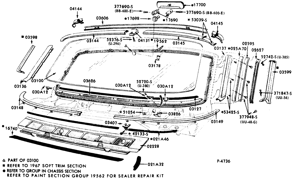
WINDSHIELD and RELATED PARTS 1965/68 FORD - BODY TYPE 76 - TYPICAL
