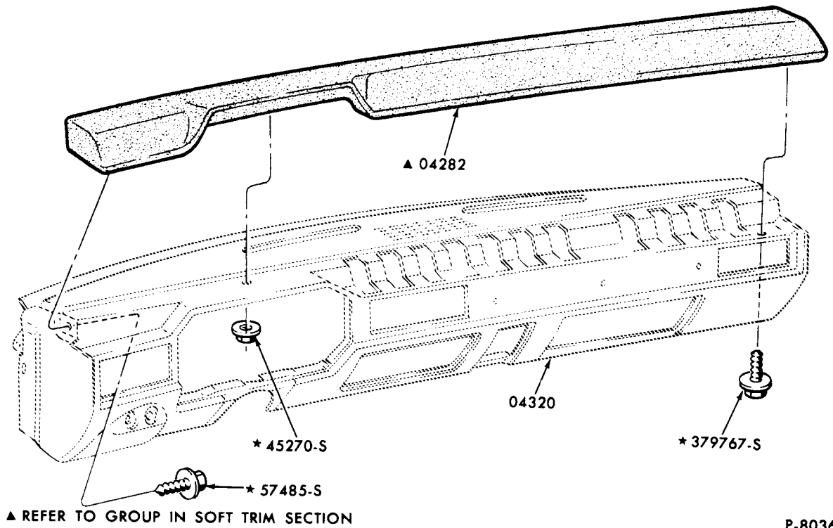
INSTRUMENT PANEL PAD and ATTACHING PARTS 1971/72 PINTO
