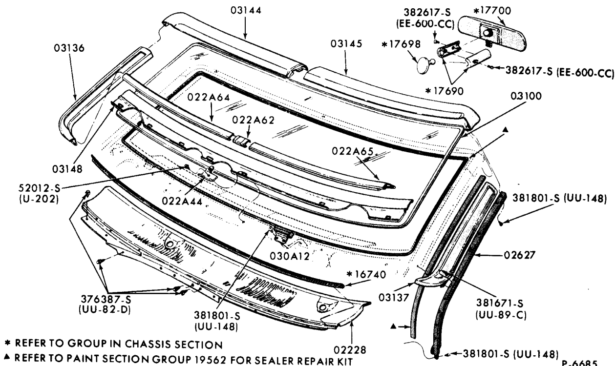
WINDSHIELD and RELATED PARTS 1969/70 FORD - BODY TYPE 76
