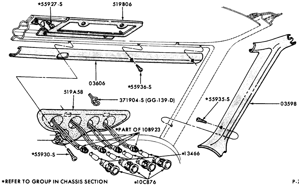
ROOF CONSOLE and RELATED PARTS 1970/71 THUNDERBIRD - BODY TYPE 65
