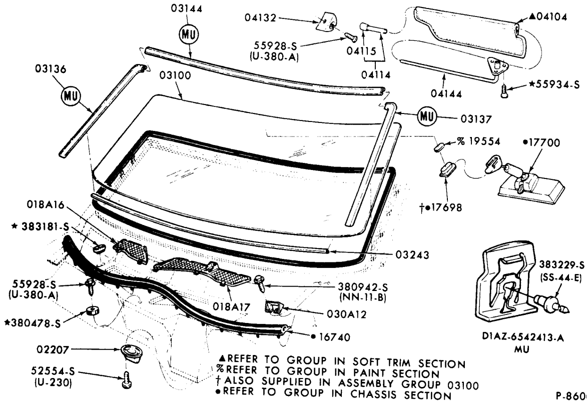
WINDSHIELD and RELATED PARTS 1972 TORINO
