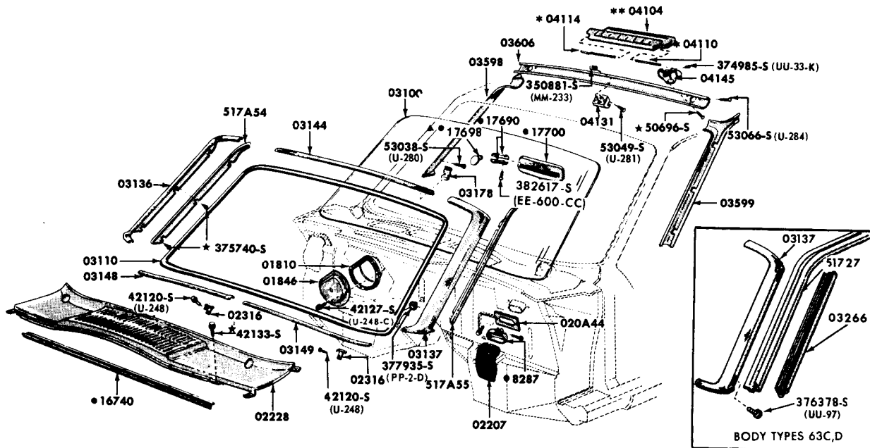
WINDSHIELD and RELATED PARTS 1965/68 MUSTANG - BODY TYPE 76
