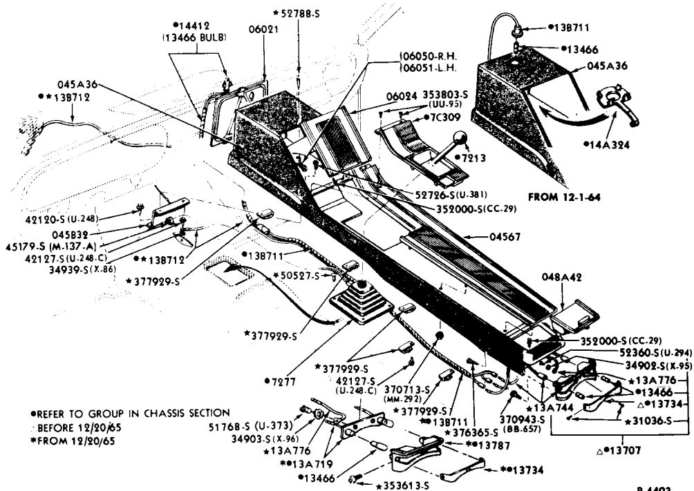
CONSOLE and RELATED PARTS 1965/66 MUSTANG (WITHOUT A/C)
