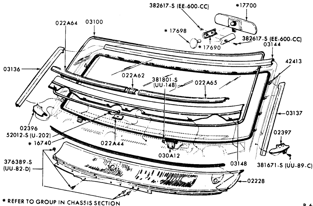
WINDSHIELD and RELATED PARTS 1969/70 FORD - BODY TYPES 54, 57, 62, 63, 65, 71
