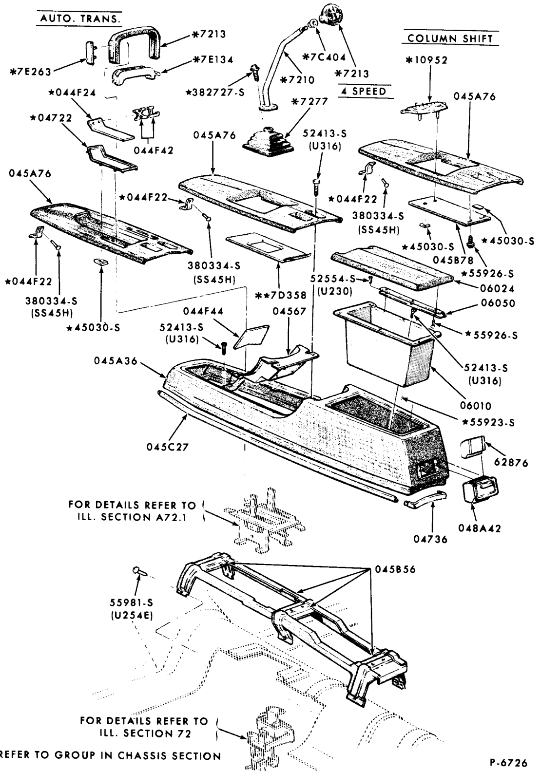
CONSOLE and RELATED PARTS 1969/71 FORD
