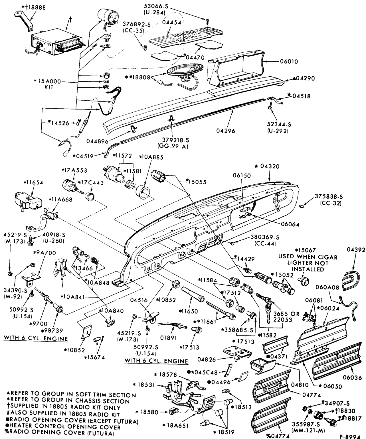
INSTRUMENT PANEL, PAD and RELATED PARTS 1965 FALCON
