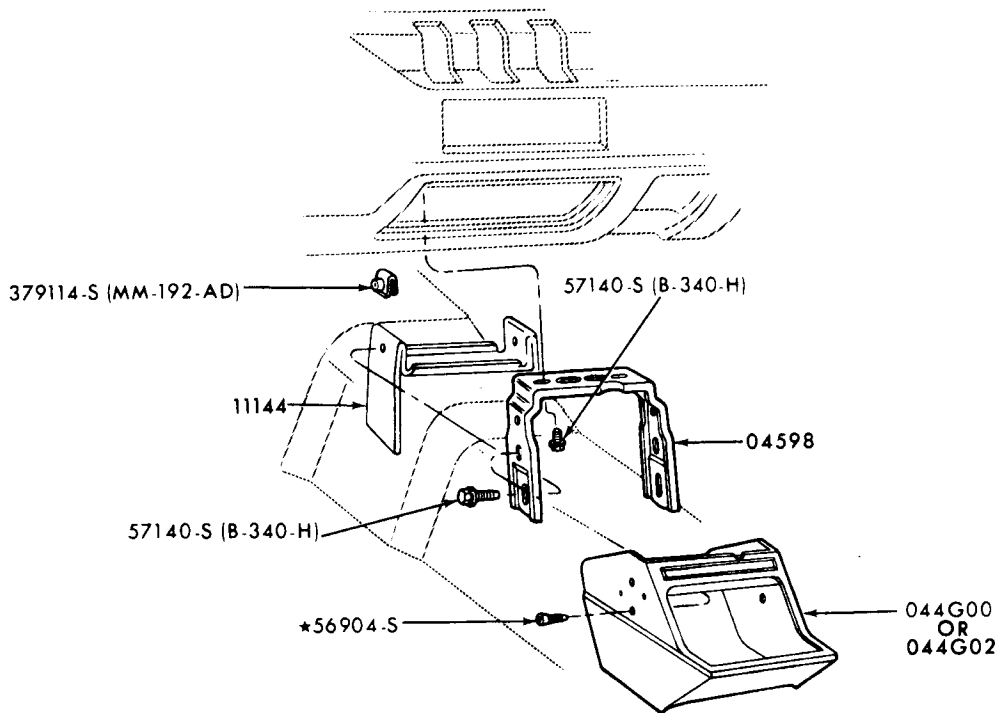
INSTRUMENT PANEL BRACE COVER 1972 PINTO
