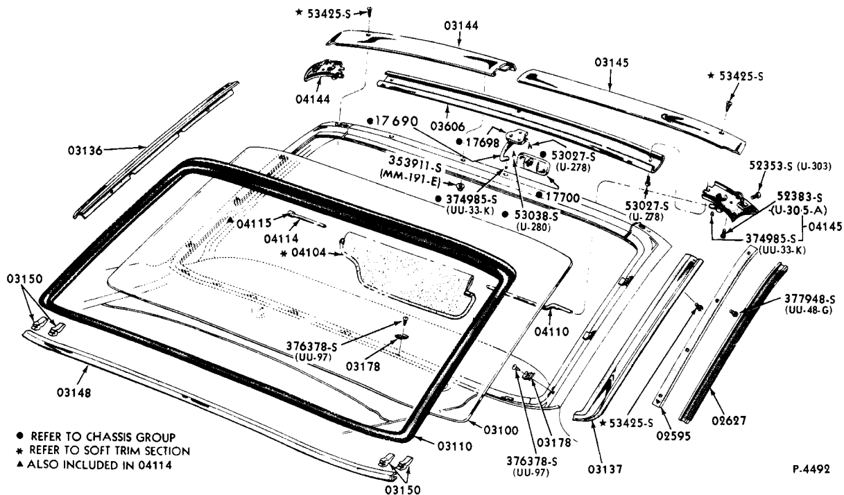
WINDSHIELD and RELATED PARTS 1965/68 MUSTANG - BODY TYPE 76
