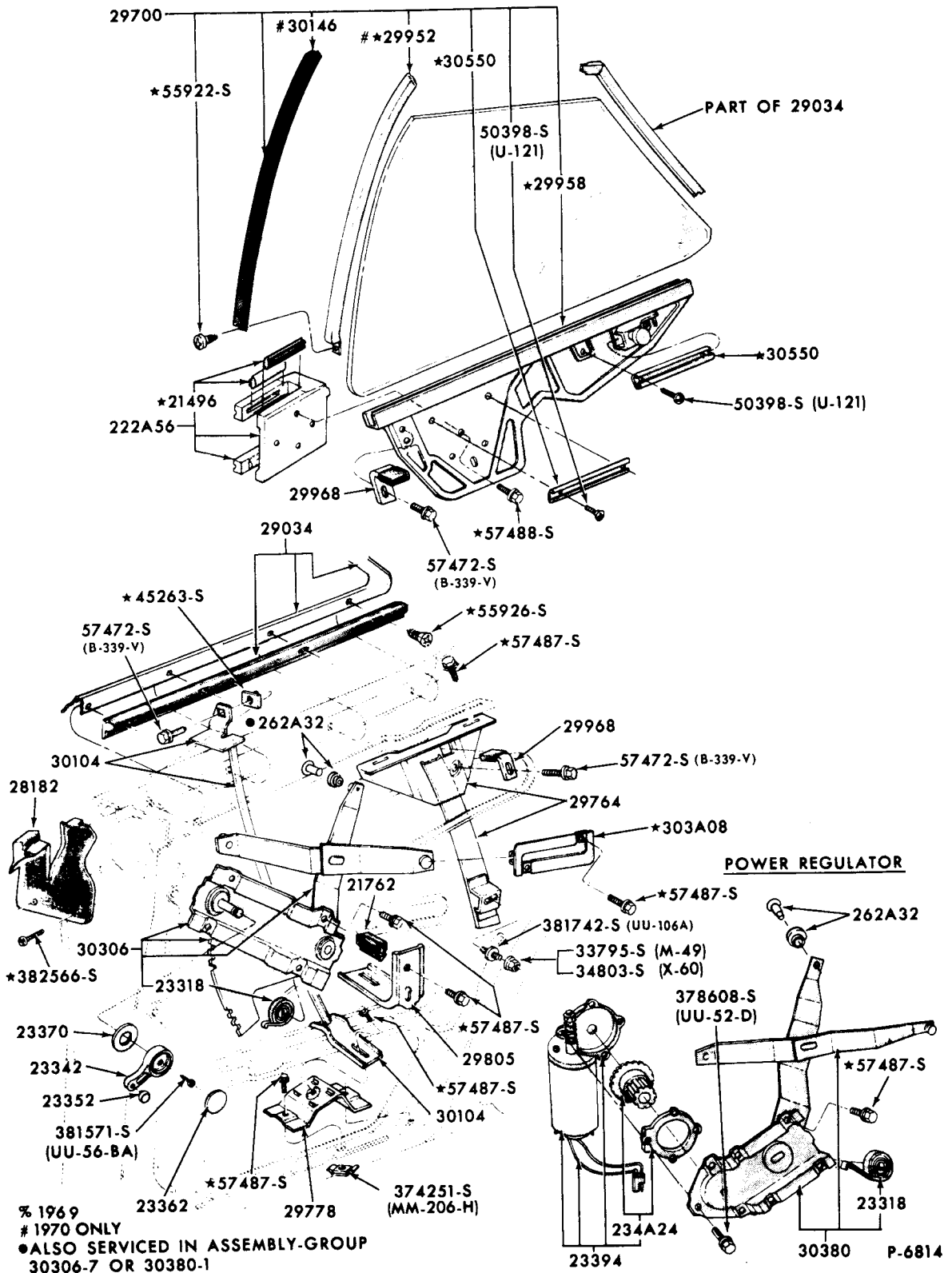
QUARTER WINDOW and RELATED PARTS
