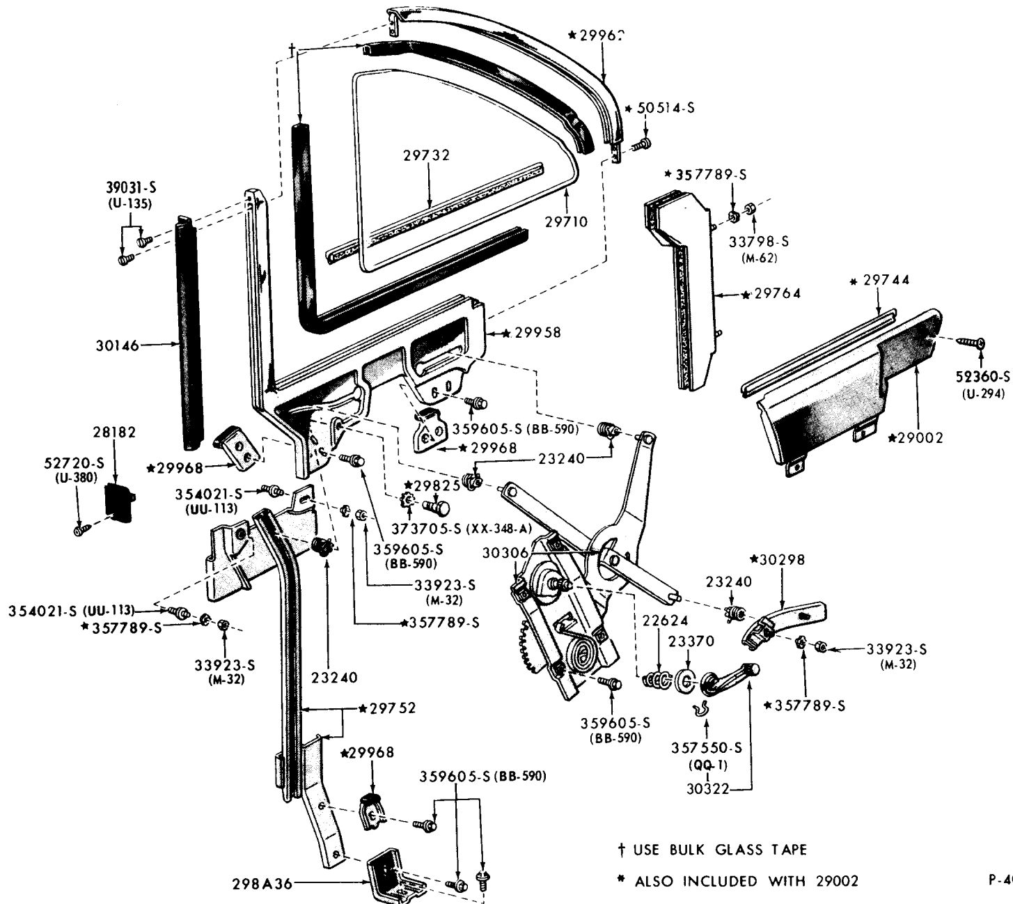
QUARTER WINDOW and RELATED PARTS 1965 FALCON - BODY TYPE 76
