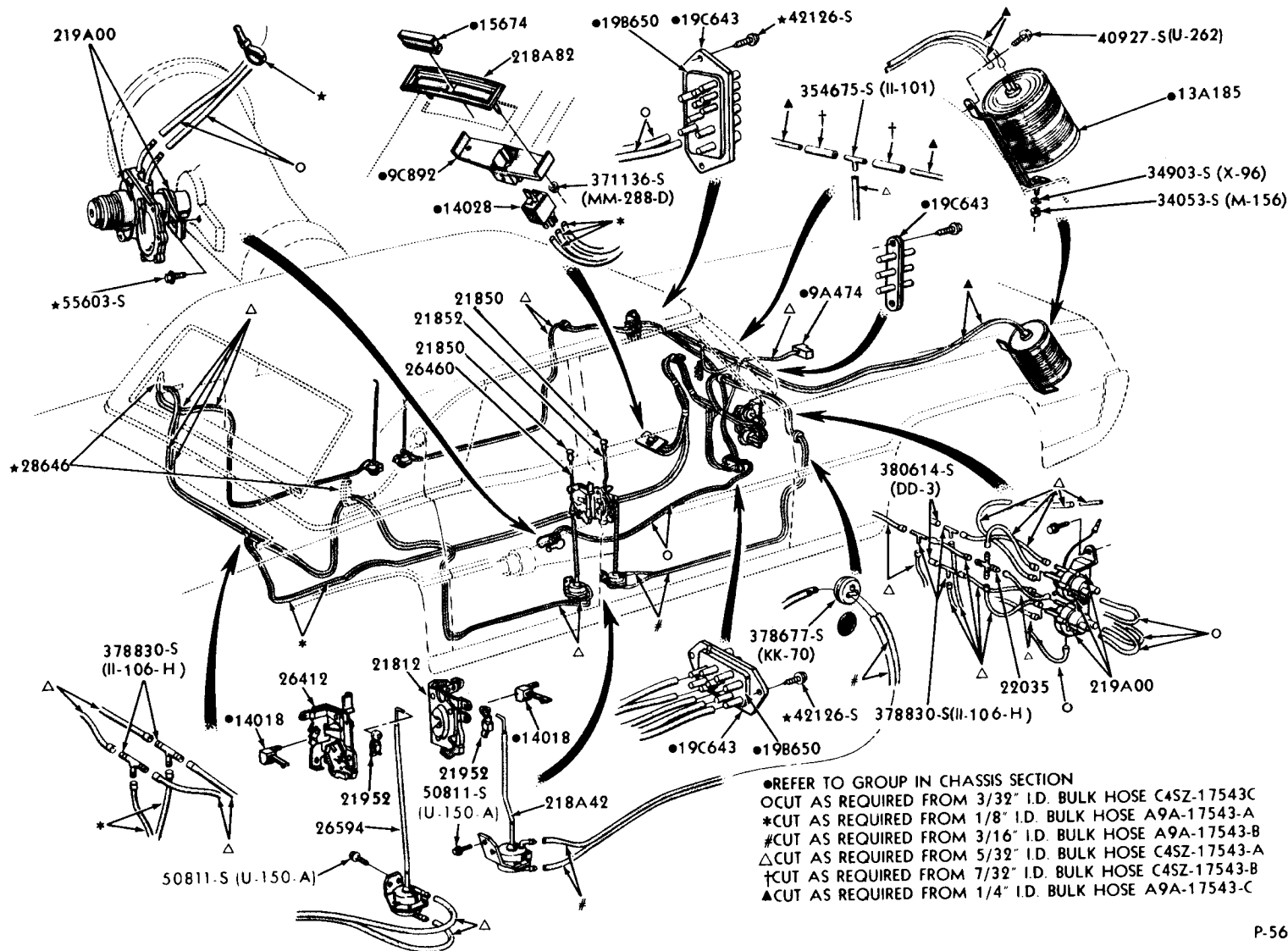
VACUUM DOOR LATCH SYSTEM 1967 THUNDERBIRD
