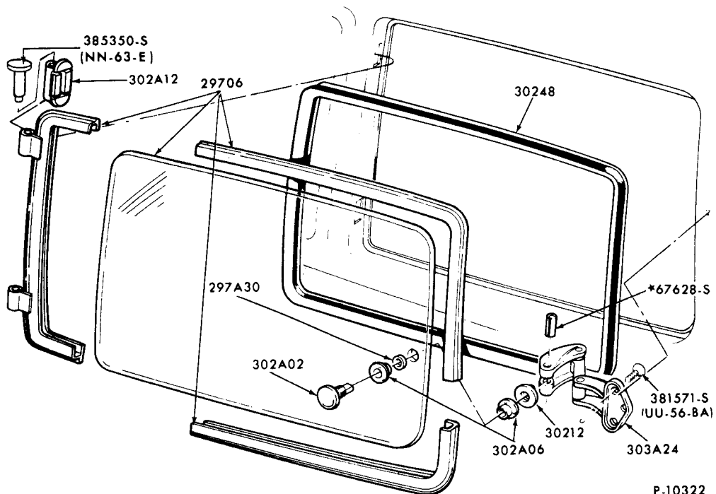
QUARTER WINDOW and RELATED PARTS - MOVEABLE 1972 PINTO - BODY TYPE 73 - "FROM 5/1/72"
