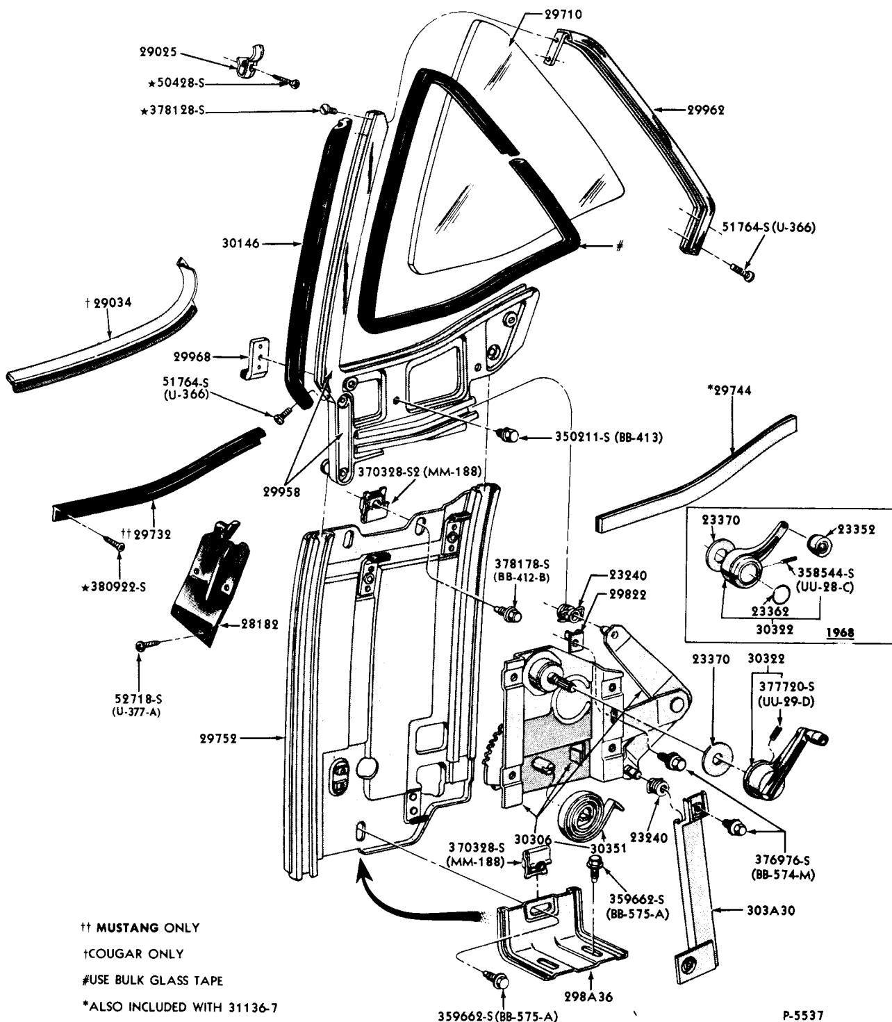
QUARTER WINDOW and RELATED PARTS 1967/68 MUSTANG - BODY TYPES 65, 76
