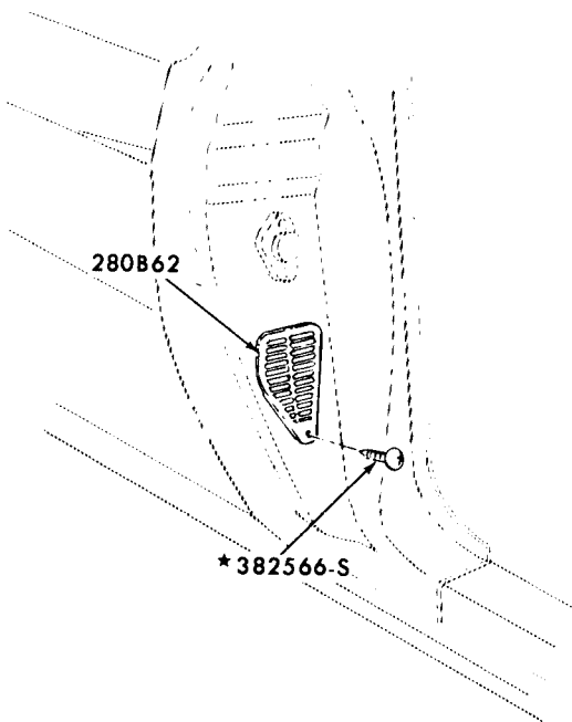
PRESSURE RELEASE VENT - QUARTER 1970/72 ALL
