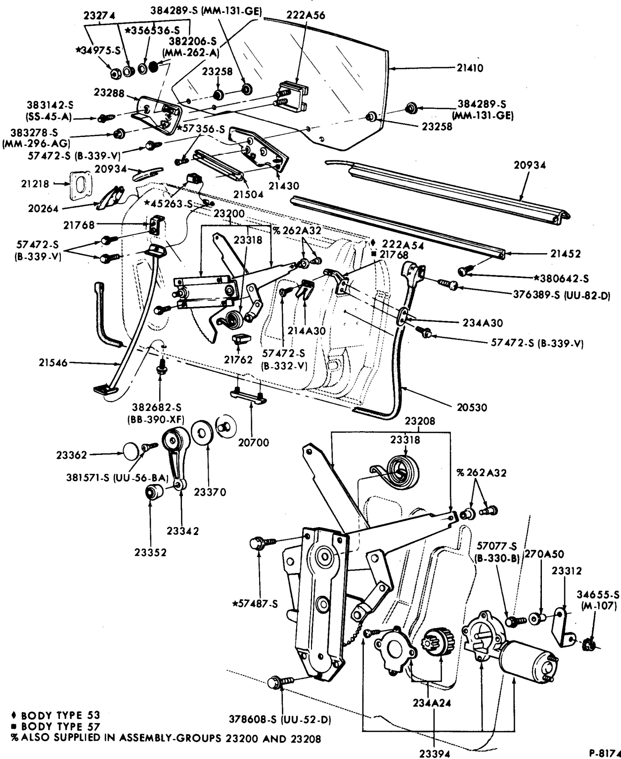
FRONT DOOR WINDOW and RELATED PARTS 1971/72 FORD - BODY TYPES 53, 57
