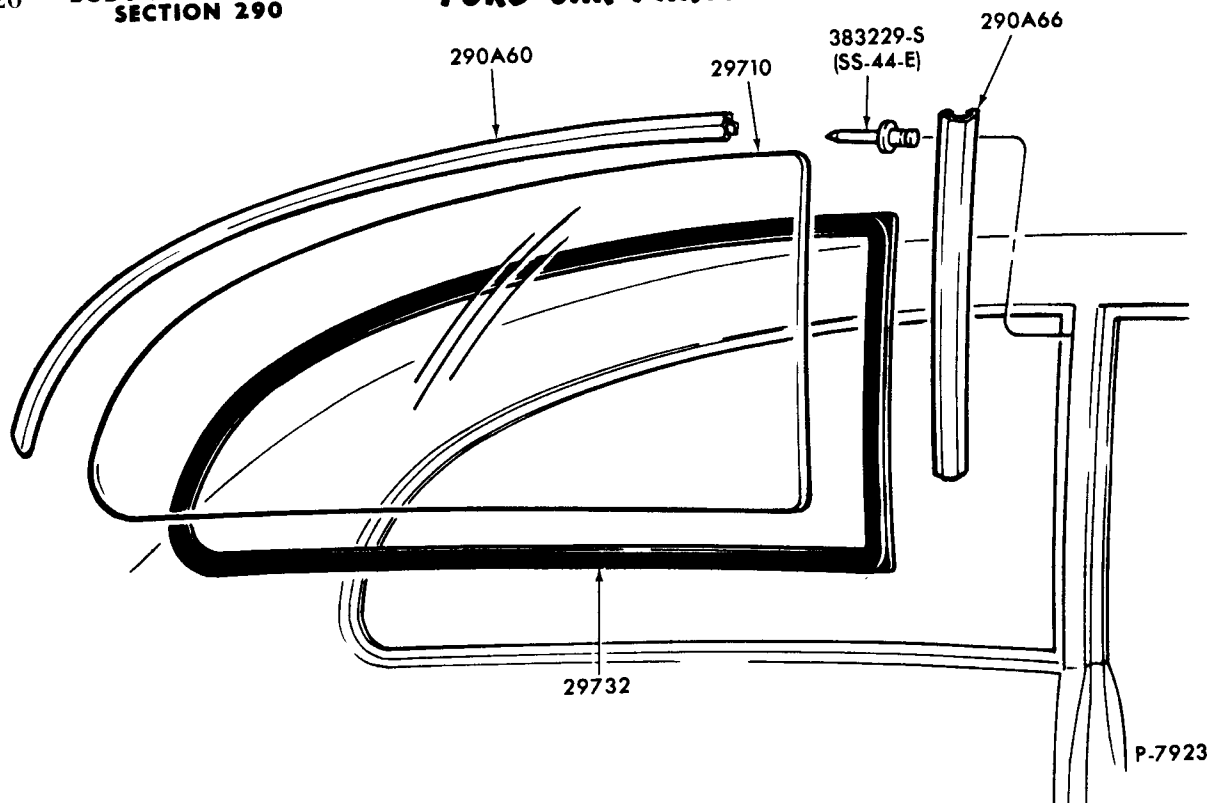
QUARTER WINDOW and RELATED PARTS - STATIONARY 1971/72 PINTO - BODY TYPES 62, 64
