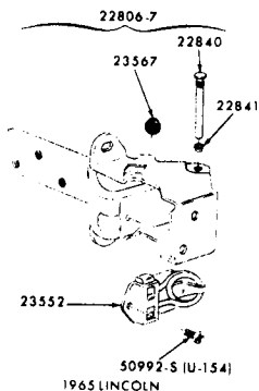
1965 LINCOLN
