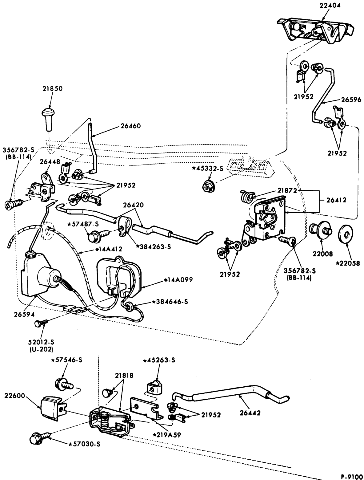
ELECTRIC REAR DOOR LATCH SYSTEM 1972 TORINO - BODY TYPES 53, 71
