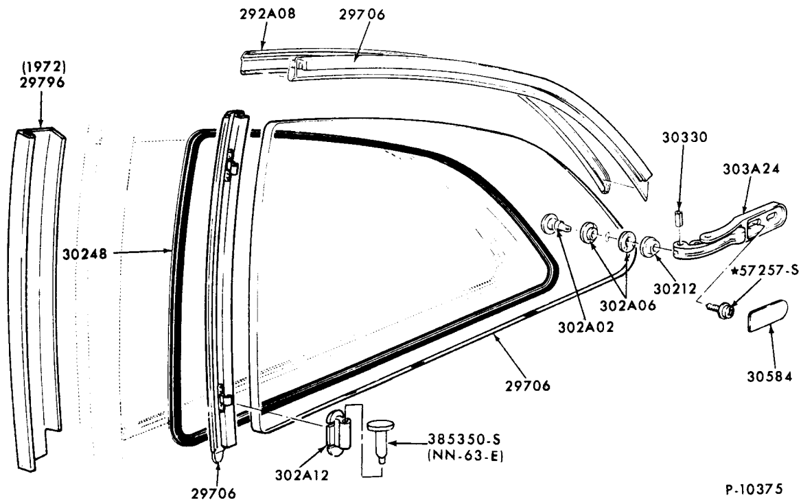
QUARTER WINDOW and RELATED PARTS - MOVEABLE 1972 PINTO - BODY TYPES 62, 64 - "From 5/1/72"
