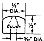
359953-S (CC-18)
