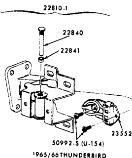
1965/66 THUNDERBIRD
