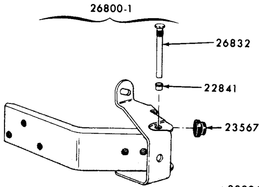
1965 LINCOLN
