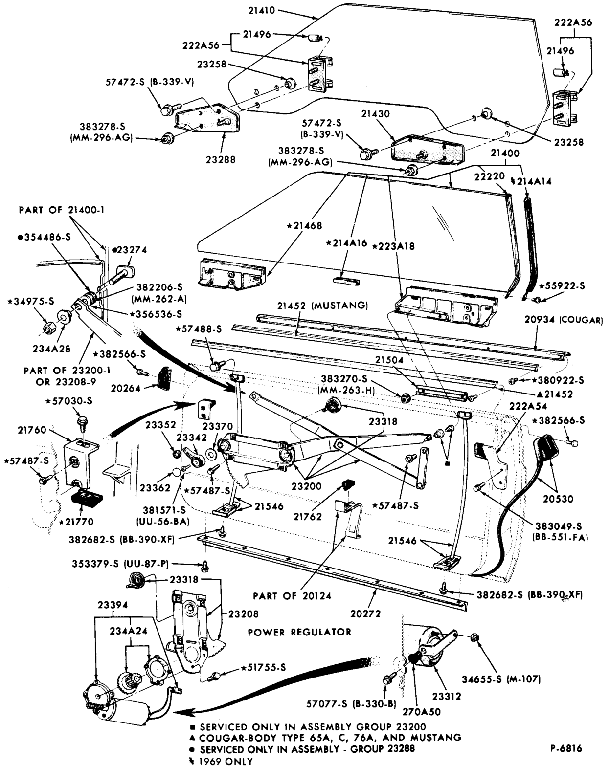
FRONT DOOR WINDOW and RELATED PARTS 1969/70 MUSTANG
