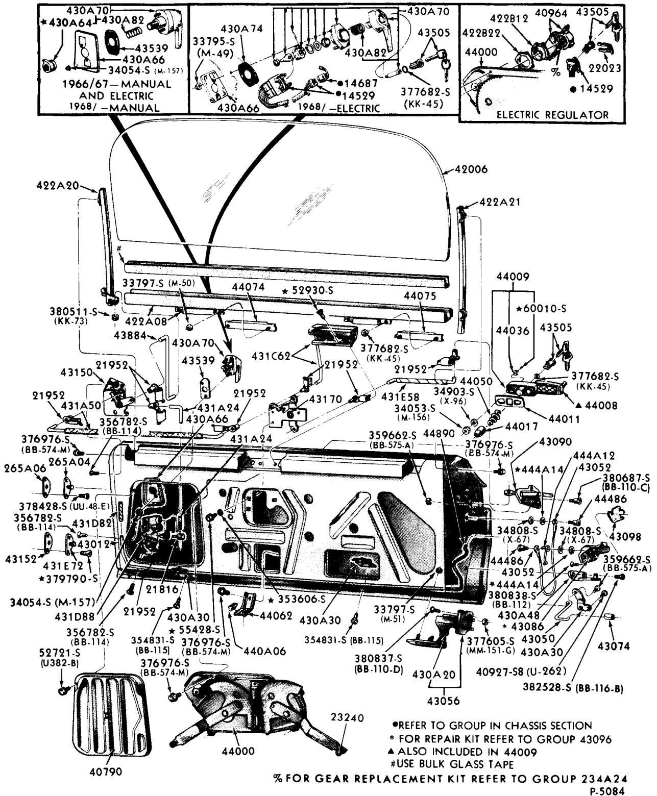
TAIL GATE WINDOW and RELATED PARTS - DUAL ACTION 1966/71 FAIRLANE and FALCON - BODY TYPE 71
