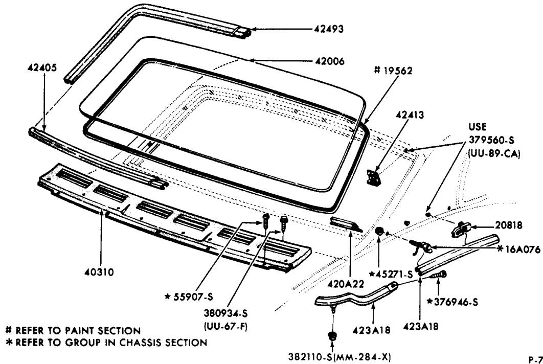
BACK WINDOW and RELATED PARTS 1970/71 THUNDERBIRD - BODY TYPE 65 A, C
