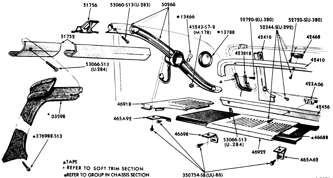
BACK WINDOW and ROOF SIDE MOULDINGS 1967/70 THUNDERBIRD - BODY TYPE 57
