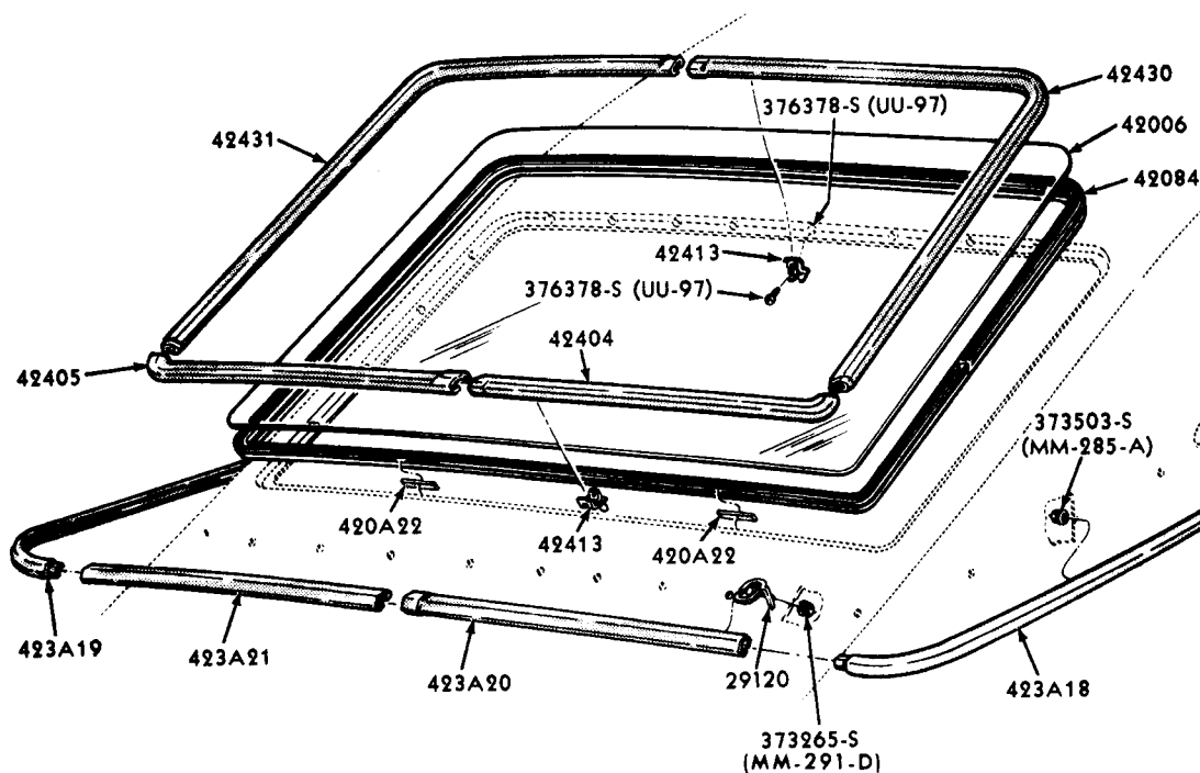
BACK WINDOW and RELATED PARTS - OUTSIDE 1967 FORD - BODY TYPE 63
