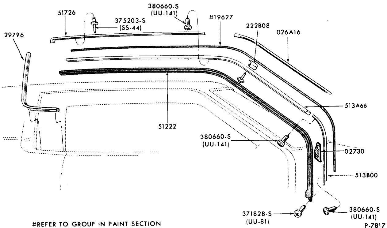
ROOF SIDE MOULDINGS and WEATHERSTRIPS 1970/72 FORD - BODY TYPE 65
