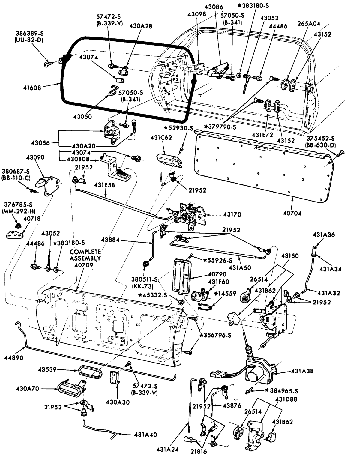
TAILGATE PARTS - HINGE and LATCH 1972 TORINO - BODY TYPE 71
