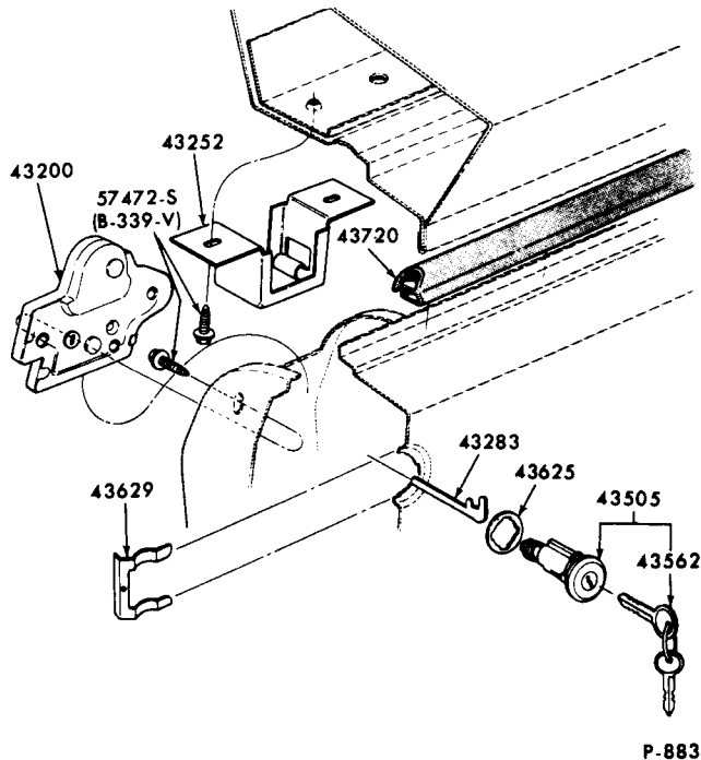
LUGGAGE COMPARTMENT DOOR LATCH and RELATED PARTS 1972 MAVERICK
