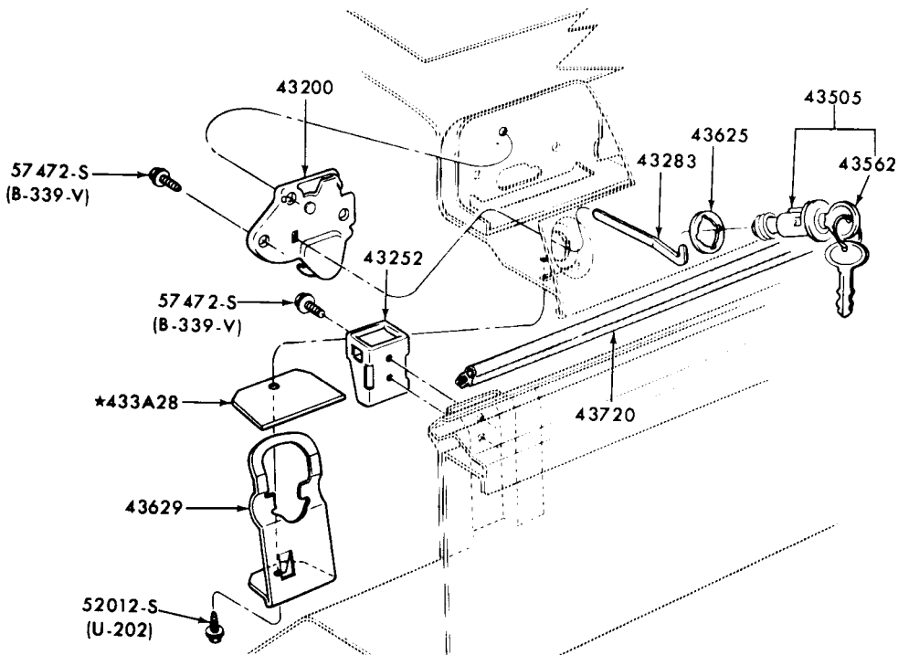
LUGGAGE COMPARTMENT DOOR LATCH and RELATED PARTS 1972 THUNDERBIRD
