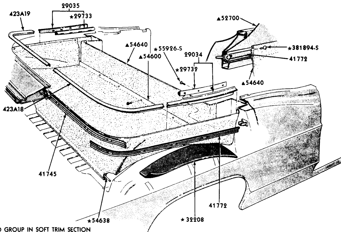
BACK BELT MOULDINGS 1968/70 FORD - BODY TYPE 76
