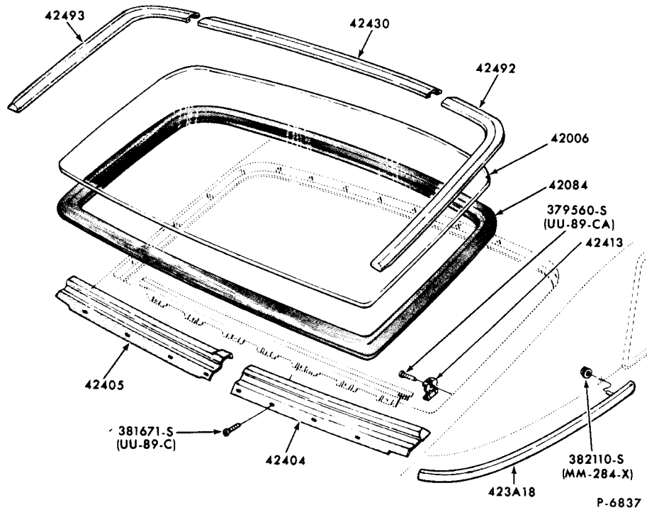
BACK WINDOW and RELATED PARTS 1970/72 MAVERICK - BODY TYPE 62
