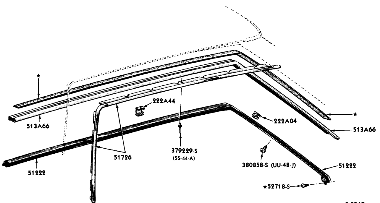
ROOF SIDE WEATHERSTRIPS and RELATED PARTS
