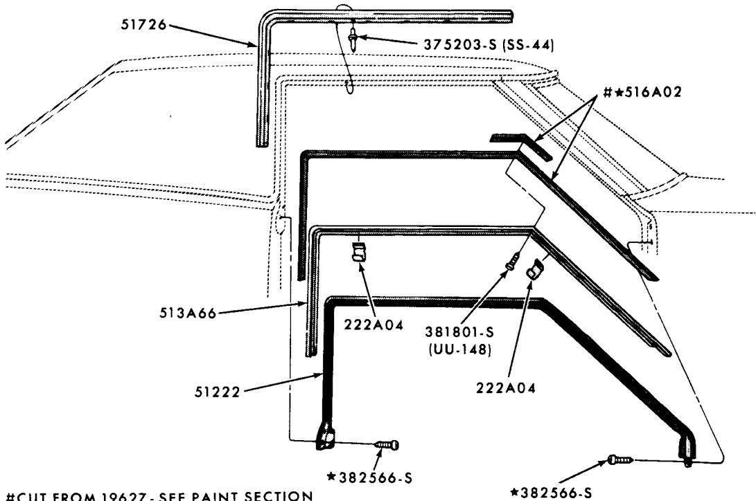
ROOF SIDE WEATHERSTRIPS and RELATED PARTS 1969 THUNDERBIRD - BODY TYPE 65B, D
