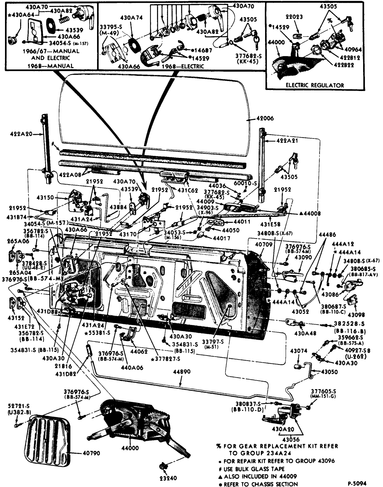
TAIL GATE WINDOW and RELATED PARTS - DUAL ACTION 1966/68 FORD - BODY TYPE 71
