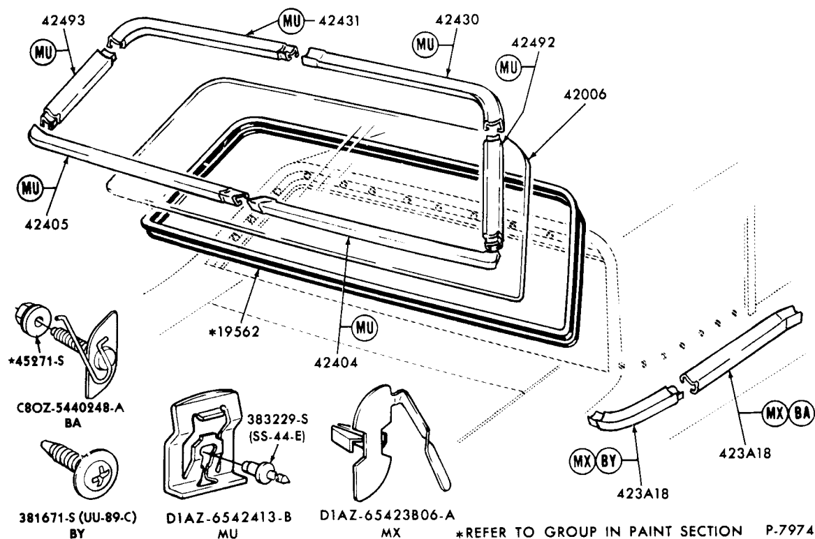
BACK WINDOW and RELATED PARTS - OUTSIDE 1971/72 FORD - BODY TYPE 65
