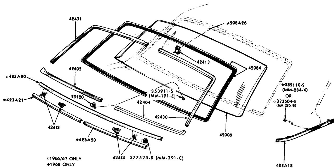
BACK WINDOW and RELATED PARTS 1966/69 FAIRLANE/TORINO and 1966/70 FALCON - BODY TYPE 54
