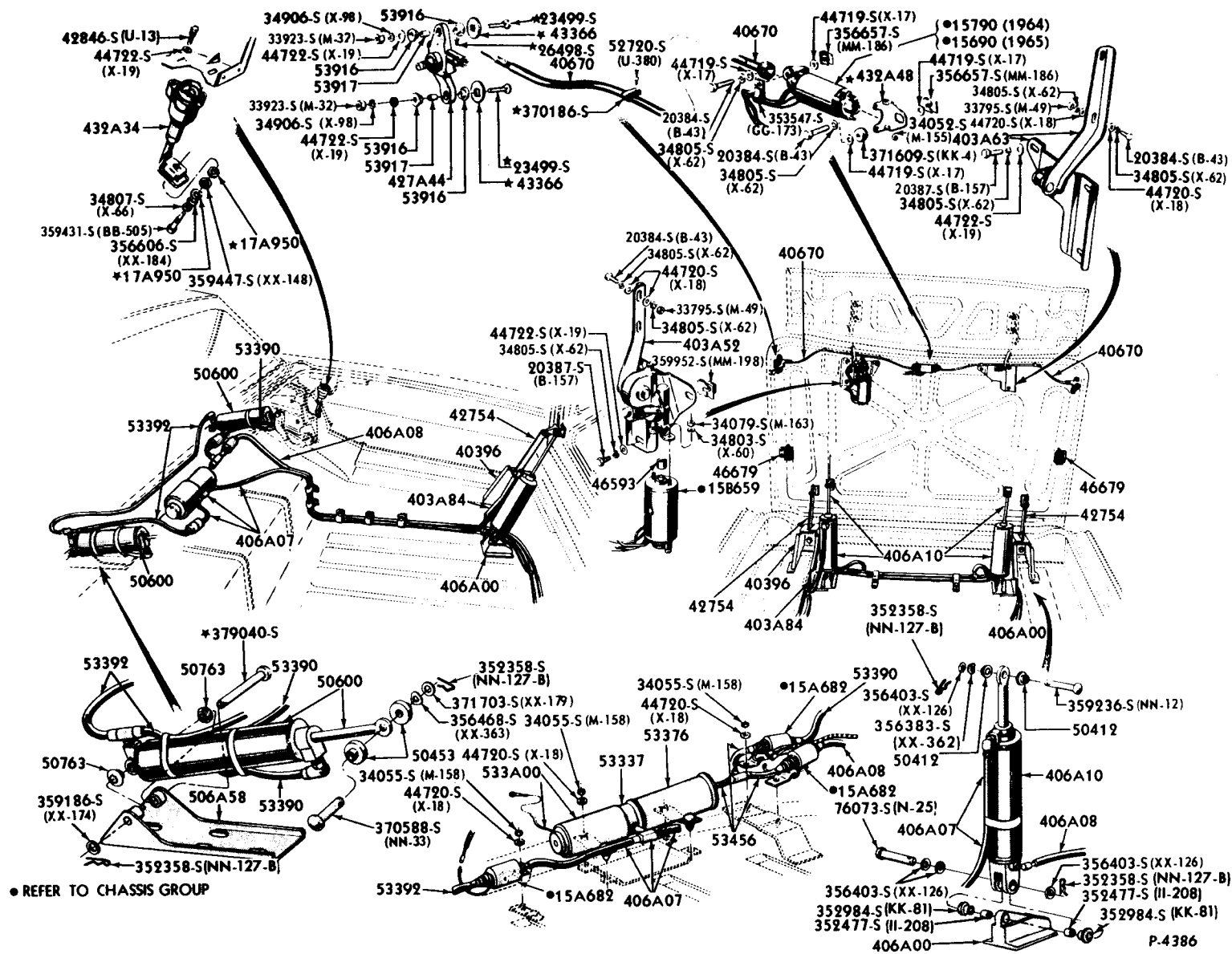
FOLDING TOP and LUGGAGE COMPARTMENT HYDRAULIC LIFT and RELATED PARTS 1965/66 THUNDERBIRD - BODY TYPE 76
