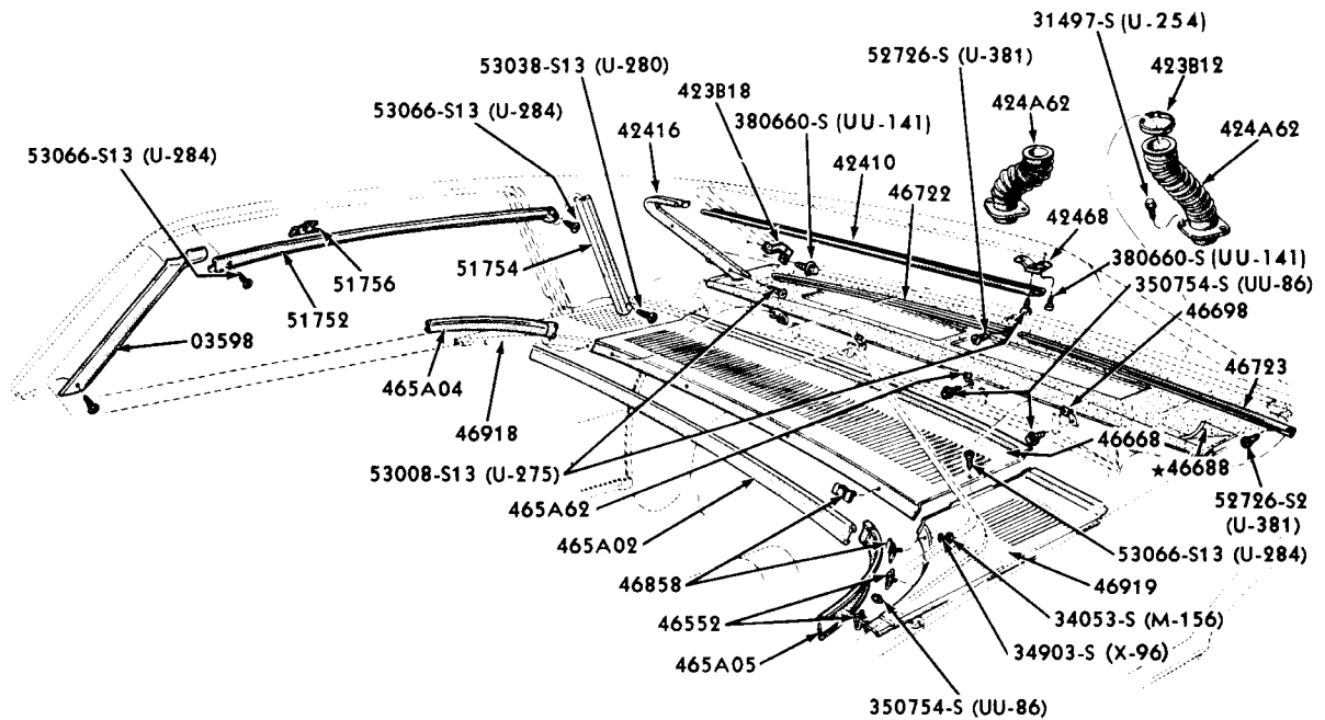
BACK WINDOW and ROOF SIDE MOULDINGS - INSIDE 1967/70 THUNDERBIRD - BODY TYPE 65
