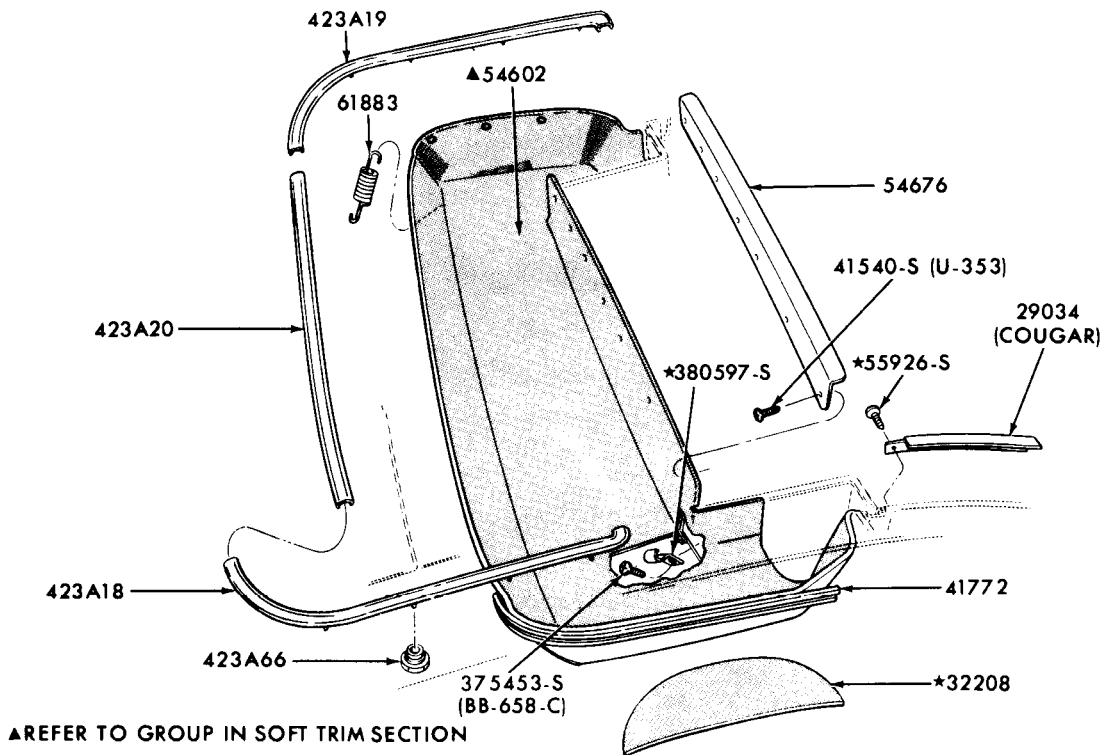
BACK BELT MOULDINGS and RELATED PARTS 1971/72 MUSTANG - BODY TYPE 76
