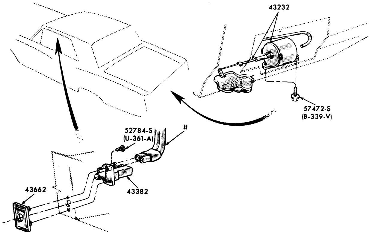
LUGGAGE COMPARTMENT VACUUM DOOR LATCH SYSTEM 1970/71 ALL
