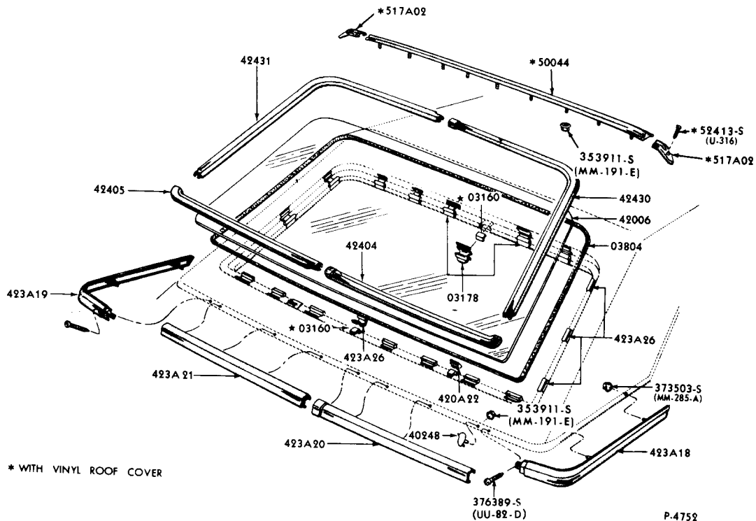
BACK WINDOW and RELATED PARTS - OUTSIDE 1965 FORD - BODY TYPE 63
