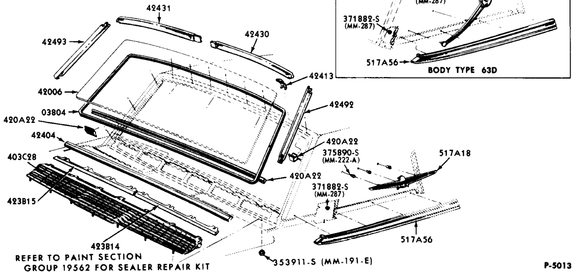
BACK WINDOW and RELATED PARTS-OUTSIDE 1966 THUNDERBIRD-BODY TYPES 63C, D
