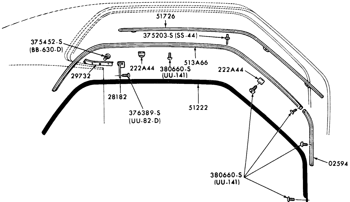
ROOF SIDE MOULDINGS and WEATHERSTRIPS 1971/72 MUSTANG - BODY TYPE 63
