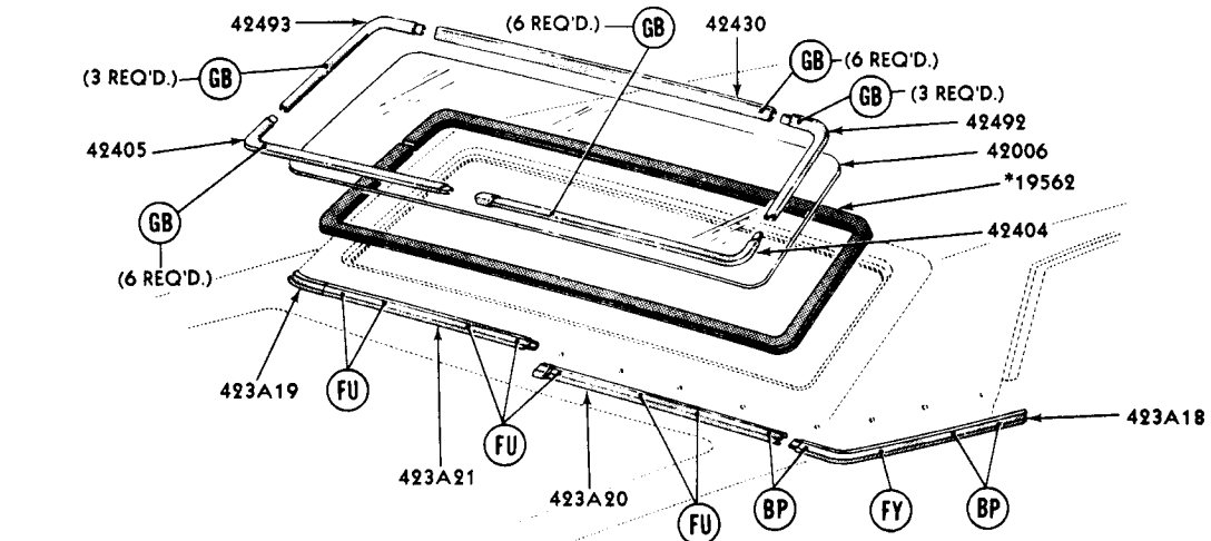
BACK WINDOW and RELATED PARTS - OUTSIDE 1969/70 FORD - BODY TYPES 54, 62
