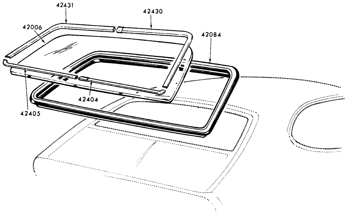
BACK WINDOW and RELATED PARTS - OUTSIDE 1971/72 PINTO - BODY TYPE 62 1971 PINTO - BODY TYPE 64
