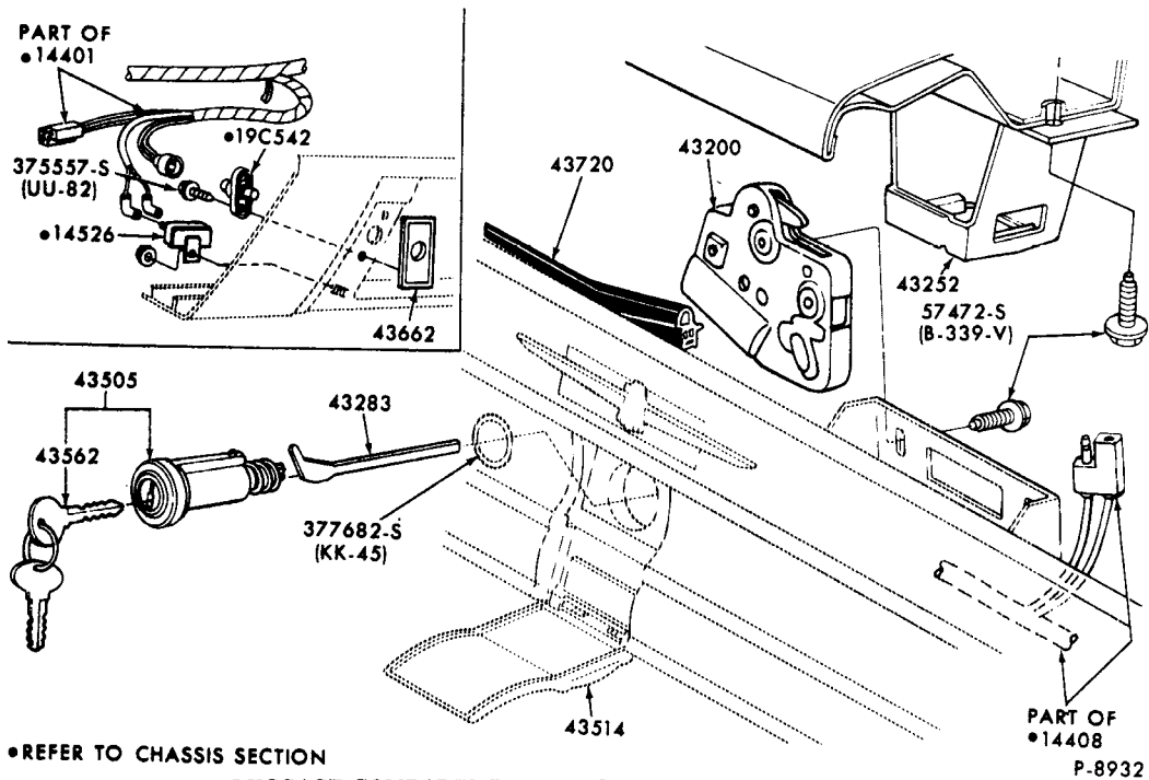
LUGGAGE COMPARTMENT ELECTRIC DOOR LATCH SYSTEM 1971/72 THUNDERBIRD
