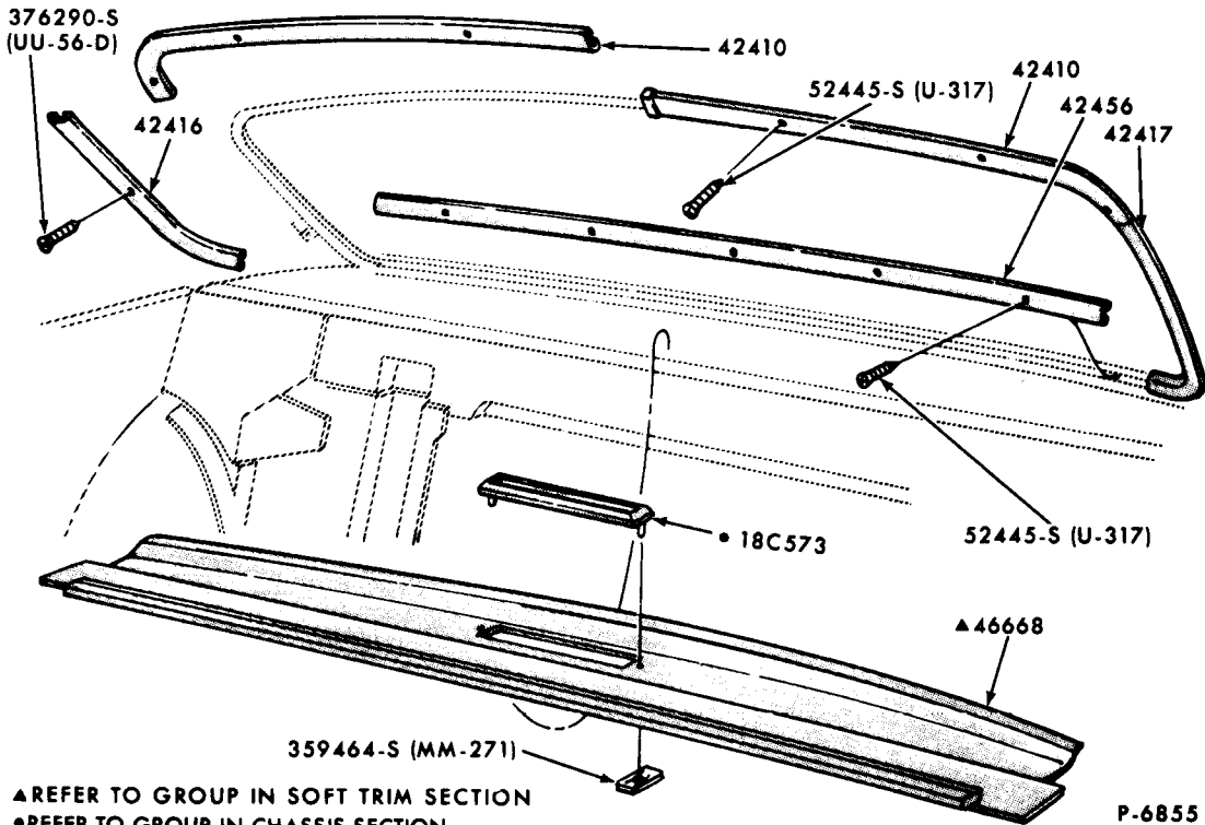
BACK WINDOW and RELATED PARTS - INSIDE 1969/72 FORD - BODY TYPES 53, 54, 57, 62, 63
