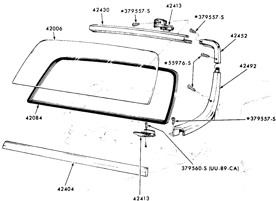
BACK WINDOW and RELATED PARTS 1970/71 FAIRLANE/TORINO - BODY TYPE 66
