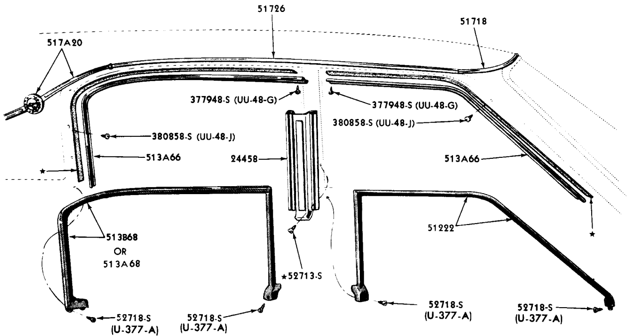
ROOF SIDE WEATHERSTRIPS and RELATED PARTS 1967/71 THUNDERBIRD - BODY TYPE 57
