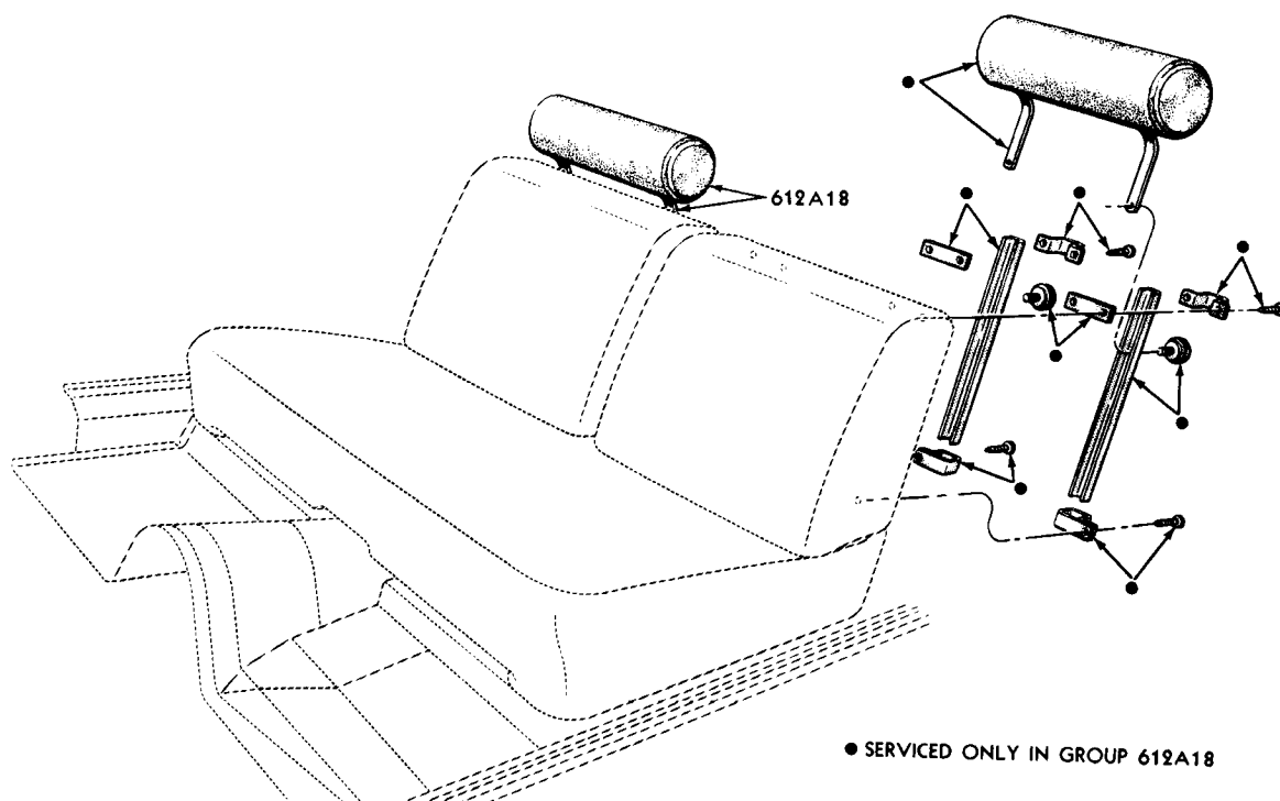
FRONT SEAT HEADREST and RELATED PARTS 1966/67 FORD, FAIRLANE, MUSTANG and FALCON
