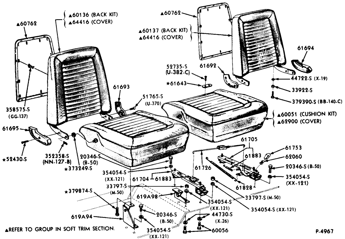
FRONT SEAT MECHANISM and RELATED PARTS - BUCKET 1966 BRONCO
