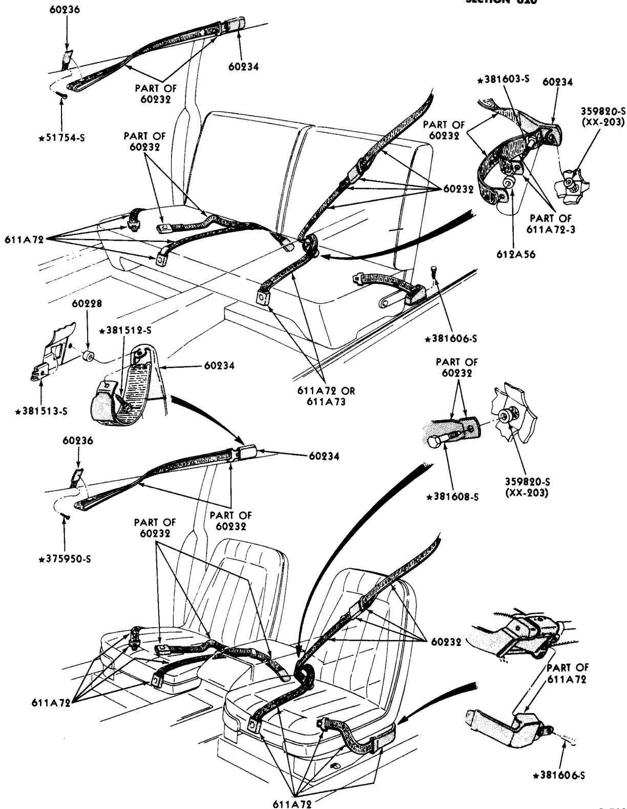
SHOULDER HARNESS INSTALLATION-FRONT SEAT
