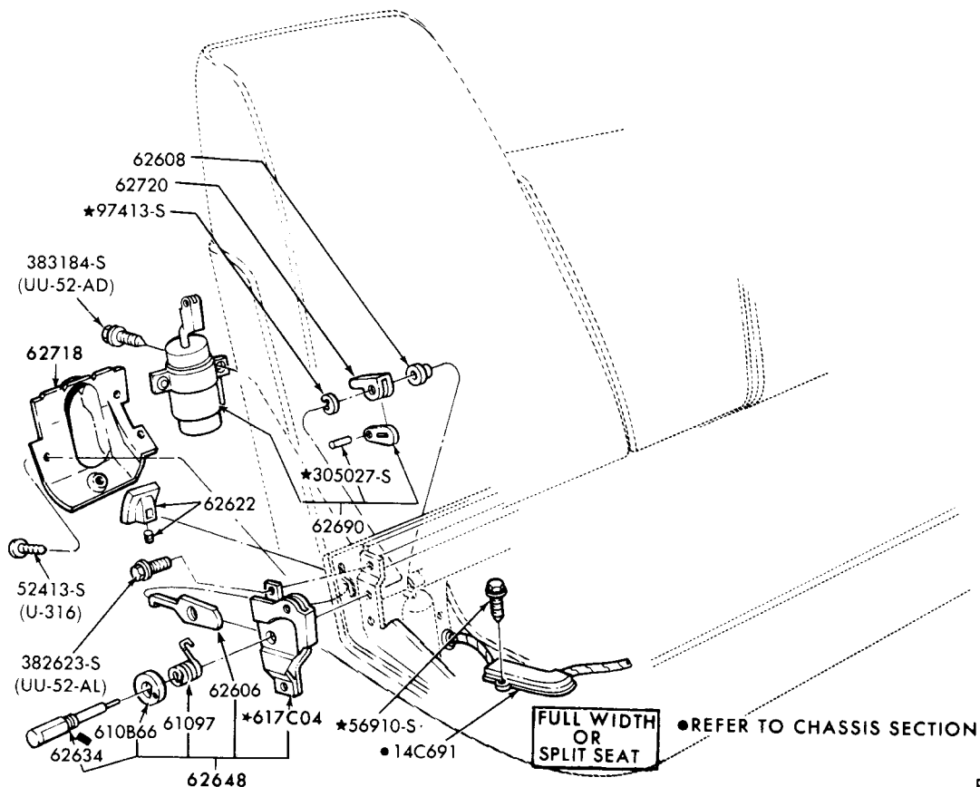
FRONT SEAT BACK LATCH MECHANISM - AUTOMATIC 1972 TORINO and THUNDERBIRD
