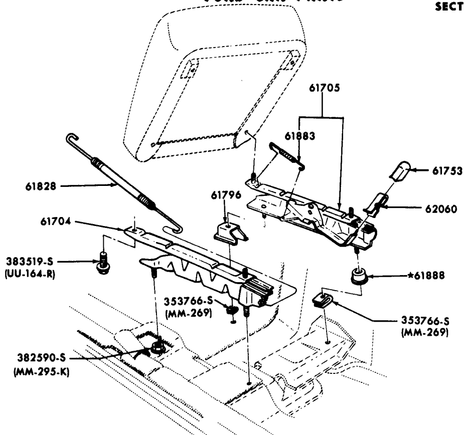
FRONT SEAT MECHANISM and RELATED PARTS - BUCKET - LOWER HALF 1971/72 MAVERICK
