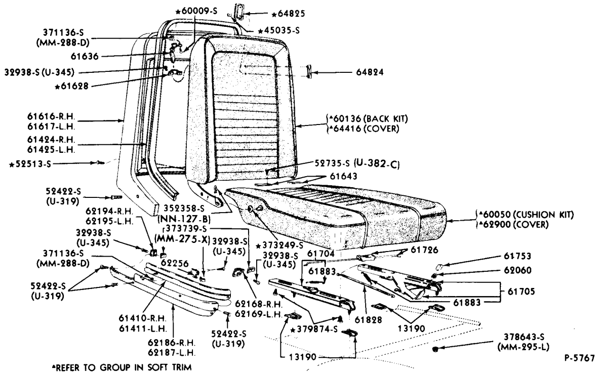
FRONT SEAT MECHANISM and RELATED PARTS - BUCKET 1967 MUSTANG - BODY TYPE 63B, 65B, 76B
