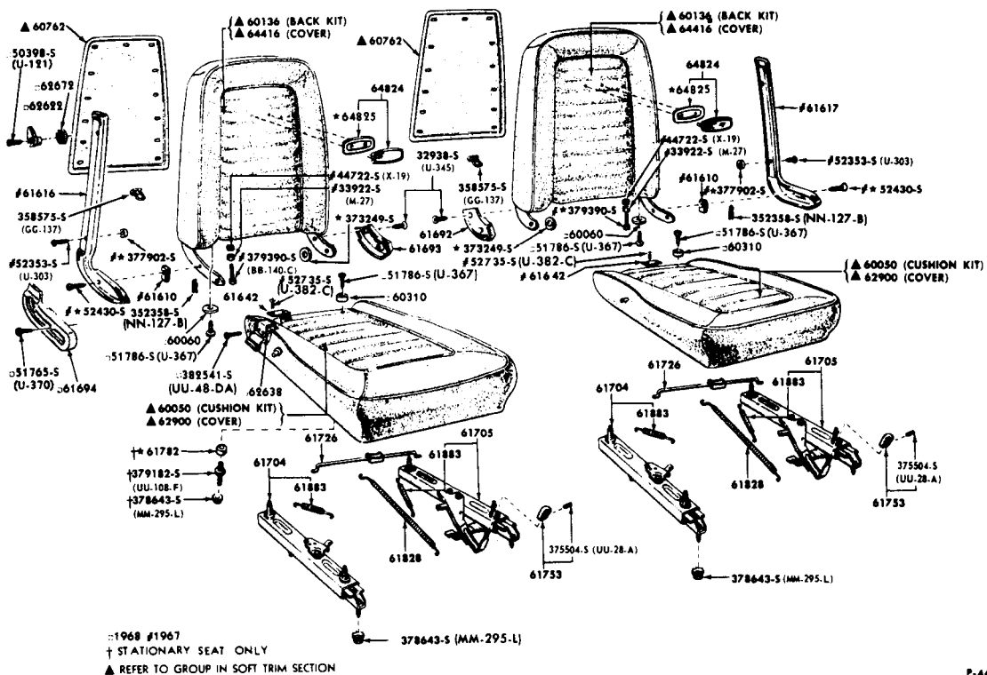
FRONT SEAT MECHANISM and RELATED PARTS - BUCKET 1965/66 MUSTANG, 1967 MUSTANG - BODY TYPE 63A, 65A, 76A and 1968/69 MUSTANG
