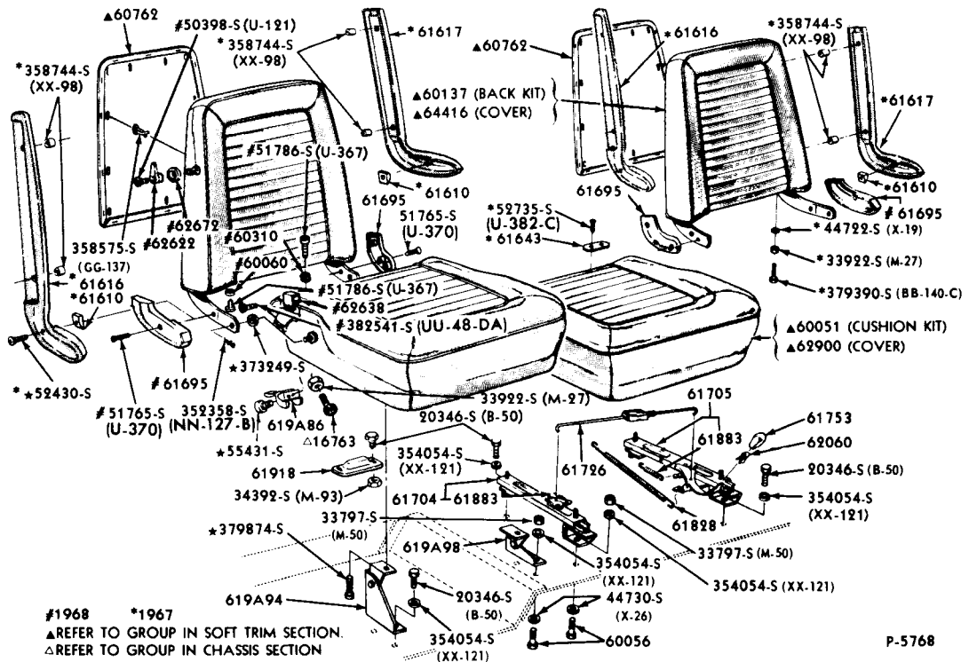
FRONT SEAT MECHANISM and RELATED PARTS - BUCKET 1967/71 BRONCO
