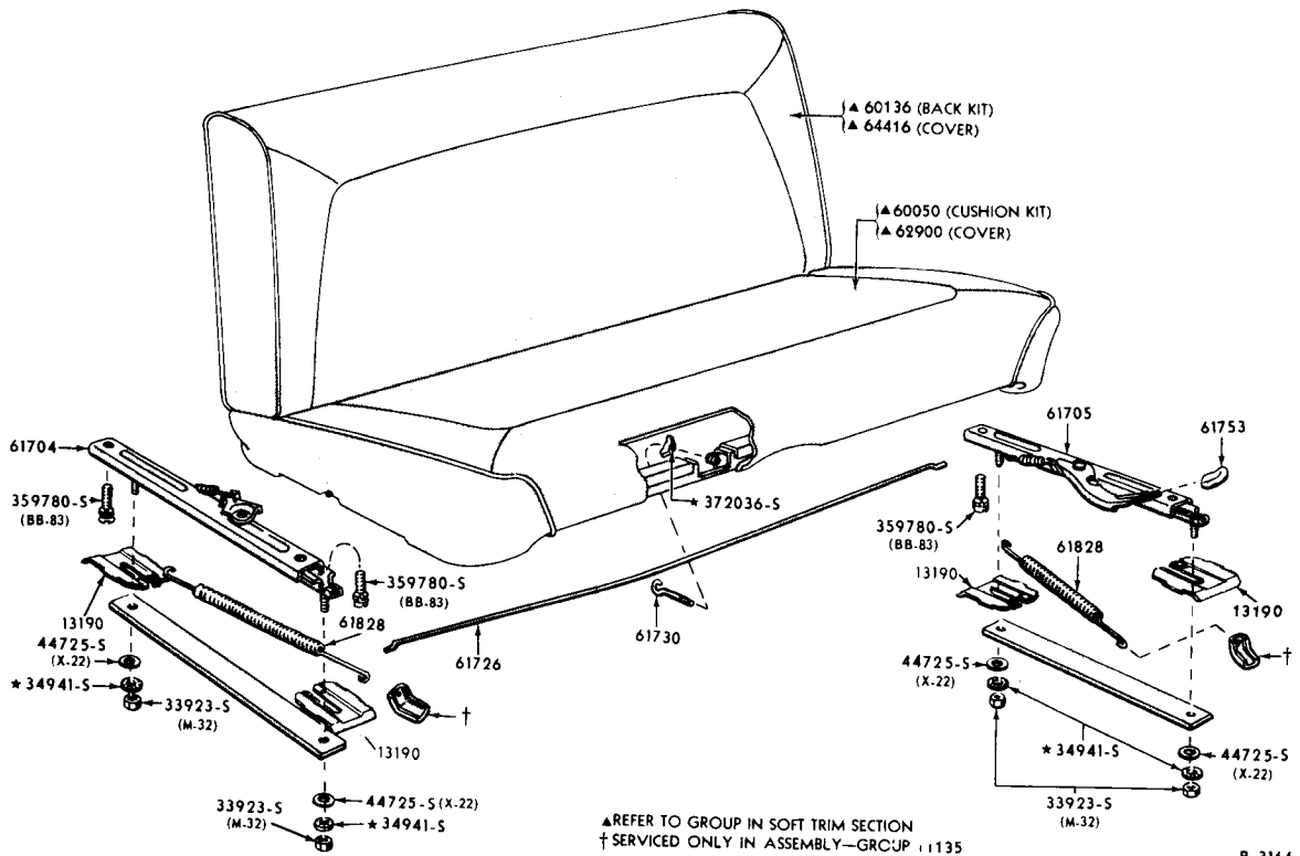
FRONT SEAT MECHANISM and RELATED PARTS - MANUAL FULL WIDTH 1965/67 FALCON
