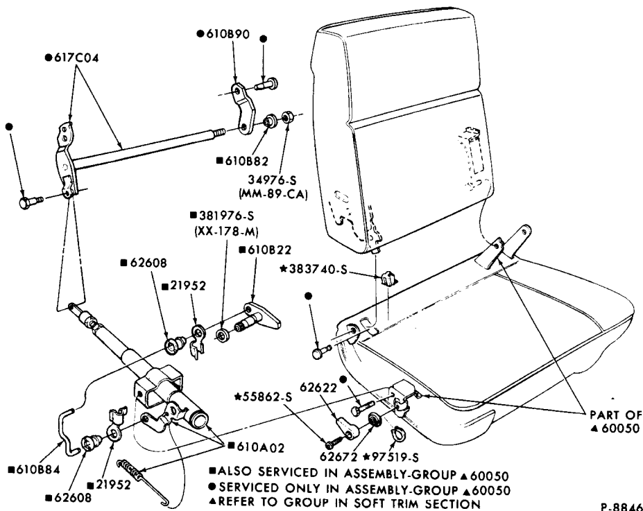
RECLINING SEAT MECHANISM and RELATED PARTS 1971/72 FORD
