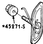
*45271-S •C9OZ-16A076-A EJ
