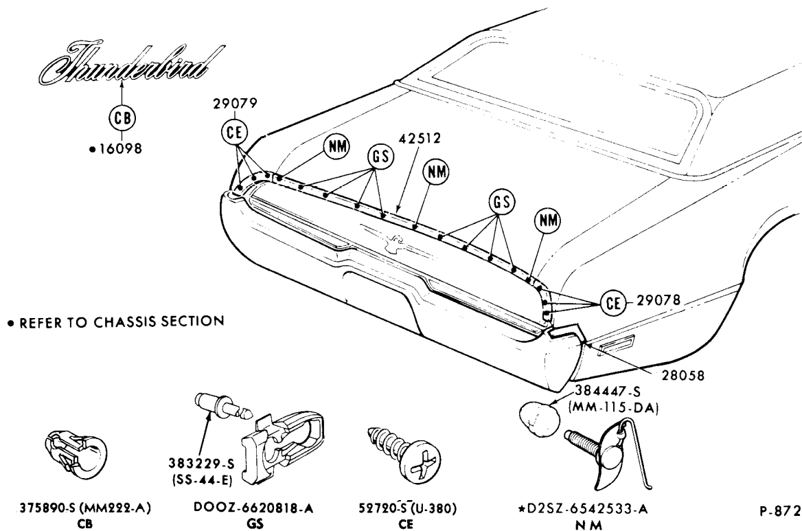
1972 THUNDERBIRD - BACK END
