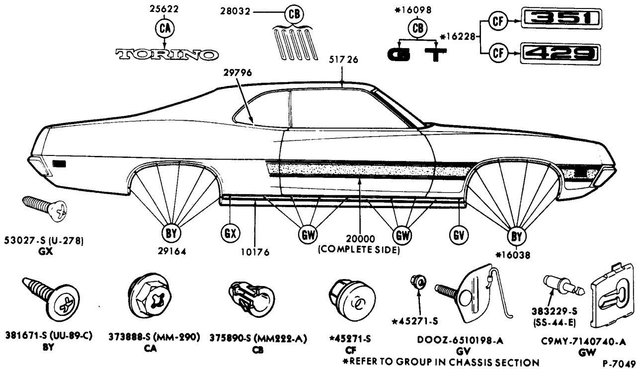
1970 FAIRLANE/TORINO - BODY TYPE 63F,65F,66C,76F - SIDE
