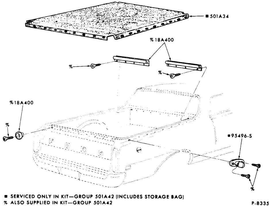
TONNEAU COVER and RELATED PARTS 1971/72 TORINO - BODY TYPES 66, 97
