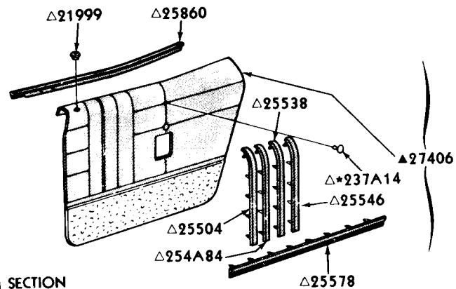
REAR DOOR
