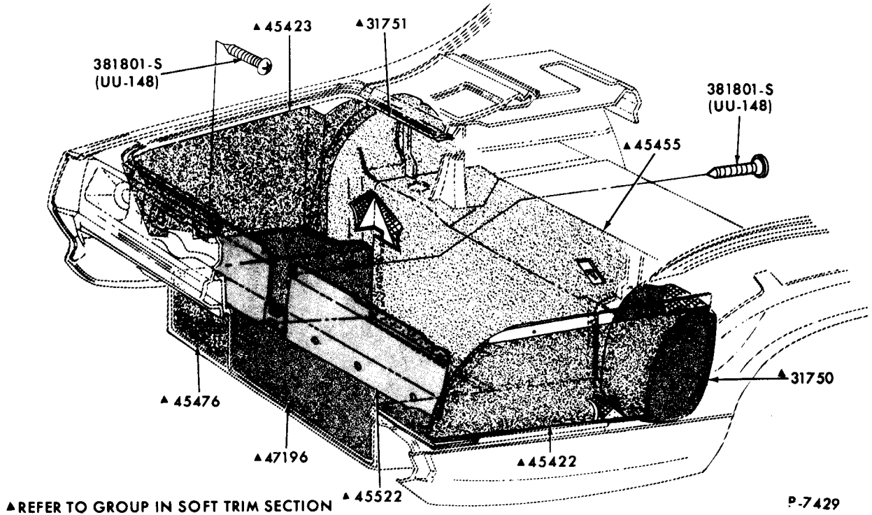
LUGGAGE COMPARTMENT TRIM 1970/71 THUNDERBIRD
