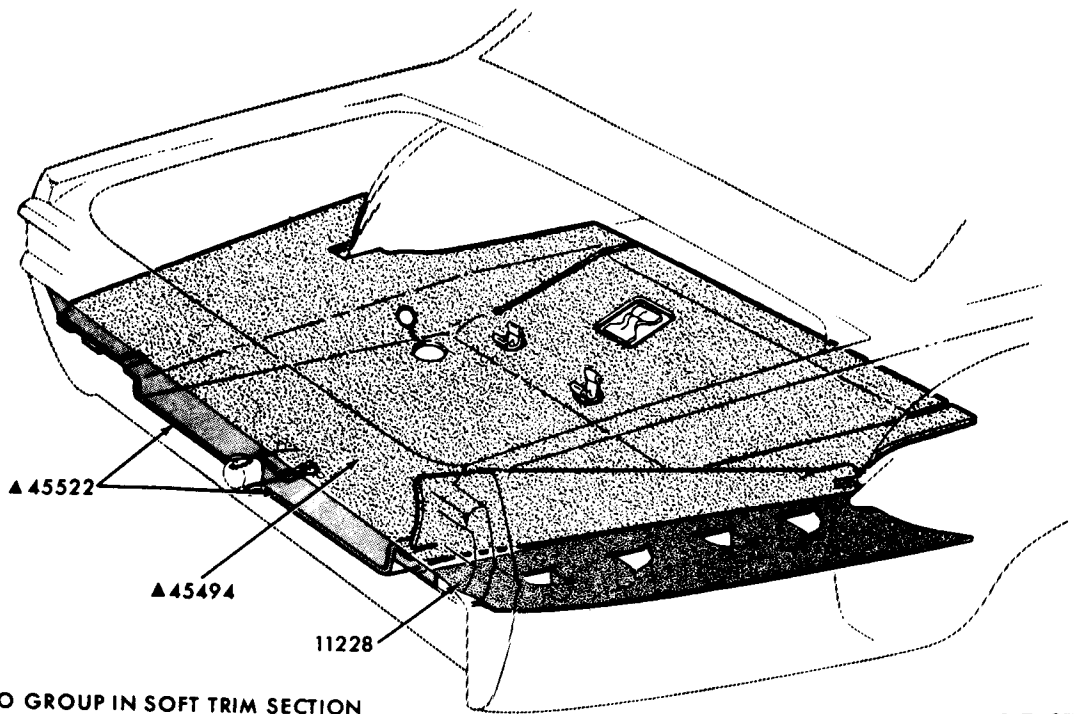
LUGGAGE COMPARTMENT TRIM 1970/71 FAIRLANE/TORINO - BODY TYPES 54, 57, 62, 63, 65 and 76
