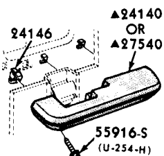
FRONT OR REAR DOOR
