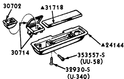
QUARTER
