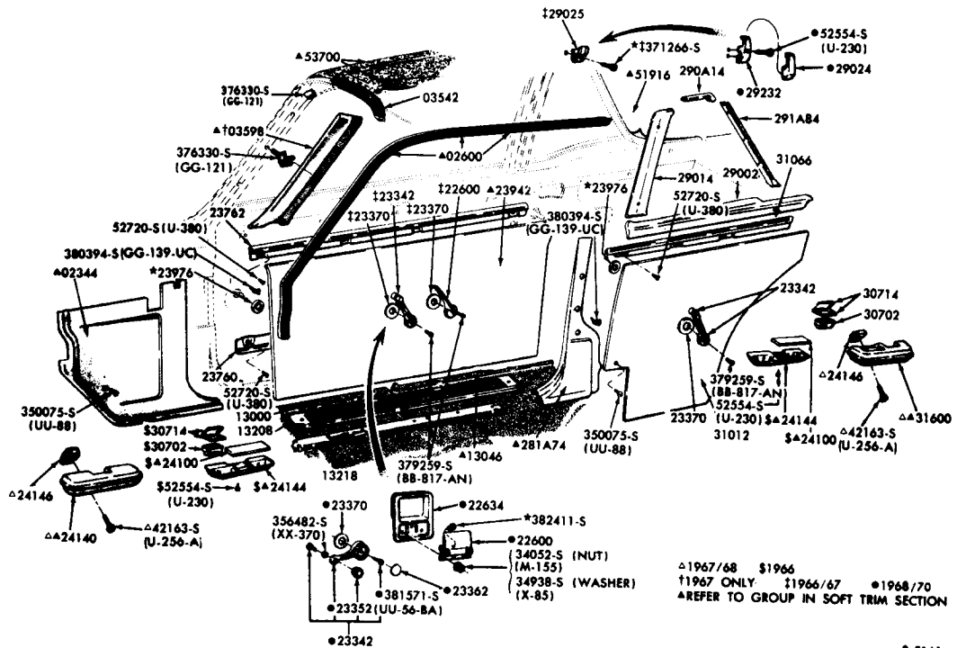
INTERIOR TRIM and RELATED PARTS
