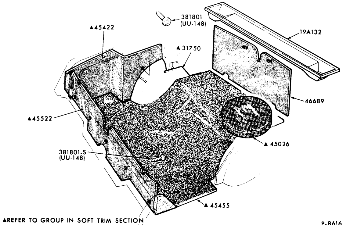
LUGGAGE COMPARTMENT TRIM 1972 THUNDERBIRD
