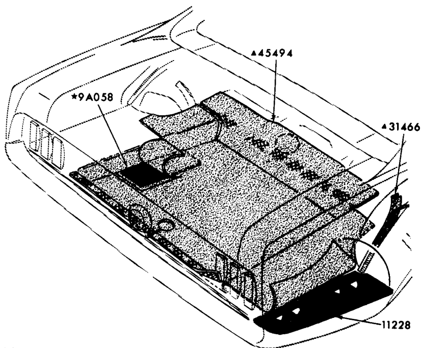
LUGGAGE COMPARTMENT TRIM 1969/72 MUSTANG
