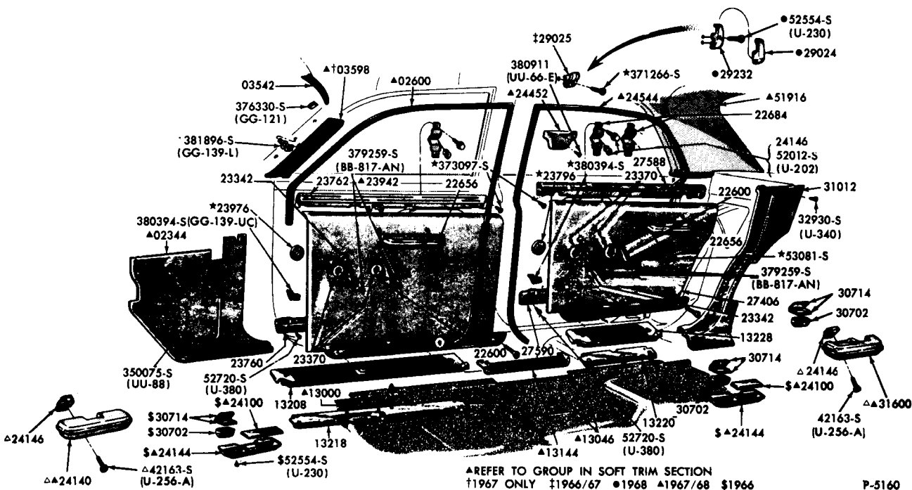
INTERIOR TRIM and RELATED PARTS 1966/67 FALCON - BODY TYPE 54
