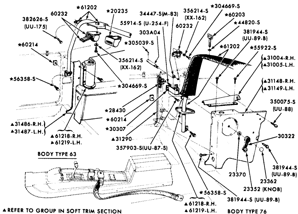
ROLL BAR AND RELATED PARTS 1969/70 MUSTANG-SHELBY GT350/500
