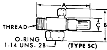
BLOCK COMPRESSOR FITTING
