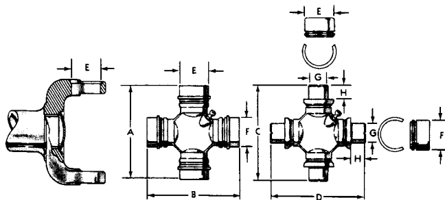
MECHANICS, CLEVELAND STEEL OR SACO DESIGN
