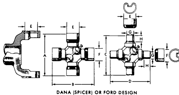
DANA (SPICER) OR FORD DESIGN
