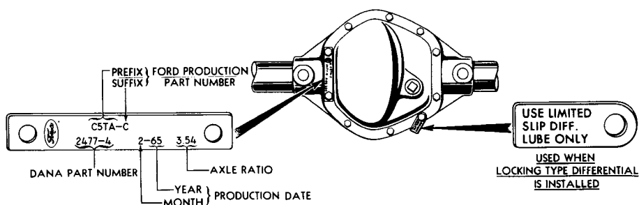
DANA AXLE IDENTIFICATION
