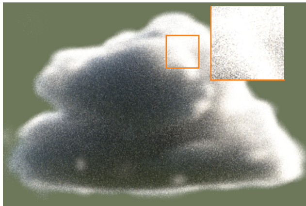
RIS K=6 (64 spp) RMSE 0.160, 7.7 s
