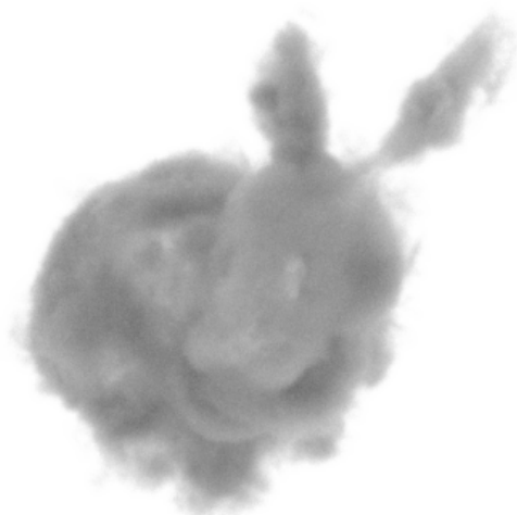
bunny — ours
