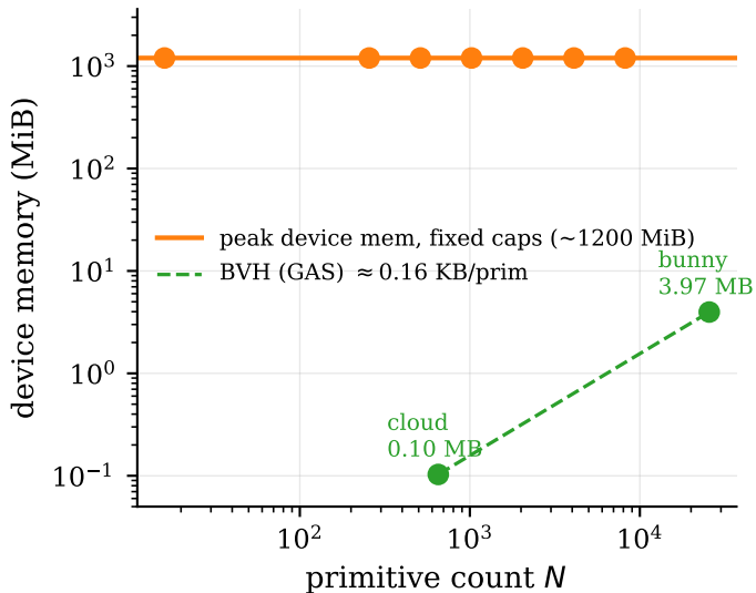
Memory is decoupled from N
