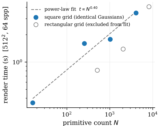
Time vs primitive count
