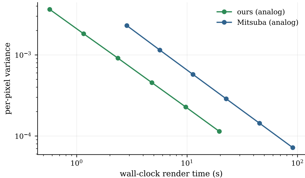
variance vs time (equal-variance = horizontal gap)
