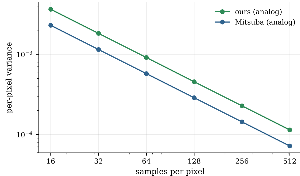
Sampler only (flat env): variance vs samples
