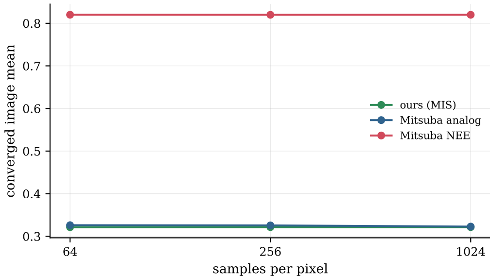
Cloud-meadow: NEE vs analog do not converge to a common mean
