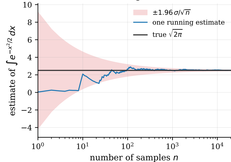
Estimate converges to the value
