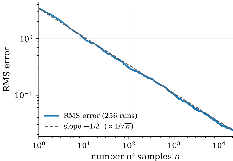
Error falls as 1/\sqrt{n}
