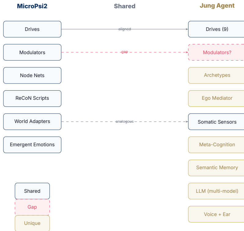
Figure 2: Architectural comparison: shared components (drives), gaps (modulators), and unique capabilities (archetypes, LLM, voice). Dashed red = missing in Jung Agent. Gold = unique to Jung Agent.
