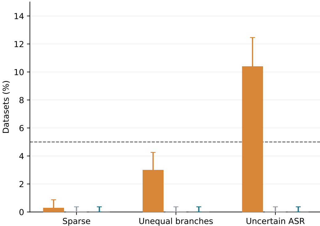
Known CTMC parameters · 1,000 datasets per condition · 95% exact intervals Null: any false discovery Injected sites: at least one detected
