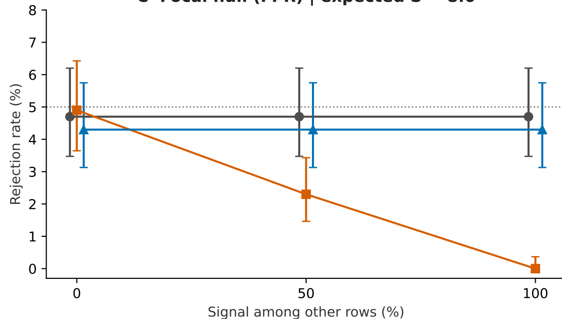
C Focal null (FPR) | expected S = 8.0
