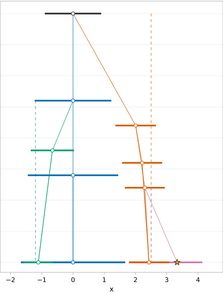
x | Prior
