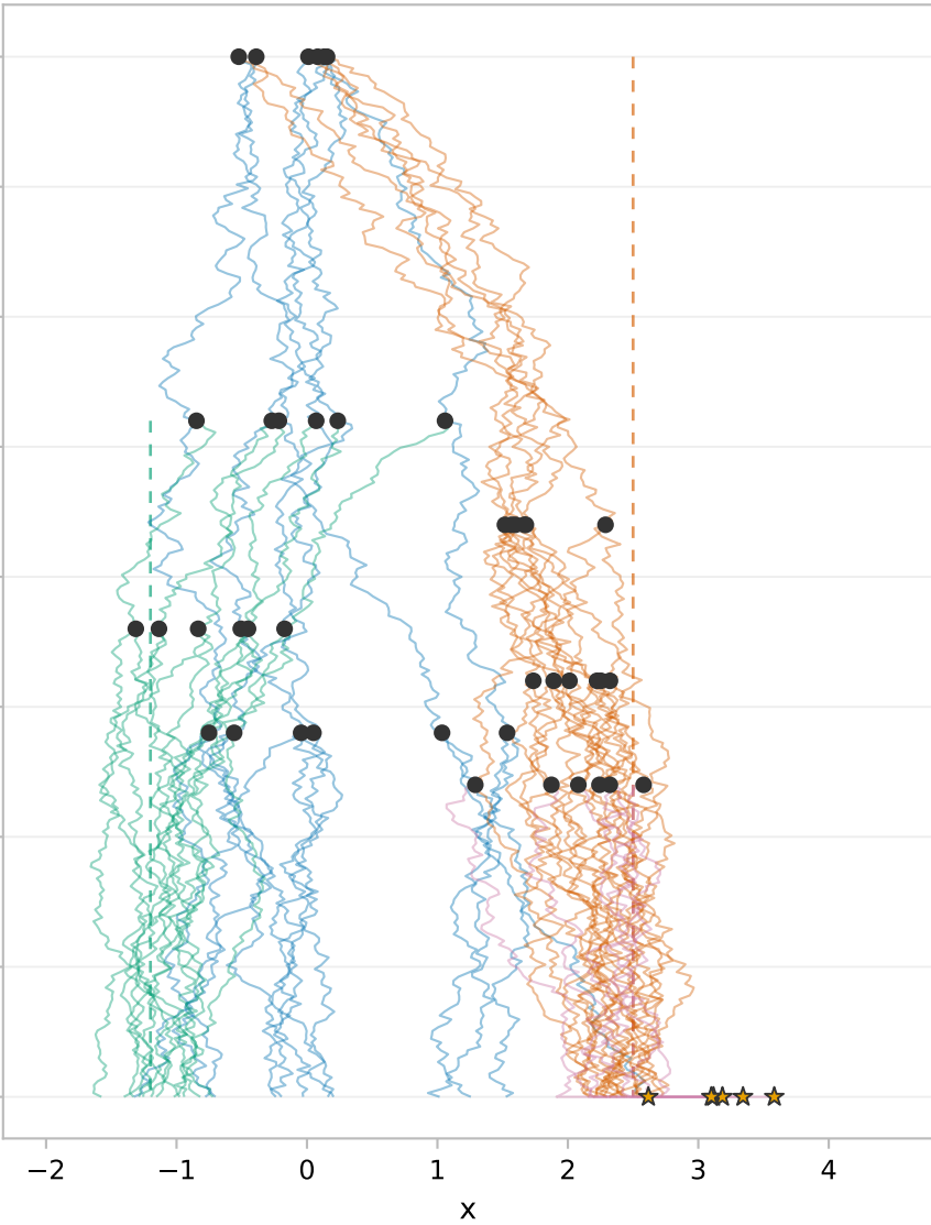
x | simulation
